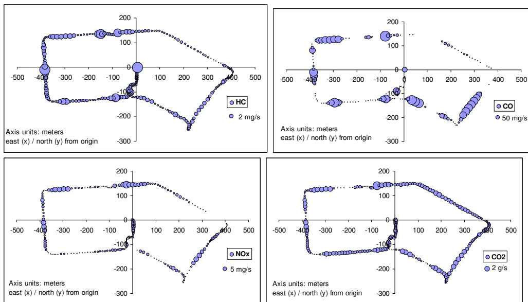
Figure 9. Top view of the on-road trip geometry with size-coded instantaneous mass emissions rates of HC, CO, NO x and CO 2 averaged on three runs of Vehicle 2. See details in Figure 3).
