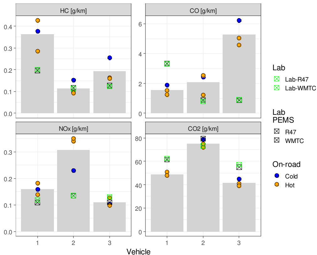
Figure 10. Summary of real driving and laboratory emissions. Roller bench data points were obtained with laboratory instrumentation (green) and the Mini-PEMS (black). Grey bars are average real driving emission factors obtained from single on-road cold start (blue) and hot start tests (orange).
