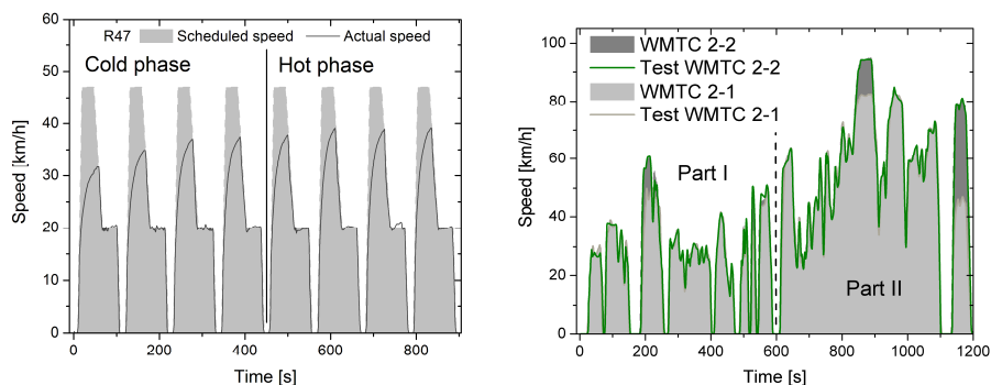
Figure 2. Legislative speed profiles (grey shaded area) and examples of actual test speed for driving cycles ECE-R47 (left panel), WMTC type 2-1 and WMTC 2-2 (right panel) run by vehicles 1, 3 and 2, respectively; see text for details.
