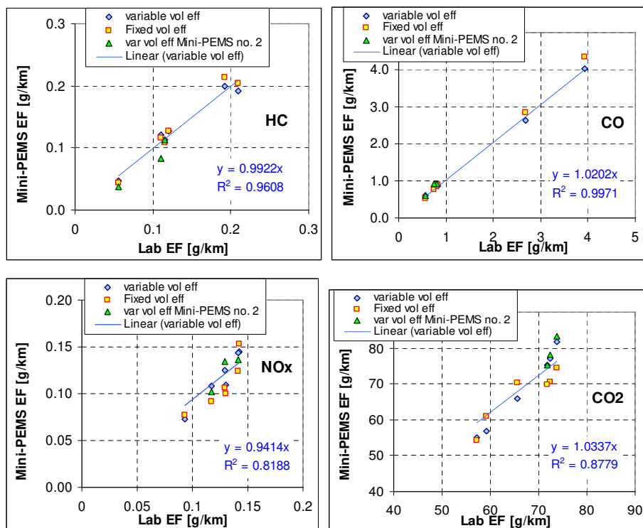
Figure 7. Emission factors of HC, NOx, CO and CO 2 from bench instrumentation (horizontal axis), and from Mini-PEMS No. 1 (vertical axis) obtained during roller bench tests.
