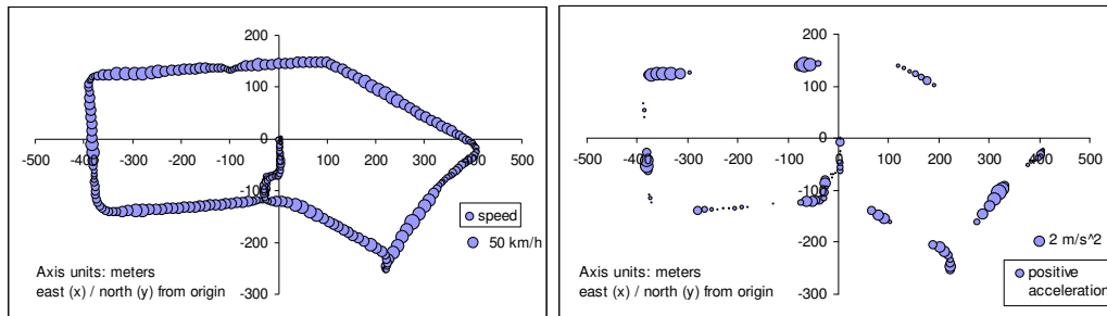
Figure 3. Top view of on-road trips geometry ([m]) with size-coded speed (left panel) and positive acceleration (right panel) for Vehicle 2. The vehicles had to pass 3 stop road-signals and 2 roundabouts.
