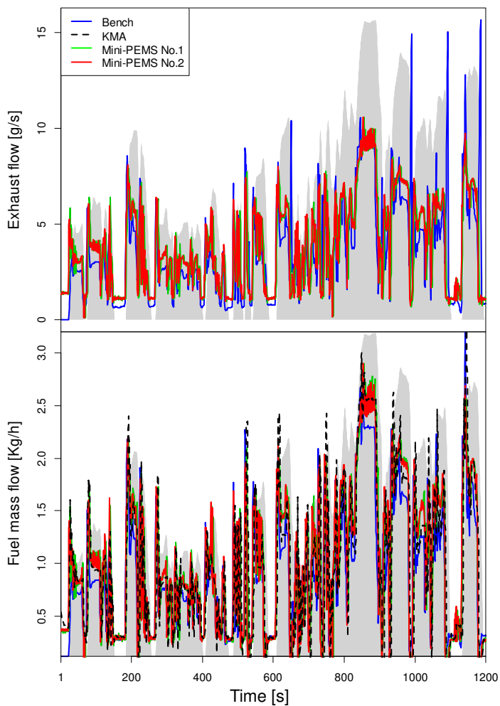
Figure 5. Upper panel: Comparison of the exhaust flow from bench instrumentation calculated with the CO 2 tracer method and from the 2 Mini-PEMS during Test 5. Lower panel: Comparison of fuel consumption (i) measured by a dedicated fuel flowmeter (KMA); (ii) calculated with the carbon balance method using HC, CO and CO 2 mass emissions rates from bench instrumentation; and (iii) calculated from Mini-PEMS No. 1 and No. 2.
