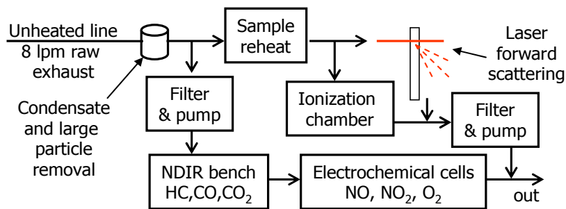
Figure 4. Schematic of the miniature portable on-board emissions monitoring system (Mini-PEMS); see text for details.
