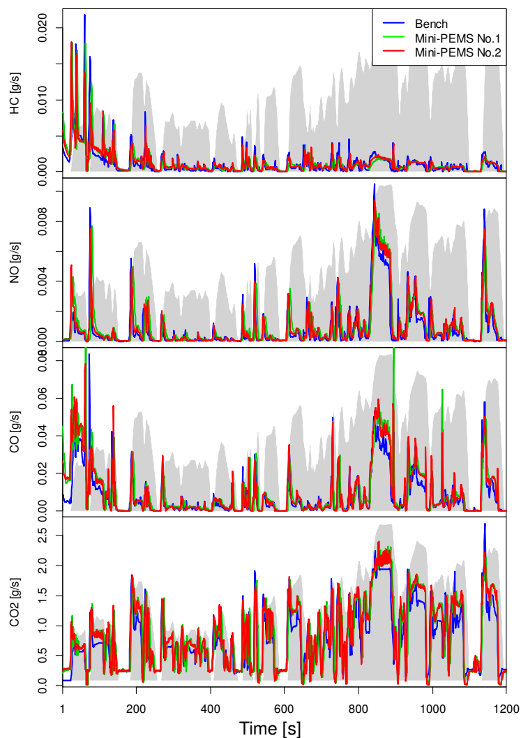
Figure 6. Mass flow rates of HC, NO x , CO and CO 2 from bench instrumentation and from the two Mini-PEMS for Vehicle 2 during Test 5 (WMTC).
