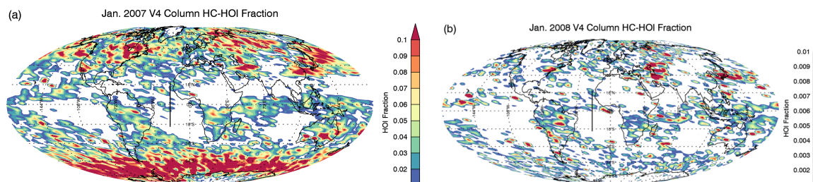
Figure 7: Comparison of the high-confidence HOI column fraction of cloudy bins observed at 0.3° and 3° by CALIOP during January 2007 and 2008, Panels (a) and (b), respectively. The column HOI fraction is calculated as the ratio of high-confidence HOI identified by the phase algorithm to the total number of cloudy bins observed by CALIOP at 5-80 km resolution, compiled at 2° latitude x 5° longitude, daytime and nighttime together. The scale in Panel (b) is 1/10 of that in Panel (a).
