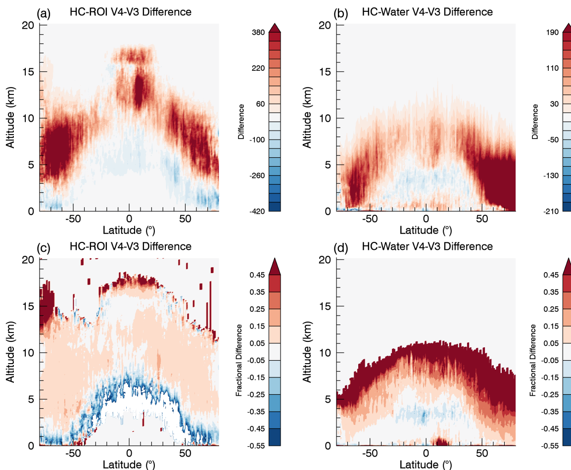
Figure 15: V4-V3 Difference plots for high-confidence ROI (HC-ROI, left-hand column) and high-confidence water (HC water, right-hand column) cloudy bins observed during October 2010. Panels (a) and (b) show the V4-V3 difference in accumulated cloudy bins for ROI and water and Panels (c) and (d) show the fractional V4-V3 difference when normalized to V4.
