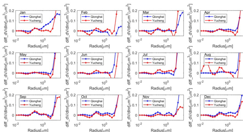
Figure : The difference between retrieved monthly volume size distribution by V4.2 and by V5.0 ( d(V_{V4.2} - V_{V5.0})/d\ln r ) for Qionghai (blued lines) and Yucheng (red lines) during February 2013 to December 2015
