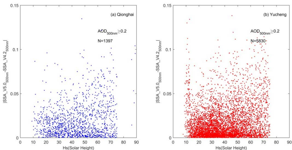
Figure: Scattergrams of the SSA differences at 500nm between V5.0 and V4.2 (defined as: |SSA_{V5.0, 500nm} - SSA_{V4.2, 500nm}| ) and the corresponding solar height over Qionghai (a) and Yucheng (b).
