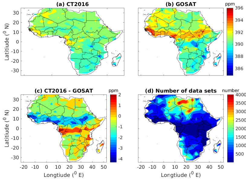
Figure 1. Distribution of five-years averages of CT2016 (a) and GOSAT (b) XCO_2 and their difference (c) gridded in 3^\circ \times 2^\circ bins over Africa's Land mass; and the total number of datasets at each grid from the GOSAT observations(d).
