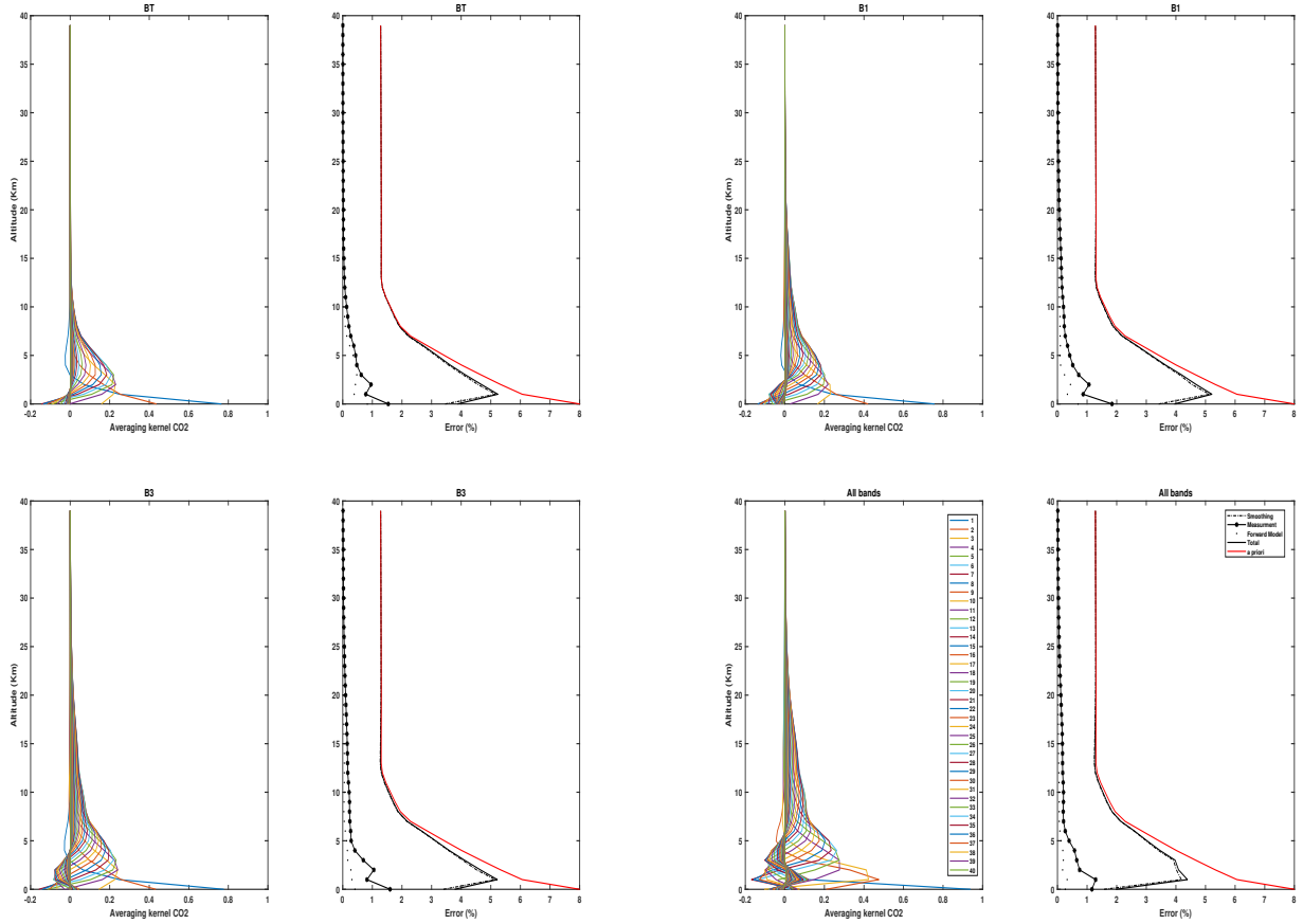
Fig. 8: Averaging kernels and error budgets of CO_2 vertical profiles for bands BT, B1 and B3 separately and all the bands together for an angle of 10^\circ for CHRIS. The red and solid black lines stand for the prior ( S_a ) and posterior ( S_x ) errors respectively; the smoothing ( S_{smoothing} ), measurement ( S_{meas.} ), and forward model parameters ( S_{fwd.mod.} ) errors are dashed/dotted, dashed/starred and dotted, respectively.
