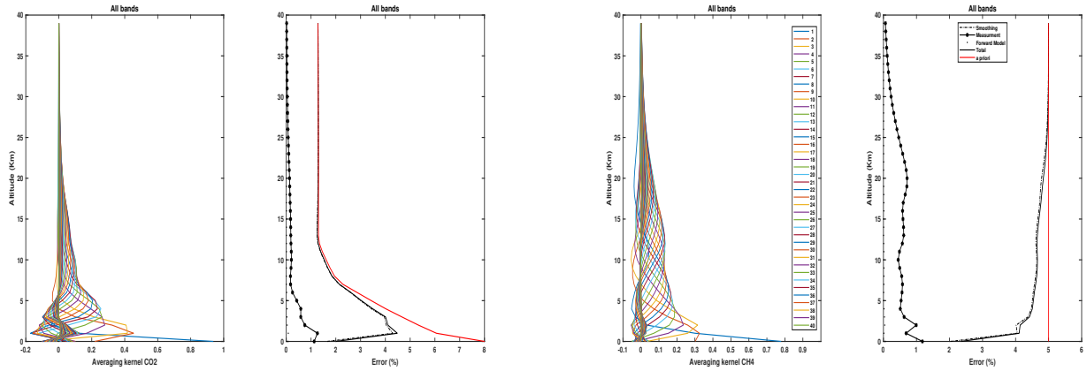
Fig. 10: Averaging kernels and error budgets of CO_2 and CH_4 vertical profiles for all the bands together for EM27/SUN and CHRIS combined for an angle of 10^\circ . The red and black lines stand for the prior ( S_a ) and posterior ( S_x ) errors respectively; the smoothing ( S_{smoothing} ), measurement ( S_{meas.} ), and forward model parameters ( S_{fd.mod.} ) errors are dashed/dotted, dashed/starred and dotted, respectively.
