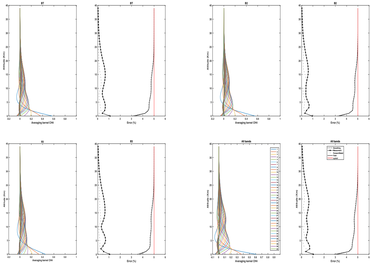
Fig. 9: Same as Fig. 8, but for CH_4 with bands BT, B2, B3 and all the bands together.
