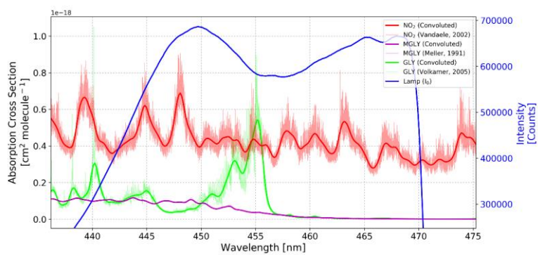
5 Figure 2. Reference spectrum of the IBBCEAS system (blue) and absorption cross sections of NO 2 , GLY, and MGLY. The thin lines are the high resolution cross sections documented in the literature and the thick lines are the cross sections after processing with the instrument function determined by the Fraunhofer reference spectrum (Kurucz et al., 1984).
