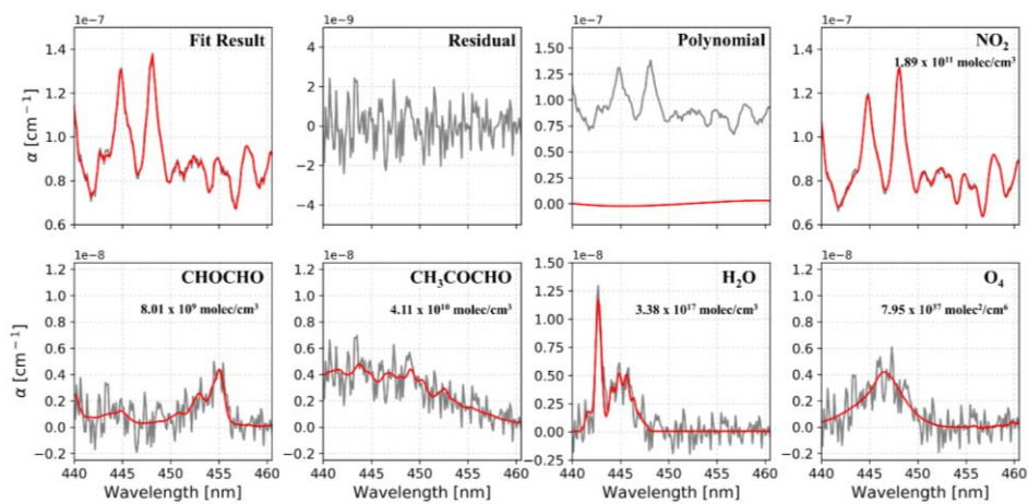
Figure 6. An example of spectral fit for one spectrum (60s average) measured during the YRD campaign. Retrievals of NO 2 , CHOCHO, CH 3 COCHO, H 2 O, and O 4 are shown, as well as the fifth-order polynomial, total fit, and residual. Red is the fitted spectrum and black is the fitted result plus residual.
