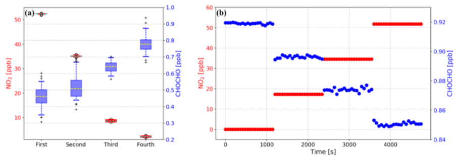
5 Figure 9. (a) Keep the concentration of GLY constant and mix it evenly with different concentrations of NO 2 for four times. The concentration of GLY measured by IBCEAS increased as that of NO 2 decreased, although only the NO 2 concentration was reduced manually. (b) Simulate a series of spectra with constant GLY concentration and increasing NO 2 concentration and then calculate concentrations of GLY and NO 2 by retrieving these simulated spectra. The retrieved GLY concentration decreased with the increasing NO 2 concentration, although the set value of GLY concentration in the simulation was kept constant.
