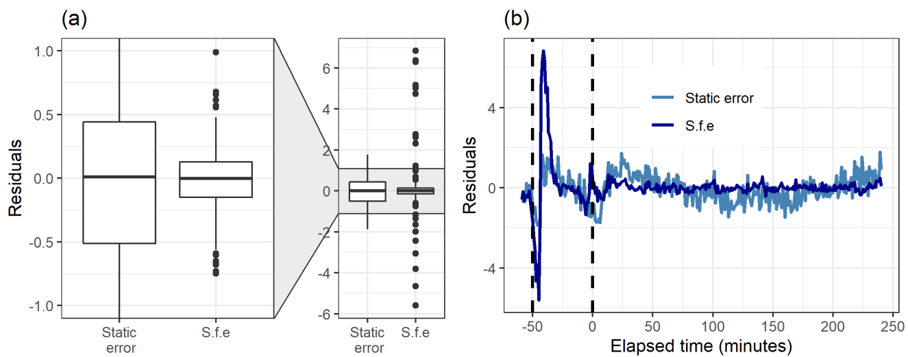
Figure 8: Boxplot (a) and the time series (b) of the residuals (original total signal – reconstructed total signal) with static error and signal following error (S.f.e) with 5 factors from PMF for the measured gas phase (PTR-MS) data.
