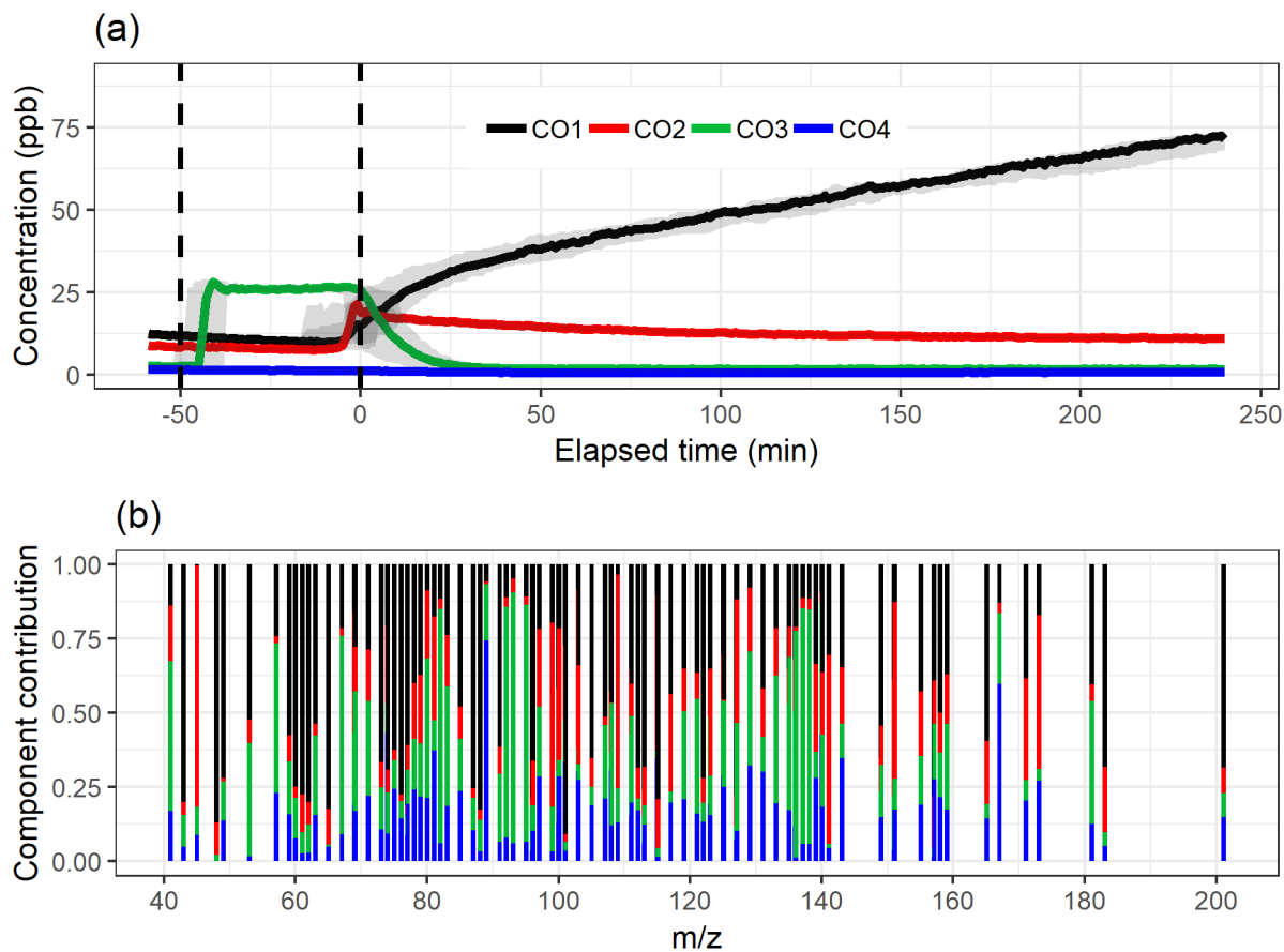
Figure 4: The component time series (a) and contribution (b) for EVD-PCA with Oblimin rotation for the 4-component solution. Shaded areas in the time series indicate the component range for the bootstrap resamples, solid lines are for the measured gas phase (PTR-MS) data. The colour code identifying components is the same in both panels. Components were identified as later/slowly forming products (CO1), early products (CO2), \alpha -pinene precursor (CO3) and background/car exhaust precursor (CO4).
