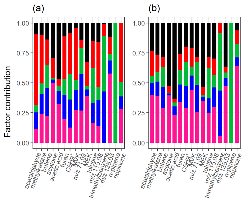
5 Figure 10: Total factor contribution of selected compounds from a) NMF and b) PMF with static error for the measured gas phase (PTR-MS) data. Colour code identifying the factors is the same in both panels and were identified as later/slowly forming products (black), early products red), α-pinene precursor (green), background/car exhaust precursor (blue) and intermediate products (pink).
