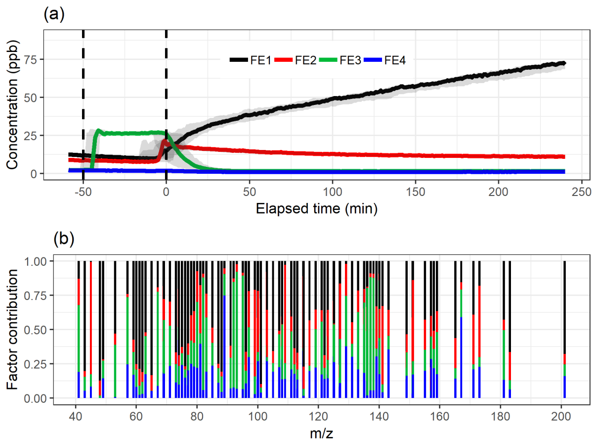
Figure 3: The factor time series (a) and contribution (b) for ml-EFA with Oblimin rotation for the 4-factor solution. Shaded areas in the time series indicate the factor range for the bootstrap resamples, solid lines are for the measured gas phase (PTR-MS) data. The colour code identifying factors is the same in both panels. Factors were identified as later/slowly forming products (FE1), early products (FE2), \alpha -pinene precursor (FE3) and background/car exhaust precursor (FE4).
