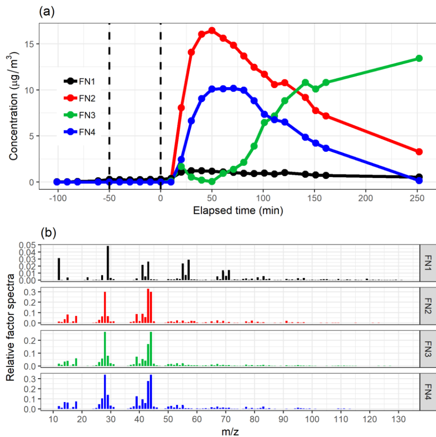
Figure 12: The factor time series (a) and relative factor spectra (b) from NMF with 4 factors for the measured particle phase (AMS) data. The colour code identifying the factors is the same in both panels. Factors were identified as primary OA (FN1), \alpha P-SOA-SVOOA (FN2), mixed LVOOA (FN3) and \alpha P-SOA-LVOOA (FN4).
