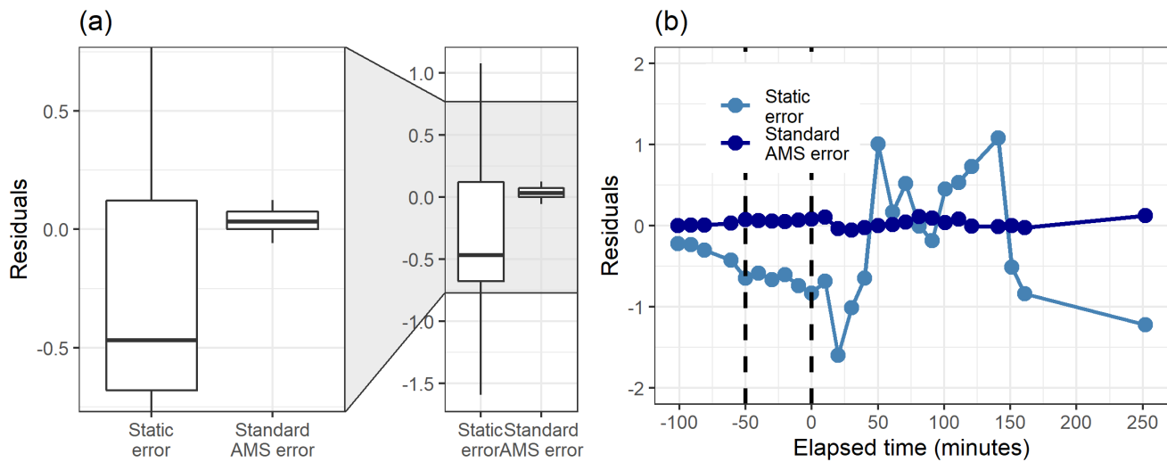
Figure 14: Boxplot (a) and the time series (b) of the residuals (original total signal – reconstructed total signal) with static error and standard AMS error with 2 factors from PMF for the measured particle phase (AMS) data.
