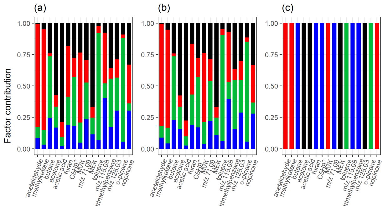
Figure 9: Total factor/component/cluster contribution of selected compounds from a) ml-EFA, b) EVD-PCA and c) PAM for the measured gas phase (PTR-MS) data. Colour code identifying the factors/components/clusters is the same in all panels and were identified as later/slowly forming products (black), early products red), \alpha -pinene precursor (green) and background/car exhaust precursor (blue).
