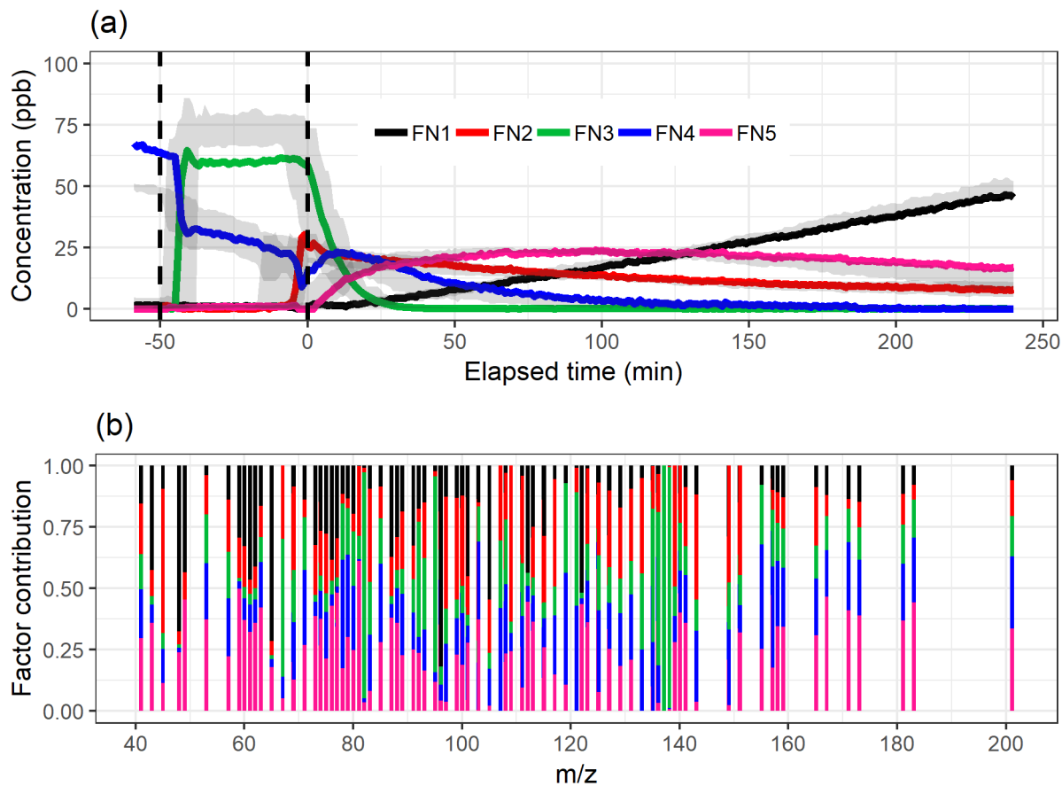
Figure 6: The time series (a) of the factors and the distribution of ion to factor (b) from NMF with 5-factor solution. Shaded areas in the time series indicates the factor range for the bootstrap resamples, solid lines are for the measured gas phase (PTR-MS) data. The colour code identifying clusters is the same in both panels. Factors were identified as later/slowly forming products (FN1), early products (FN2), \alpha -pinene precursor (FN3), background/car exhaust precursor (FN4) and intermediate products (FN5).
