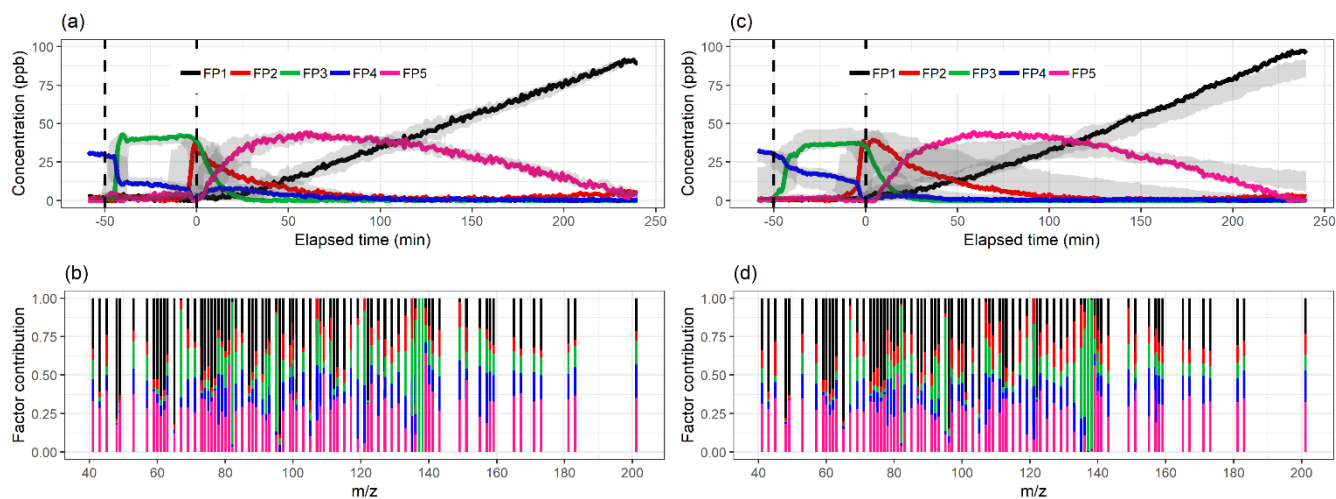
Figure 7: Factor time series and contribution from PMF with static error (a-b) and signal following error (c-d) for factorization rank 5. Shaded areas in the time series indicates the factor range for the bootstrap resamples, solid lines are for the measured gas phase (PTR-MS) data. The colour code identifying the factors is the same in the top and bottom panels. Factors were identified as later/slowly forming products (FP1), early products (FP2), \alpha -pinene precursor (FP3), background/car exhaust precursor (FP4) and intermediate products (FP5).
