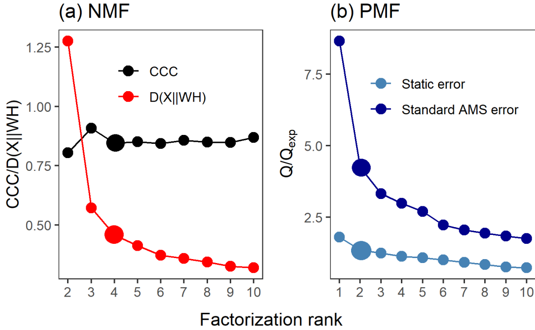
5 Figure 11: Factor number indexes for particle phase data (AMS). Estimation of the factorization rank for NMF in (a) with CCC and D(X||WH) and for PMF in (b) with Q/Q_{exp} for the two error schemes. Larger points indicate the solution that was selected for more detailed interpretation.
