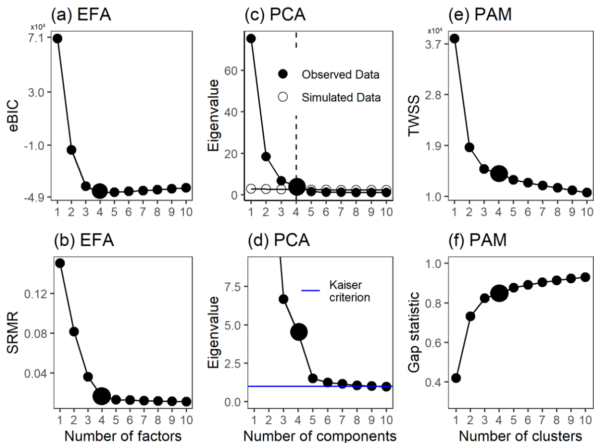
5 Figure 1: Factor number indexes for gas phase data (PTR-MS). Empirical BIC (a) and SRMR (b) as a function of the number of factors for ml-EFA, Parallel analysis (c) and Kaiser criterion (d) for EVD-PCA and TWSS (e) and Gap statistic (f) for PAM. Larger points indicate the solution that was selected for more detailed interpretation.
