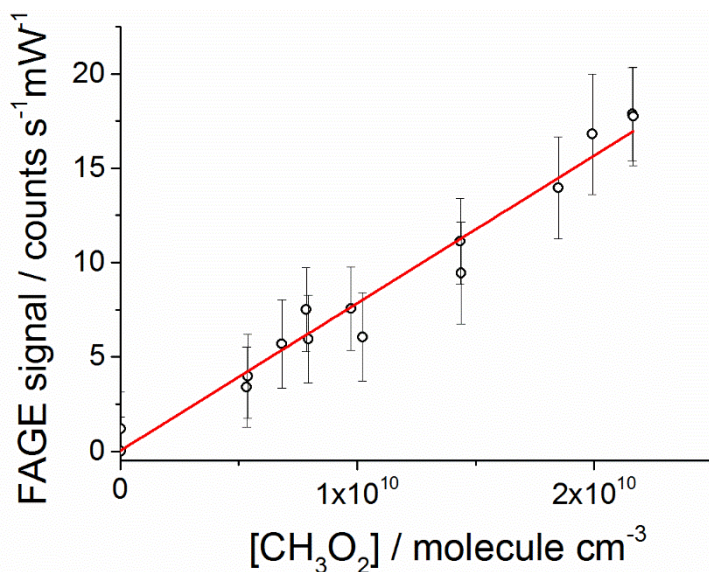
Figure S1. An example of a calibration using the indirect FAGE technique for \text{CH}_3\text{O}_2 detection using 184.9 nm photolysis of water vapour at 295 K and atmospheric pressure to generate OH radicals. \text{CH}_3\text{O}_2 radicals were generated using the reaction OH with \text{CH}_4 in the presence of \text{O}_2 , in the range of \sim (0.5\text{--}2.0) \times 10^{10} molecule \text{cm}^{-3} by varying the power supplied to the photolysis lamp; [\text{CH}_4] = 5.0 \times 10^{16} molecule \text{cm}^{-3} and [\text{NO}] = 6.7 \times 10^{13} molecule \text{cm}^{-3} . A line of best fit through these data yields a sensitivity factor C_{\text{CH}_3\text{O}_2} = (7.8 \pm 0.4) \times 10^{-10} counts \text{cm}^3 molecules ^{-1} s ^{-1} mW ^{-1} , where the error limits are the standard error of the fit to the data. The error limits in the FAGE signal are statistical errors at the 1\sigma level.
