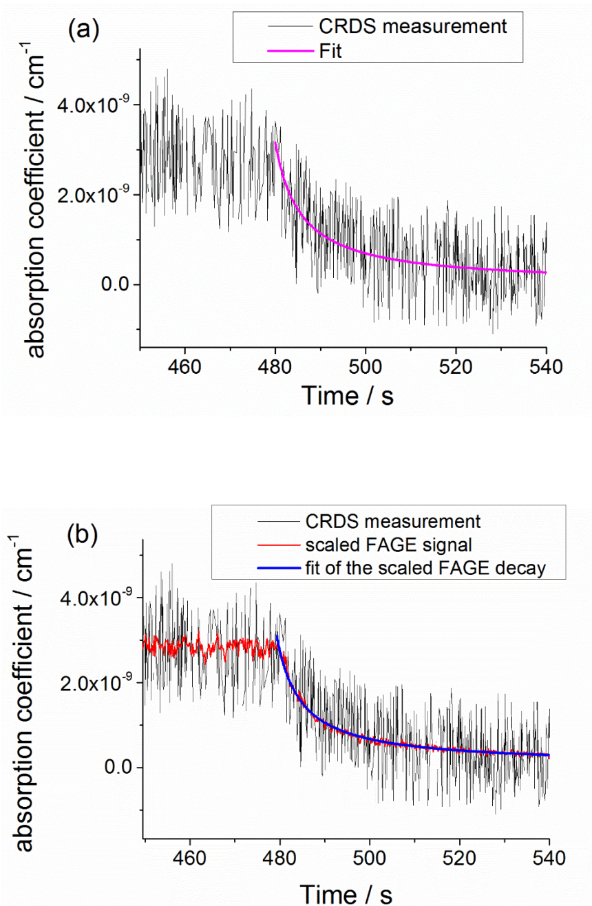
Figure S5. Second-order decay of the \text{CH}_3\text{O}_2 absorption coefficient at 7488 \text{ cm}^{-1} from CRDS data (single ring-down events – black line in both panels (a) and (b)) along with the FAGE signal monitored simultaneously but scaled vertically to overlap the CRDS data (red line; panel (b)). The traces were recorded at 295 K and with a 80 mbar mixture of \text{He}:\text{O}_2 = 3:1 ; [\text{Cl}_2]_0 = 1.1 \times 10^{14} \text{ molecule cm}^{-3} and [\text{CH}_4]_0 = 2.5 \times 10^{16} \text{ molecule cm}^{-3} . The fit of Eq. (8) in the main text to the CRDS data (magenta line in panel (a)) resulted in \sigma_{\text{HO}_2} = (1.71 \pm 0.15) \times 10^{-20} \text{ cm}^2 \text{ molecule}^{-1} while the fit of the same equation to the scaled FAGE data (blue line; panel (b)) gave \sigma_{\text{HO}_2} = (1.55 \pm 0.02) \times 10^{-20} \text{ cm}^2 \text{ molecule}^{-1} . The error limits are statistical errors at the 1\sigma level.
