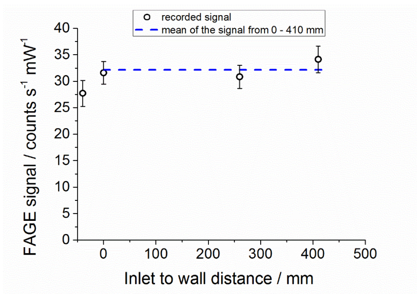
Figure S4. Measurement of the \text{CH}_3\text{O}_2 radical signal plotted against the distance the FAGE inlet protrudes from the HIRAC chamber. Each point (black circles) shows the steady-state \text{CH}_3\text{O}_2 signal averaged over 5 min for a certain position of the instrument inlet across the chamber radius. The blue line represents the mean of the signal recorded from 0 mm (inlet flush with the wall) to 410 mm inlet to internal wall distance. \text{CH}_3\text{O}_2 was generated by photolysing ozone ( \sim 2.5 \times 10^{13} molecule \text{cm}^{-3} ) in the presence of methane ( 2.5 \times 10^{17} molecule \text{cm}^{-3} ) at 254 nm. The FAGE instrument couples to the chamber through a flange mounted on the outside, allowing the inlet to be positioned behind the chamber walls similar to the CRDS mirrors. Here (40 mm behind the wall, so -40 mm), a 14% signal drop was observed compared to the mean of values from 0 – 410 mm.
