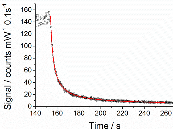
Figure S2. \text{CH}_3\text{O}_2 decay via its self-reaction measured by FAGE for the 80 mbar He: \text{O}_2 (3:1) atmosphere within HIRAC. Radicals were generated by photolysis of molecular chlorine in the presence of methane, with [\text{Cl}_2] = 3.2 \times 10^{14} molecule \text{cm}^{-3} and [\text{CH}_4] = 2.5 \times 10^{17} molecule \text{cm}^{-3} . The photolysis lamps were turned off at \sim 150 s. Fitting Eq. (5) in the main text to the data yields the sensitivity factor C_{\text{CH}_3\text{O}_2} = (3.89 \pm 0.05) \times 10^{-9} counts \text{cm}^3 molecules ^{-1} s ^{-1} mW ^{-1} . The error limits are statistical errors at the 1\sigma level.
