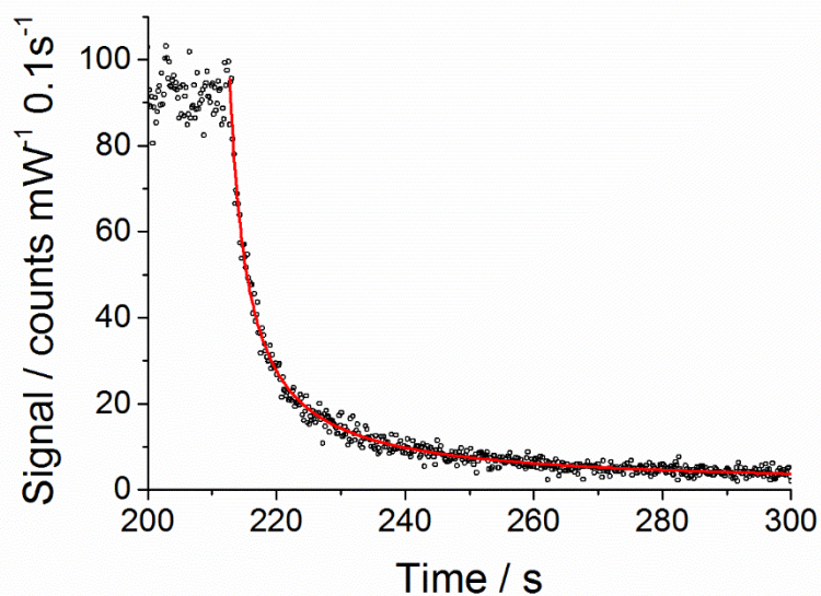
Figure S3. \text{CH}_3\text{O}_2 decay via its self-reaction measured by FAGE for the 100 mbar synthetic air atmosphere within HIRAC. Radicals were generated by photolysis of molecular chlorine in the presence of methane, with [\text{Cl}_2] = 3.3 \times 10^{14} \text{ molecule cm}^{-3} and [\text{CH}_4] = 2.5 \times 10^{17} \text{ molecule cm}^{-3} . The photolysis lamps were turned off at \sim 210 \text{ s} . Fitting Eq. (5) in the main text to the data yields the sensitivity factor C_{\text{CH}_3\text{O}_2} = (2.65 \pm 0.04) \times 10^{-9} \text{ counts cm}^3 \text{ molecules}^{-1} \text{ s}^{-1} \text{ mW}^{-1} . The error limits are statistical errors at the 1\sigma level.
