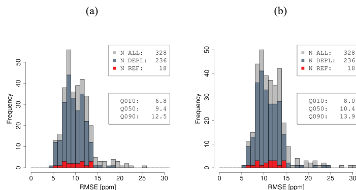
Figure 8: RMSE values of sensor calibration (a) using Eq. (4) and (b) using Eq. (5). Three histograms are overlaid: all calibrated sensors, sensors deployed in the Carbosense network (DEPL) and sensors at locations with a reference instrument (REF). The indicated quantiles refer to the set of deployed sensors.
