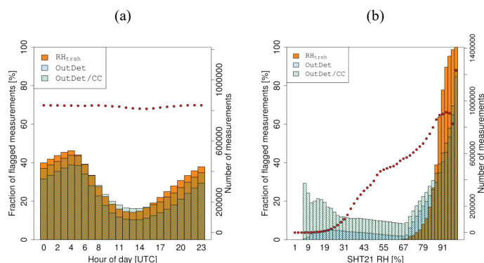
10 Figure 14: Analysis of the results of measurement filtering referring to time of day (a) and relative humidity (b). Filtering is based on (i) a sensor specific \text{RH}_{\text{trsh}} value, (ii) the outlier detection algorithm (OutDet), and (iii) the outlier detection algorithm plus a consistency check (OutDet/CC). For the calculation of the fraction of flagged measurements, the number of measurements and flags of all deployments are summed. The numbers of measurements are depicted as red dots.
