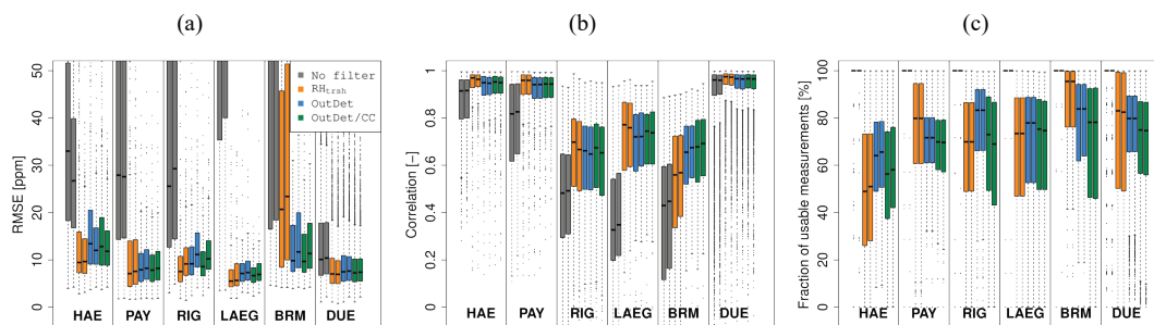
Figure 10: (a) Weekly RMSE values for all the sensors deployed at HAE, PAY, RIG, BRM/LAEG and DUE. For each site four versions are presented for the drift adjusted measurements: (i) no filtering applied, (ii) outlier detection based on sensor specific RH_{trsb} value, (iii) outlier detection algorithm, and (iv) outlier detection algorithm plus consistency check. The left bar with the same colour refers to Eq. (4), the right bar to Eq. (5). (b) Same as in (a) for the weekly correlation. (c) Same as in (a) for the weekly fraction of used data. Here, the fraction refers to the number of measurements transmitted to the database.
