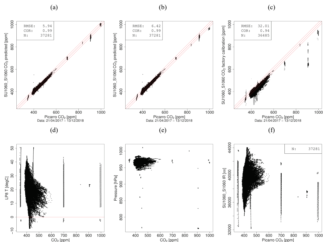
Figure 7: (a) Calibrated sensor measurements (Eq. 4) versus measurements from Picarro instruments exemplarily shown for sensor 1060. The data set contains measurements from the climate and pressure chambers and ambient measurements. The band between the red dashed lines denotes a range of \pm 20 ppm. (b) Same as in (a) but for Eq. (5). (c) Same as in (a) but for factory calibrated sensor measurements. Measurements outside the sensor specifications are depicted in gray and included for RMSE/correlation. (d) \text{CO}_2 – LP8 T plot and (e) \text{CO}_2 – P plot depicting the environmental conditions covered during calibration. Same data set as in (a). (f) LP8 IR measurements versus \text{CO}_2 from the Picarro instruments. Same data set as in (a).
