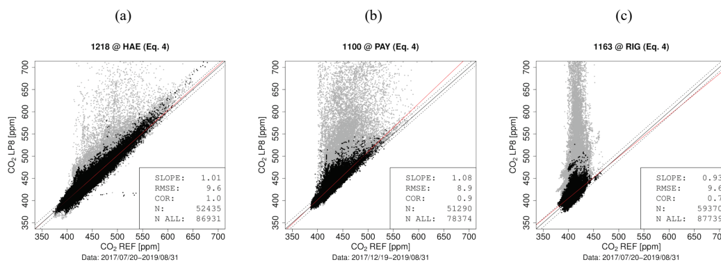
5 Figure 15: Comparison between LP8 and reference measurements. The LP8 measurements are outlier screened, drift corrected and checked for consistency. (a) Site HAE is located next to a motorway, (b) site PAY is located in a rural landscape, and (c) site RIG is an elevated background site. Points in grey are outliers.
