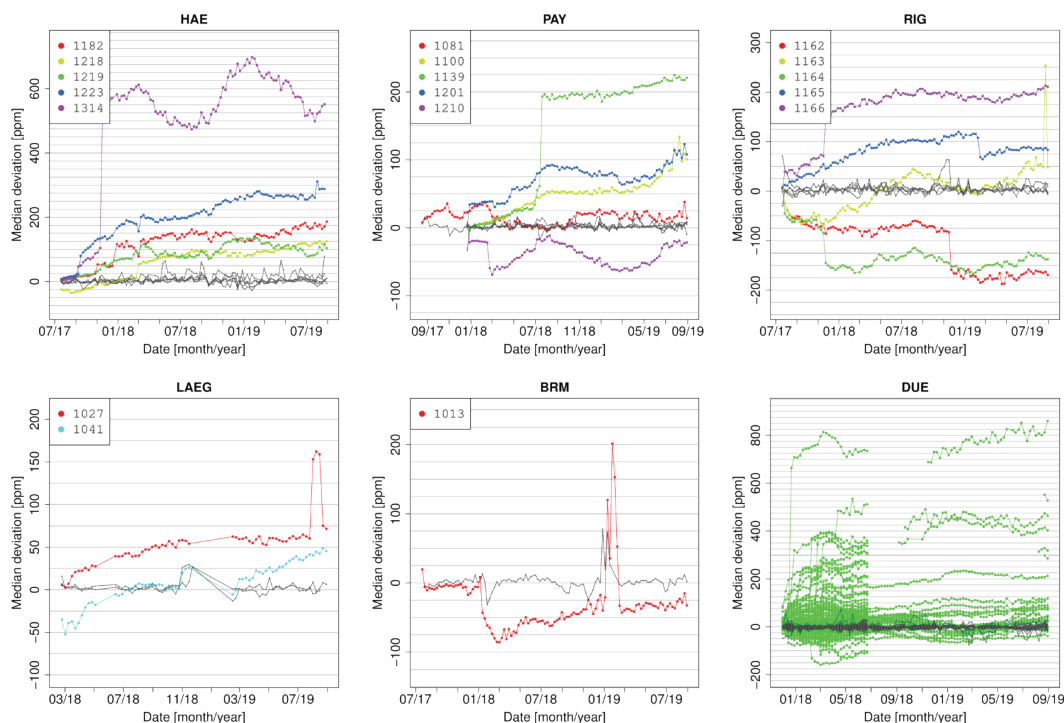
Figure 9: Weekly median deviation of sensors operated in HAE, PAY, RIG, LAEG, BRM and DUE before (coloured) and after drift correction (grey). Note the different scales in the y-axis.
