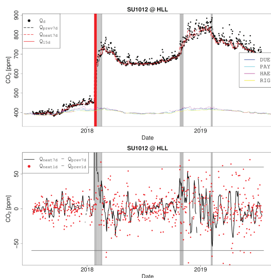
Figure 5: (a) Time series of Q_d , Q_{prev7d} , Q_{next7d} and Q_{15d} for sensor unit 1012 deployed in Hallau (HLL). The red vertical lines depict days when |Q_{next7d} - Q_{prev7d}| is larger than the threshold. Shaded periods indicate time periods with increased |b_{15d}| . For comparison, the Q_{15d} values for the reference sites DUE, PAY, RIG and HAE are shown. (b) Time series of Q_{next7d} - Q_{prev7d} and Q_{next1d} - Q_{prev1d} for the same sensor. The horizontal lines depict the threshold \Delta Q_{TRSH} .
