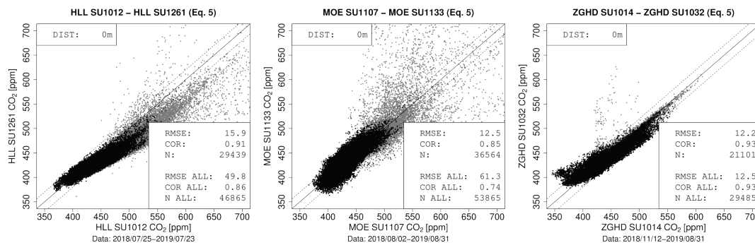
Figure 12: Comparison of LP8 measurements (drift corrected, outlier detection algorithm) from co-located sensors (distance between sensors < 45 m). Points in grey are flagged as outliers. The header of the individual figures indicates the sensor pairs by the location name and the sensor unit ID as well as the sensor model.
