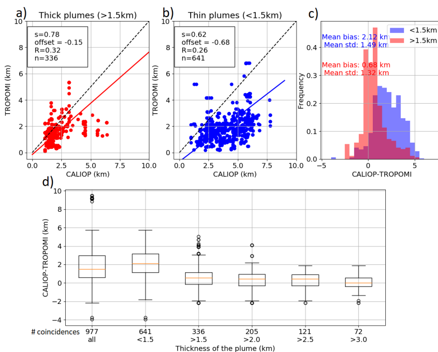
Figure 4. CALIOP-TROPOMI comparison for (a) thick plumes (>1.5 km) and (b) thin plumes (<1.5 km), together with the statistics of the line of best fit (correlation coefficient, R , slope, s , and number of observations, n ). The plume thickness is determined by the CALIOP top and base plume height. (c) shows the histogram for the differences in plume height (CALIOP-TROPOMI) for thick (red) and thin (blue) plumes. (d) shows the statistics for different plume thickness filters.
