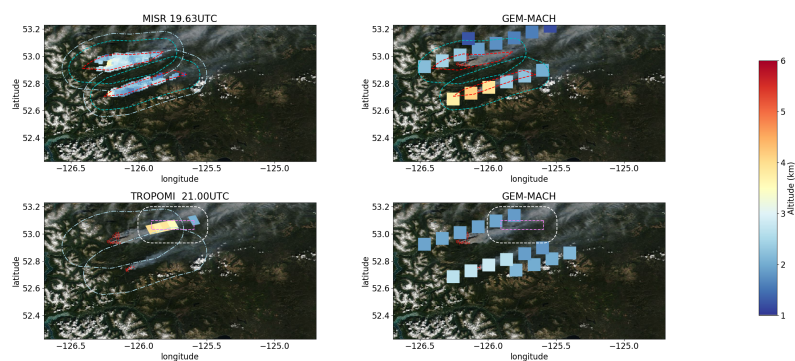
Figure 2. Example of two fire plumes on 6 August 2018 in British Columbia, Canada (approximately 56^{\circ}\text{N} , 126^{\circ}\text{W} ). The color scheme illustrates the altitude of the plume (a) as observed by MISR at 19:38 UTC, (b) modeled in GEM-MACH using CFFEPS at 19:38 UTC, (c) observed by TROPOMI at 21:00UTC, and (d) modeled by GEM-MACH using CFFEPS at 21:00 UTC. The dashed lines outline the shape of the plume as used for the comparison (see text for further details). (Underlying VIIRS images obtained from NASA Worldview ( https://worldview.earthdata.nasa.gov/ ))
