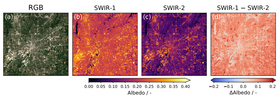
Fig. 1. (a) True color RGB for the city of Indianapolis. Corresponding surface reflectance/albedo data in SWIR-1 (b) and SWIR-2 (c) as well as the difference between SWIR-1 and SWIR-2 (d).
