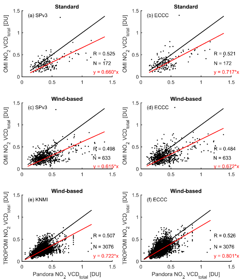
Figure 9. OMI and TROPOMI vs. Pandora no. 104 (Downsview) NO 2 total columns, using (a, b) the standard coincidence comparison method for OMI SPv3 and OMI ECCC, respectively; (c, d) wind-based method for OMI SPv3 and OMI ECCC, respectively. (e) and (f) are results using the wind-based method for TROPOMI KNMI and ECCC, respectively, with extended y_{rotate} range. On each scatter plot, the red line is the linear fit with intercept set to 0, and the black line is the one-to-one line.
