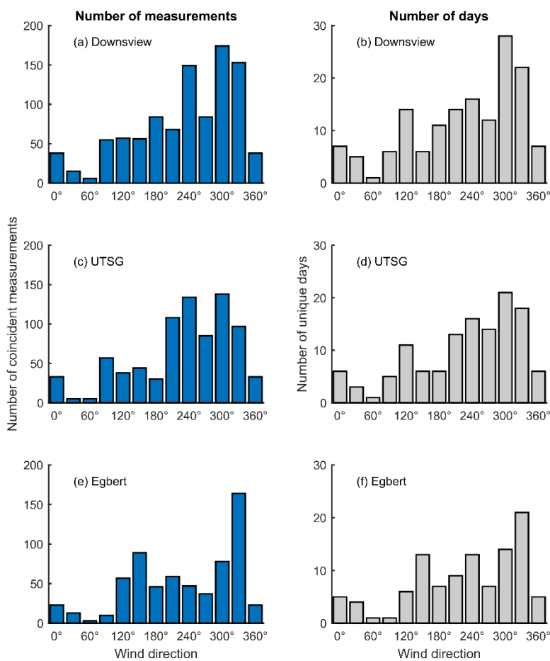
Figure 8. The number of coincidences of TROPOMI and Pandora measurements and number of unique days for each wind-bin for the data shown in Figures 6 and 7.
