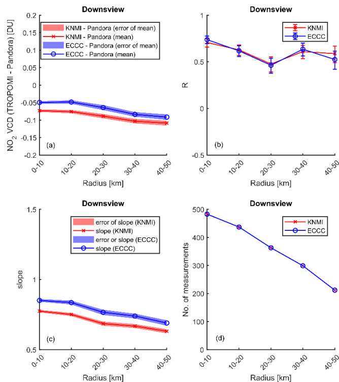
5 Figure B1. Sensitivity test for Pandora no. 104 at Downsview. For data within each radius bin, (a) shows the mean difference between TROPOMI and Pandora NO 2 VCD total , (b) shows the correlation coefficients, (c) shows the slope (zero offset linear fit), and (d) shows the number of coincident measurements. KNMI data are shown in red, ECCC data are shown in blue. The (a) symmetric standard error of mean and (c) error of slope are shown by colour-coded envelopes, indicated by the legends. The asymmetric error of the correlation coefficients is shown by error bars in (b and d).
