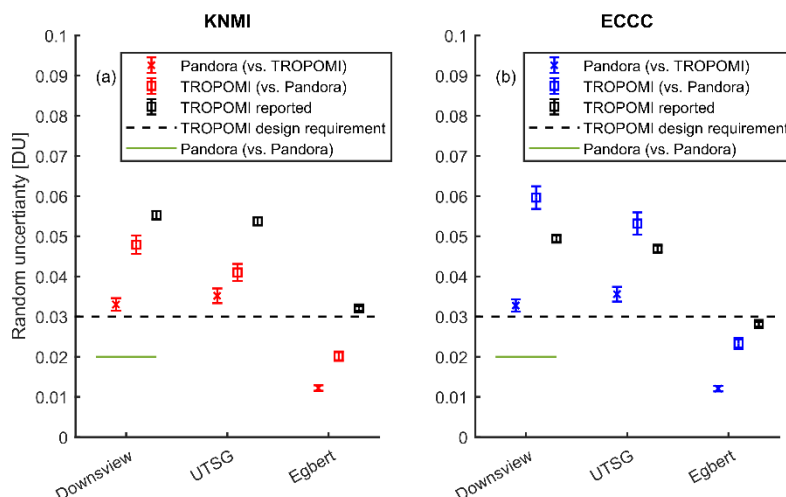
5 Figure 12. Statistical uncertainty estimations for TROPOMI and Pandora total column NO 2 , using their coincident measurements paired by wind-based methods. (a) TROPOMI KNMI vs. Pandoras at three sites (site names are on the x-axis), the estimated statistical random uncertainties are shown in red with estimated errors. Black squares represent the mean of reported uncertainties for TROPOMI KNMI NO 2 data, with error bars representing the uncertainty of the mean. (b) TROPOMI ECCC vs. Pandoras at three sites (x-axis), the estimated statistical random uncertainties are shown in blue with estimated errors. Black squares represent the mean of reported uncertainties for TROPOMI ECCC NO 2 data, with error bars representing the uncertainty of the mean. The black dashed line is the TROPOMI design requirement for precision, while the green line is the Pandora instrument precision estimated independently (statistical estimation using co-located Pandoras at Downsview).
