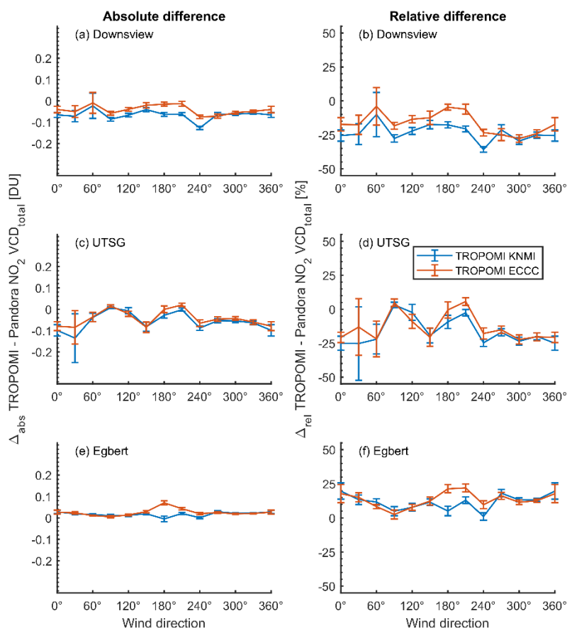
5 Figure 7. The absolute and relative differences between TROPOMI and Pandora coincident measurements from three sites, binned by wind direction. TROPOMI and Pandora absolute differences are shown in (a), (c), and (e); their relative differences are shown in (b), (d), and (f). Blue lines are differences calculated using TROPOMI KNMI data products, red lines are their counterparts using ECCC data products. Error bars are the standard error of the mean.
