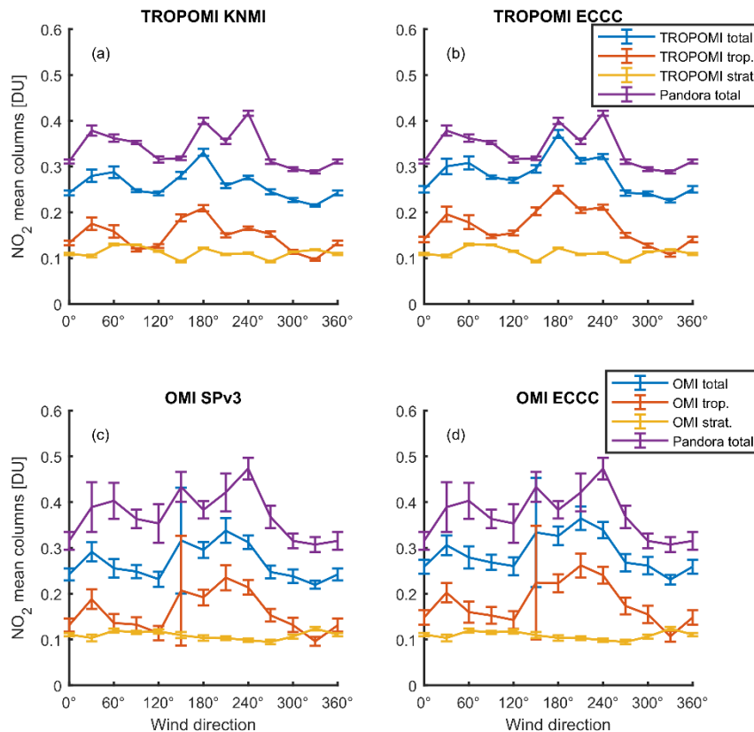
Figure 10. TROPOMI, OMI, and coincident Pandora measurements from Downview, binned by wind direction. TROPOMI data in (a) are from KNMI products and (b) are from ECCC products (2018). OMI data in (c) are from NASA SPv3 products and (d) are from ECCC products (2015-2018). Blue, red, and yellow lines are TROPOMI or OMI total, tropospheric, and stratospheric columns. Purple lines are Pandora total columns. Error bars are the standard error of the mean.
