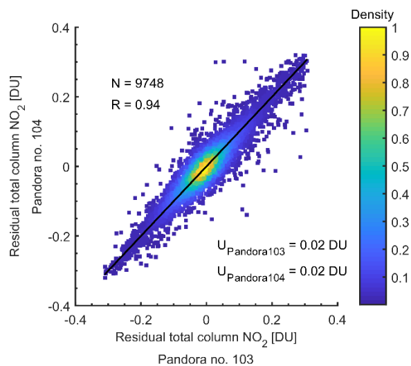
Figure 11. Scatter plot of residual total column NO 2 measured by Pandora nos. 103 and 104 (2017 December to 2019 June), colour-coded by the normalized density of the points. The black line is the one-to-one line.
