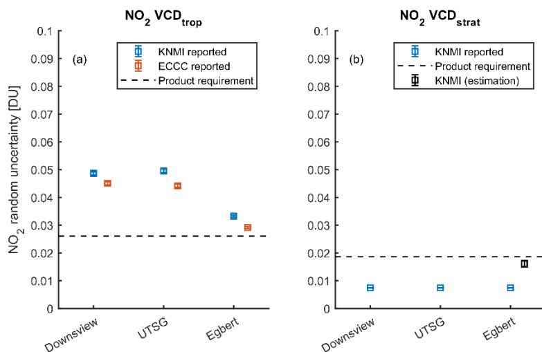
5 Figure C1. TROPOMI reported random uncertainties of (a) tropospheric and (b) stratospheric NO 2 columns. Blue squares are KNMI reported random uncertainties, with error bars from the uncertainty of the mean. Red squares are ECCC reported random uncertainties. The black dash lines are the design requirements. The black square represents the estimated uncertainty of KNMI stratospheric data.
