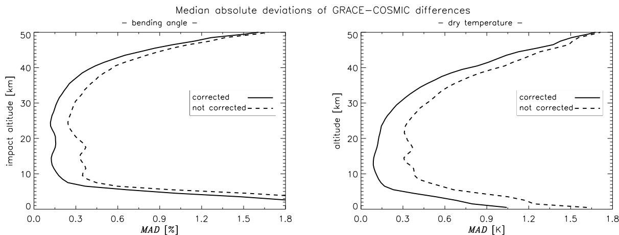
Figure 12. Median absolute deviations of GRACE-COSMIC differences computed from all monthly bins in 1-km height intervals during the mission overlap period March 2007 to December 2016; deviations for bending angles to the left and for dry temperature to the right. The solid lines show deviations with sampling-error correction applied, and the dashed lines show deviations without correction.
