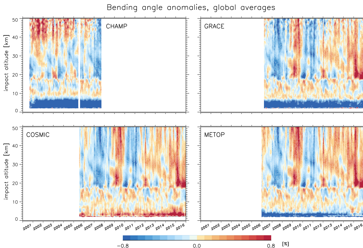
Figure 7. Global monthly mean bending angle anomalies, for the four RO missions included in the ROM SAF Climate Data Record v1.0. There is overlap between CHAMP and COSMIC from August 2006 to September 2008, between GRACE and COSMIC from March 2007 to December 2016, and between Metop and COSMIC from December 2006 to December 2016. Data are given on a 5 degrees by 200 meter latitude-altitude grid and have been sampling-error corrected. The anomalies for the four satellite missions are computed based on the same reference climatology, obtained from RO data itself.
