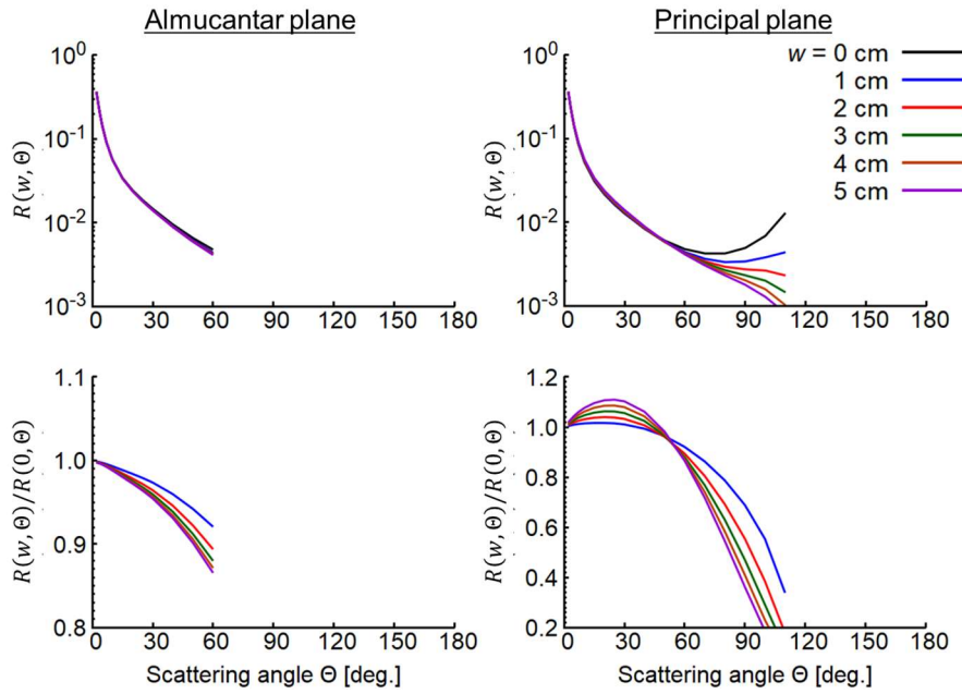
Figure 5: Similar to Fig. 4 but for \text{SZA} = 30^\circ .
