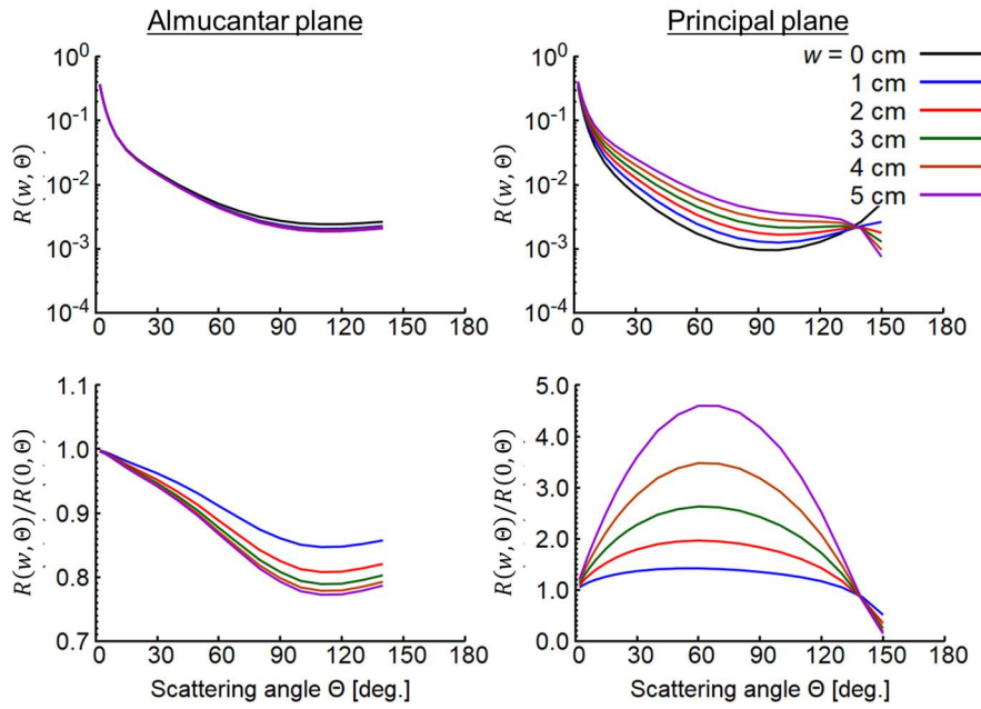
Figure 4: Normalized angular distributions simulated for transported dust aerosol (Table 21) in the almucentar and principal planes with an aerosol optical thickness of 0.06 at 940 nm. The s Simulations were conducted for \text{SZA} = 70^\circ and \text{PWV} (w) = 0, 1, 2, 3, 4, \text{ and } 5 \text{ cm} . The top row is the normalized radiance R(w, \Theta) , and the bottom row is the ratio of R(w, \Theta) to R(0, \Theta) .
