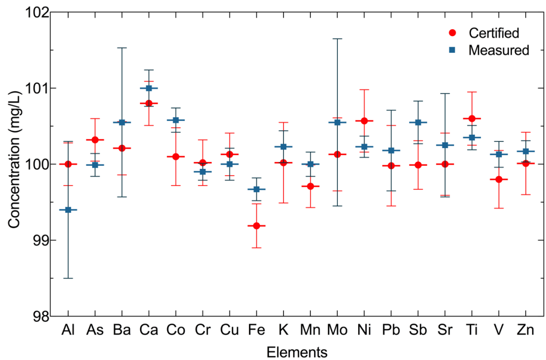
885 Figure 2: Good agreement observed between measured and certified values of metals in the multi-element standard solution.
