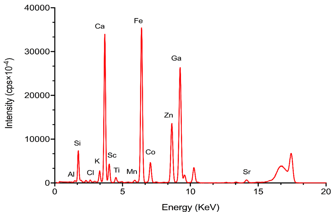
900 Figure 5: TXRF spectra of particulate matter PM10 samples collected at the AM5 station and measured with the Mo-excitation anode for their metal element.
