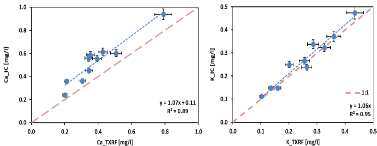
895 Figure 4: Comparison of Ca and K values of aerosol extracts in water measured by TXRF and ion Chromatography ICS 9000.
