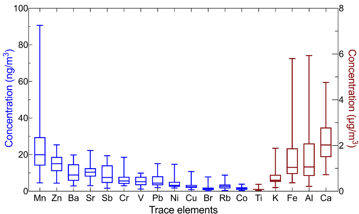
905 Figure 6: Box plots of ambient aerosol trace metal concentrations observed at the AM5 station during August and early September 2017
