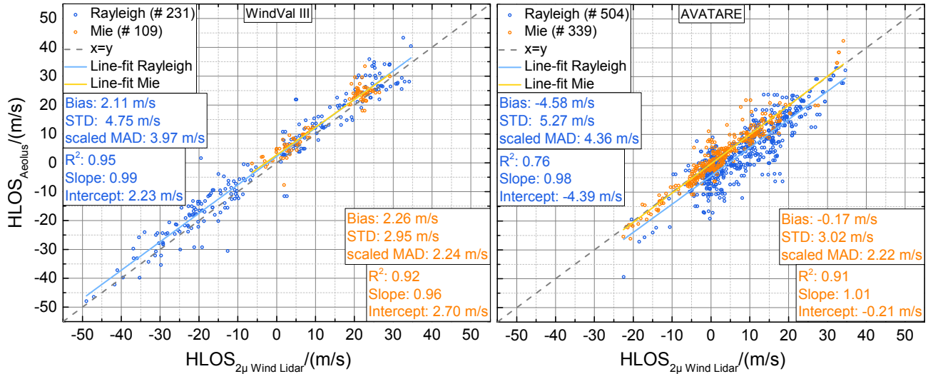
Figure 7. Aeolus HLOS wind speed plotted against the 2- \mu\text{m} DWL wind speed projected onto the horizontal viewing direction of Aeolus for 8 flight legs from 4 underflights performed during the WindVal III campaign 2018 (left) and for 10 flight legs from 6 underflights performed during the AVATARE campaign 2019 (right) (see also Table 1). The wind measurements are separated in Rayleigh-clear winds (blue) and Mie-cloudy winds (orange). Corresponding least-square line fits are indicated by the light blue and yellow line, respectively. The fit results are shown in the insets. The x = y -line is represented by the gray-dashed line.
