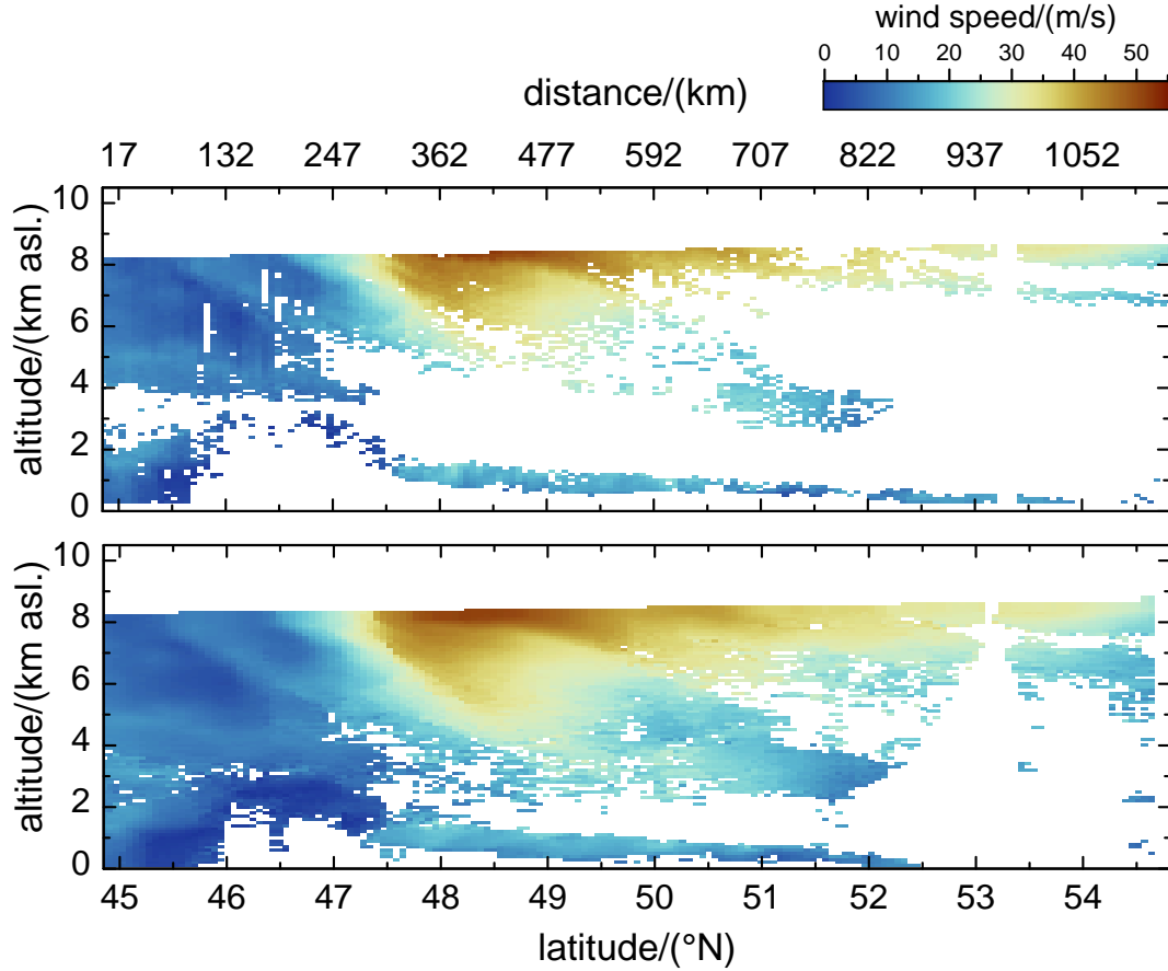
Figure 2. Wind speed retrieved from 2- \mu\text{m} DWL data by means of the MFAS algorithm for one scanner revolution (top) and five scanner revolutions and five range-gates with a sliding window (bottom), respectively during the first ever Aeolus underflight performed on 17 November 2018 during the WindVal III campaign (see also Table 1 and Fig. 1, left, red line). The flight leg ranges from 44.85°N to 54.82°N which corresponds to 1146 km track length. The leg started in the south at 15:57 UTC and ended in the north at 17:45 UTC. The satellite overflight was at around 17:02 UTC. White colors indicate areas with no valid wind measurements due to aerosol-poor atmospheric conditions and a corresponding insufficient SNR.
