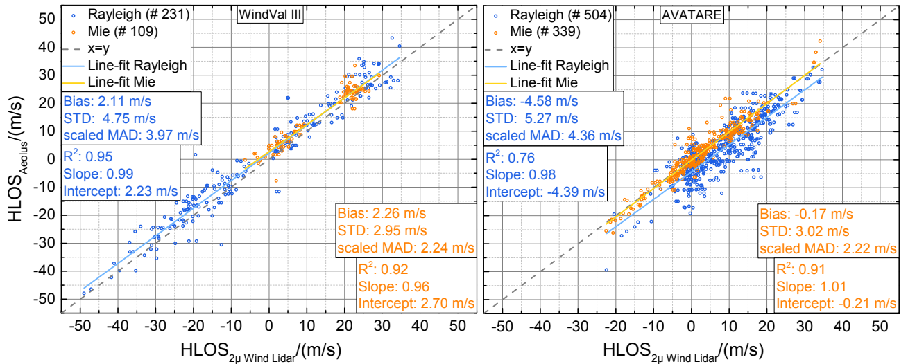
Figure 7. Aeolus HLOS wind speed plotted against the 2\text{-}\mu\text{m} DWL wind speed projected onto the horizontal viewing direction of Aeolus for 8 flight legs from 4 underflights performed during the WindVal III campaign 2018 (left) and for 10 flight legs from 6 underflights performed during the AVATARE campaign 2019 (right) (see also Table 1). The wind measurements are separated in Rayleigh-clear winds (blue) and Mie-cloudy winds (orange). Corresponding least-square line fits are indicated by the light blue and yellow line, respectively. The fit results are shown in the insets. The x = y -line is represented by the gray-dashed line.
