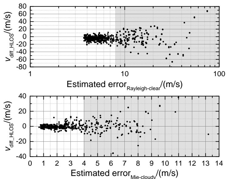
Figure 6. Wind speed difference of Aeolus HLOS winds and 2- \mu\text{m} DWL winds projected onto Aeolus viewing direction according to Eq. (2) depending on the estimated error given in the L2B product for Rayleigh-clear winds (top) and Mie-cloudy winds (bottom). Shown are all valid data points from WindVal III and AVATARE. Data points with an estimated error larger than 8 m/s (Rayleigh) or rather 4 m/s (Mie) are not considered as valid observations (gray areas).
