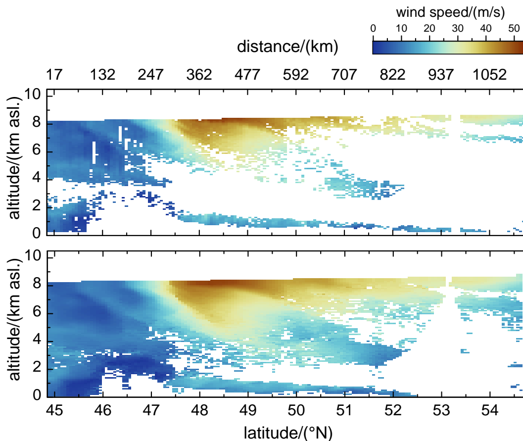
Figure 2. Wind speed retrieved from 2- \mu\text{m} DWL data by means of the MFAS algorithm for one scanner revolution (top) and five scanner revolutions and five range-gates with a sliding window (bottom), respectively during the first ever Aeolus underflight performed on 17 November 2018 during the WindVal III campaign (see also Table 1 and Fig. 1, left, red line). The flight leg ranges from 44.85°N to 54.82°N which corresponds to 1146 km track length. The leg started in the south at 15:57 UTC and ended in the north at 17:45 UTC. The satellite overflight was at around 17:02 UTC. White colors indicate areas with no valid wind measurements due to aerosol-poor atmospheric conditions and a corresponding insufficient SNR.
