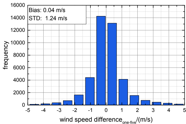
Figure 3. Histogram of the difference of wind speeds derived from 2- \mu m DWL data by means of one scanner revolution and five scanner revolutions ( v_{2\mu m_{1\text{-scan}}} - v_{2\mu m_{5\text{-scans}}} ) for all flights performed during the AVATARE campaign (see also table 1). The mean and the standard deviation (STD) of the data are indicated by the inset.
