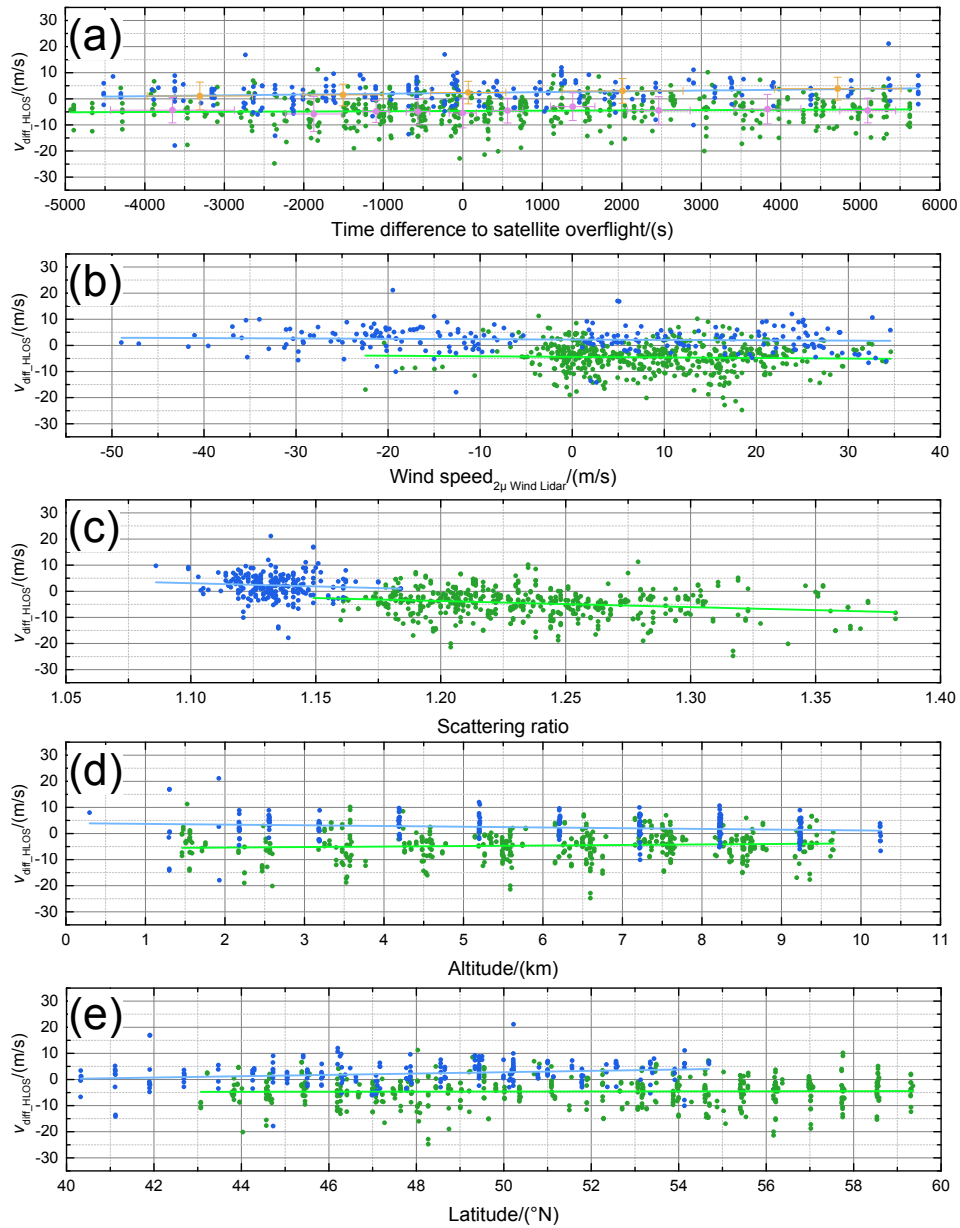
Figure 8. Wind speed difference of Aeolus Rayleigh-clear winds and 2- \mu m DWL winds calculated according to Eq. (2) depending on time difference of 2- \mu m DWL observation to satellite overflight time (a), wind speed (b), scattering ratio (c) and altitude (d) and latitude (e). Data points of the WindVal III and AVATARE campaign are indicated in blue and green, respectively. Least-square line-fits to the data points are represented by the light blue and light green lines. In plot (a), the mean of 50 subsequent data points and the corresponding standard deviation (error bars) are show for WindVal III (orange) and AVATARE (magenta).
