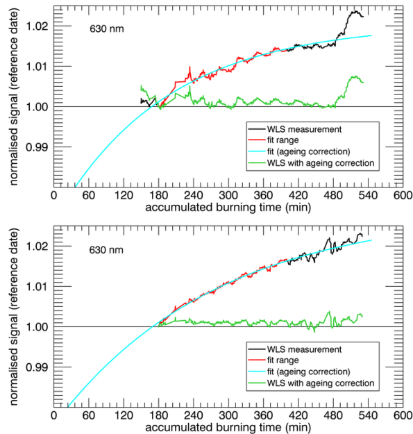
Figure 5. Relative WLS intensity at 630 nm as a function of its accumulated burning time in orbit. Top: WLS measurements in ESA V9.01 calibration; bottom: after the final iteration of the modified degradation model. The black curve shows the WLS measurements. The (fit) range that is used to derive the parameterization of the WLS change is indicated in red . The best fit to describe the ageing of the WLS is plotted in light blue . In green , the corrected WLS measurements as used in the degradation model is shown.
