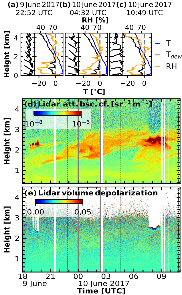
Figure 12. (a-c) same as Fig. 9 but for 9 June 2017 18:00 UTC – 10 June 2017 11:00 UTC up to 5 km height. (d+e) measurements from Polly XT between 9 June 2017, 18:00 UTC – 10 June 2017, 11:00 UTC. In (d) and (e), the 1064-nm attenuated backscatter coefficient and the 532-nm volume depolarization are shown, respectively. The black dashed lines mark the time of the radiosonde launches as shown in (a-c). The grey box indicates the period used for averaging in Fig. 13.
