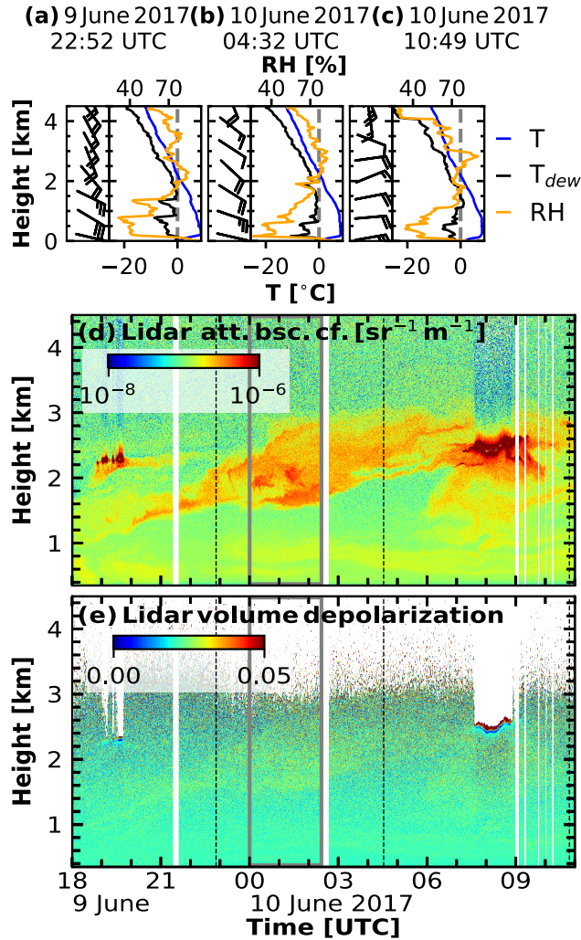
Figure 12. (a-c) same as Fig. 9 but for 9 June 2017 18:00 UTC – 10 June 2017 11:00 UTC up to 4.5 km height. (d+e) measurements from Polly XT between 9 June 2017, 18:00 UTC – 10 June 2017, 11:00 UTC. In (d) and (e), the 1064-nm attenuated backscatter coefficient and the 532-nm volume depolarization are shown, respectively. The black dashed lines mark the time of the radiosonde launches as shown in (a–c). The grey box indicates the period used for averaging in Fig. 13.
