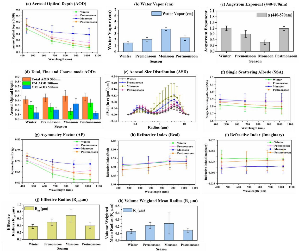
Figure 7. Seasonal mean variations in aerosol products.
