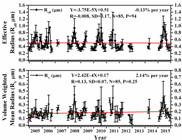
Figure 10. Long-term monthly mean variation of Effective radius ( R_{eff}\mu\text{m} ) and Volume weighted mean radius ( R_v\mu\text{m} ). Vertical bar at each data point represents standard deviation from mean.
