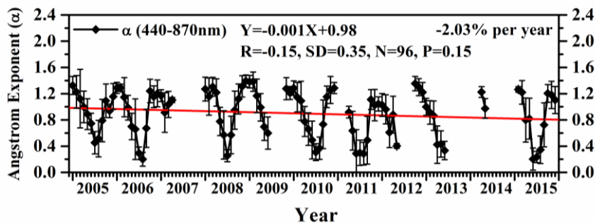
Figure 12. Monthly mean variation of Angstrom Exponent (AE) during the study period. Vertical bar at each data point represents standard deviation from mean. Solid red line indicates long-term decreasing trend.
