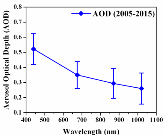
315 Figure 5. Composite spectral AOD variations from one-decade Cimel measurements at Pune, India. Vertical bar at each data point represents standard deviation from mean.
