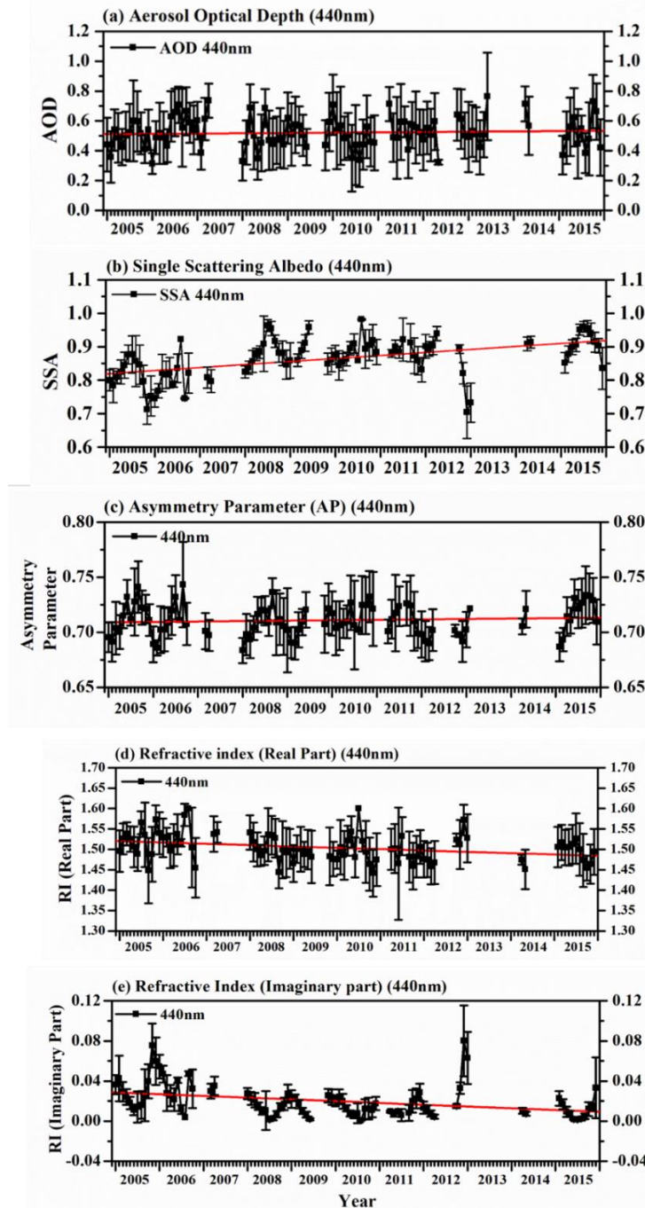
Figure 9. Long-term trends in aerosol products at 440 nm.
