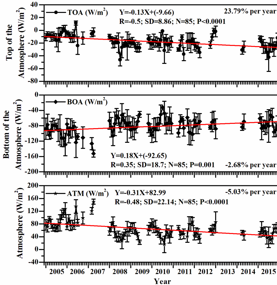
Figure 14. Long-term monthly mean variation in radiative forcing at Top of the Atmosphere (TOA; Wm^{-2} ), Bottom of the Atmosphere (BOA; Wm^{-2} ), and in the Atmosphere (ATM; Wm^{-2} ). Vertical bar at each data point represents standard deviation from mean.
