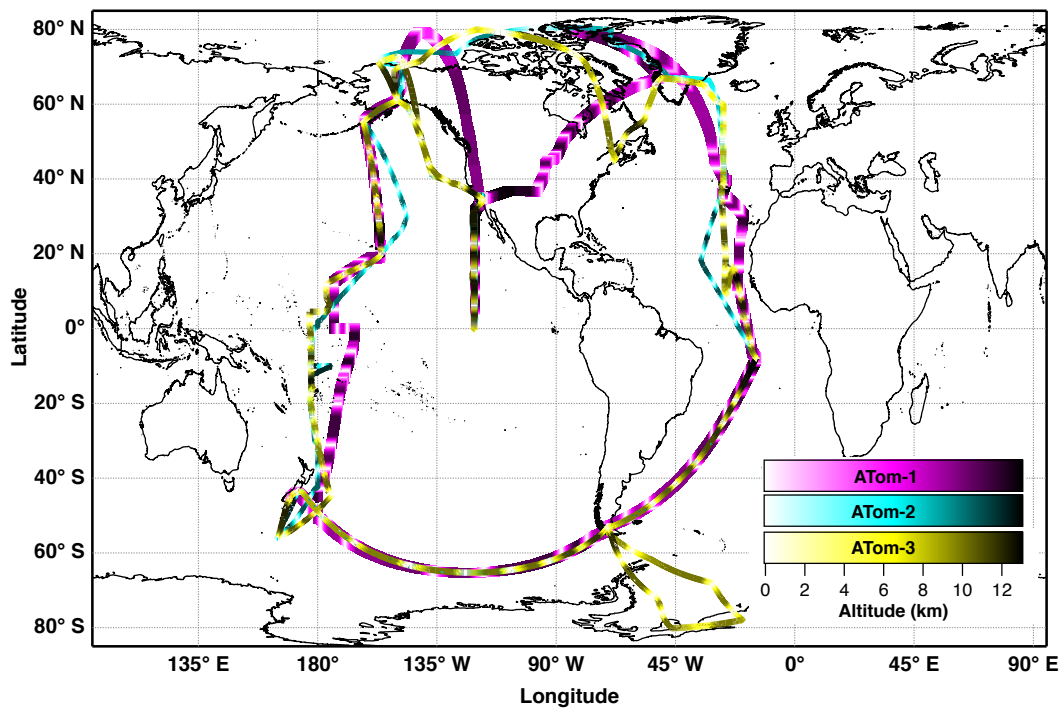
Figure 1. Flight tracks of the NASA DC-8 for ATom-1 (magenta), ATom-2 (cyan), and ATom-3 (yellow), shaded to show altitude.
