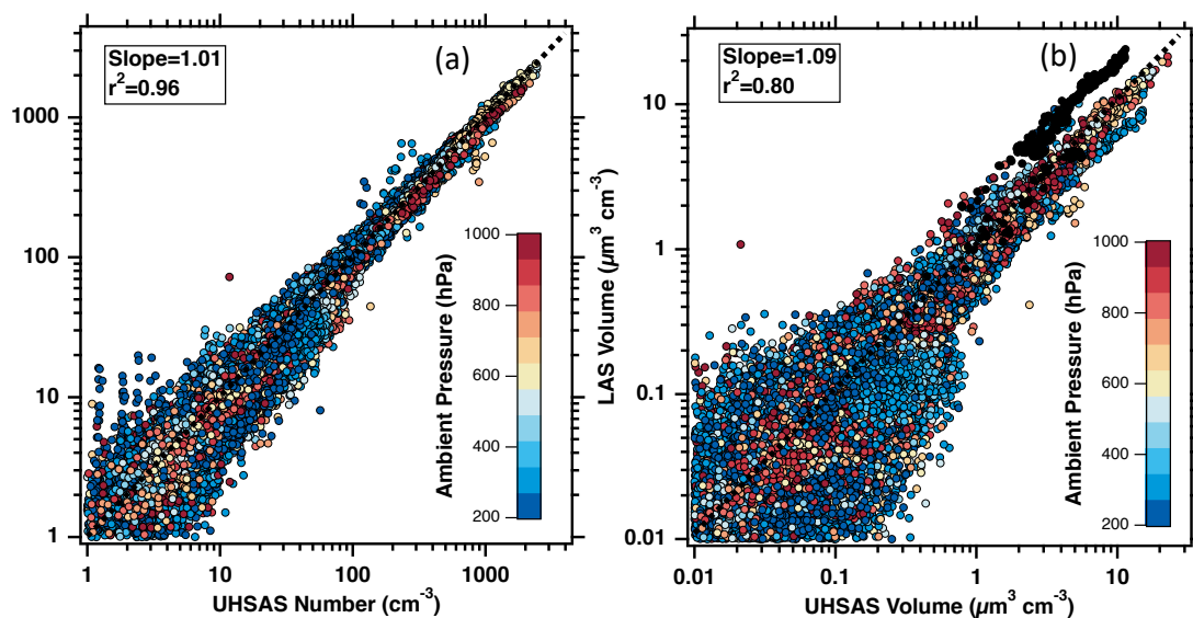
Figure 7. (a) Integrated ten-second average particle number concentrations from 0.104 to 0.97 \mu\text{m} diameter from the UHSAS and LAS instruments for all of the ATom-1 deployment. (b) As for (a), but for integrated particle volume. Colors indicate ambient pressure. Slopes from two-sided least squares regressions forced through a zero intercept are shown. Values of r^2 are from a one-sided linear least-squares regression. Black points in the volume plot show periods of dust from Africa.
