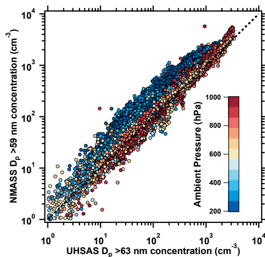
Figure 8. Ten-second particle number concentration from the largest NMASS CPC channel as a function of the concentration measured by the non-thermodenuded UHSAS for all of the ATom-1 deployment. Line is the 1:1 ratio. The NMASS concentrations are higher than the UHSAS concentrations at lower pressures because the aerosol size distribution is more steeply sloped toward smaller particles, while within the boundary layer the accumulation mode dominates.
