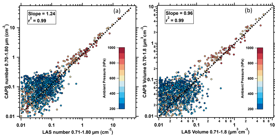
Figure 10. (a) One-minute average CAPS number concentrations for diameters from ~0.7-1.80 μm plotted against the same parameter from the LAS instrument for periods of flight during ATom-1 when RH with respect to liquid water was <40 %. (b) As in (a), but for particle volume. Lines and slopes are from two-sided least-squares linear regression forced through zero.
