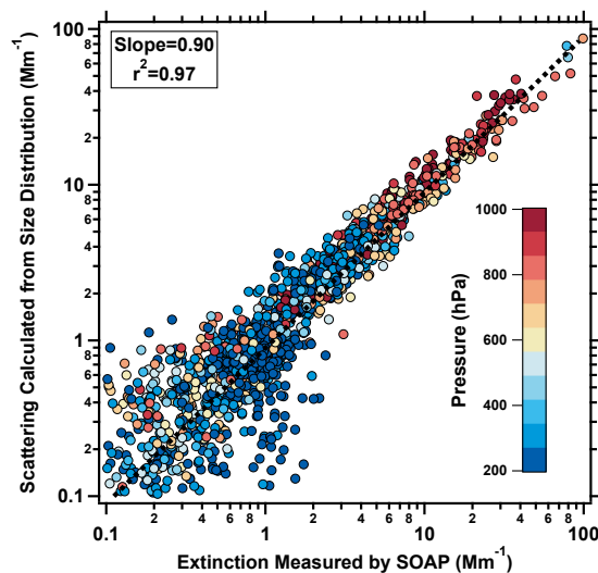
Figure 12. Dry aerosol scattering at 532 nm calculated using Mie theory from the particle size distributions measured by the NMASS, UHSAS, and LAS instruments as a function of the dry aerosol extinction at 532 nm measured directly by the SOAP instrument. Data are 60 s averages from the entire ATom-4 campaign. Line and slope are from a two-sided linear least-squares fit forced through zero intercept. Value of r^2 is from a one-sided linear least-squares regression.
