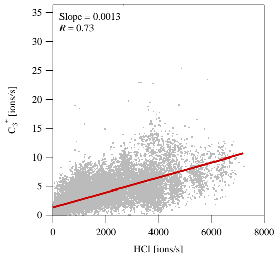
Figure 1. Signal comparisons between \text{C}_3^+ and \text{HCl} at m/z 36
