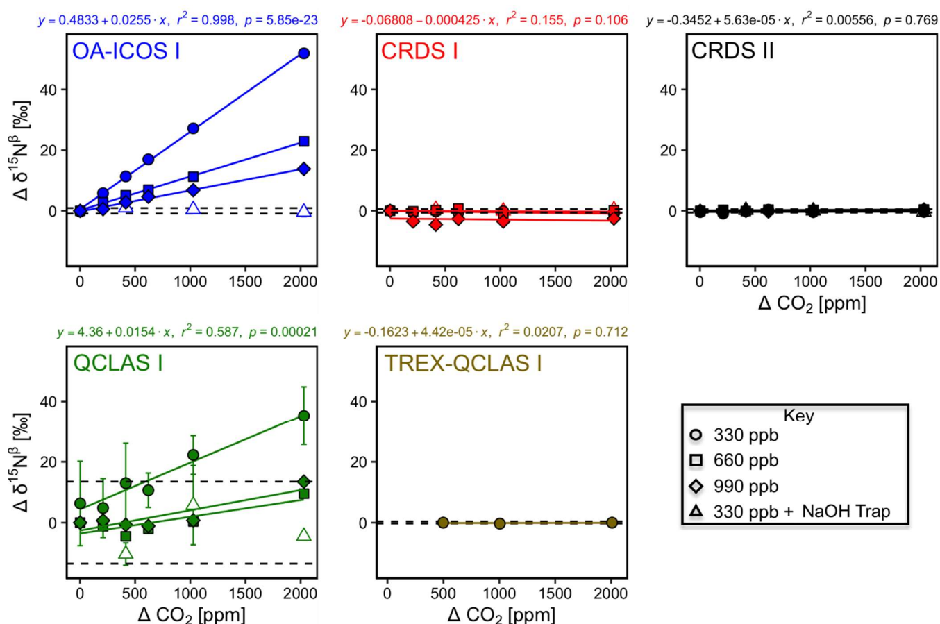
Fig. 7. Deviations of the measured [\text{N}_2\text{O}] , \delta^{15}\text{N}^{\alpha} , \delta^{15}\text{N}^{\beta} and \delta^{18}\text{O} values according to \Delta\text{CO}_2 (ppm) at different \text{N}_2\text{O} mole fractions (330, 660 and 990 ppb) for the OA-ICOS I (blue), CRDS I (red), CRDS II (black), QCLAS I (green) and TREX-QCLAS I (brown). The remaining plots for [\text{N}_2\text{O}] , \delta^{15}\text{N}^{\alpha} and \delta^{18}\text{O} are provided in Supplementary Material 4 (Fig. S4-6). The standard deviation of the Anchor gas ( \pm 1\sigma ) is indicated by dashed lines. Data points represent the mean and standard deviation ( 1\sigma ) of triplicate measurements. Dependencies are best-described by linear fits, which are indicated by solid lines.
