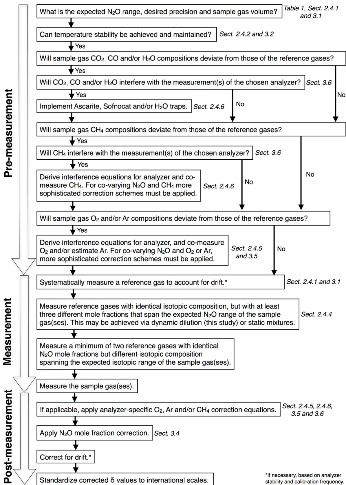
Fig. 15. Proposed measurement workflow for the operation of \text{N}_2\text{O} isotope laser spectrometers. Relevant sections of this study are shown next to each step.
