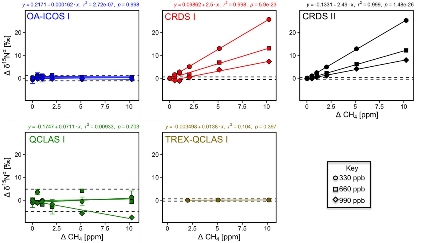
Fig. 8. Deviations of the measured [N 2 O], \delta^{15}\text{N}^\alpha , \delta^{15}\text{N}^\beta and \delta^{18}\text{O} values according to \Delta\text{CH}_4 (ppm) at different N 2 O mole fractions (330, 660 and 990 ppb) for the OA-ICOS I (blue), CRDS I (red), CRDS II (black), QCLAS I (green) and TREX-QCLAS I (brown). The remaining plots for [N 2 O], \delta^{15}\text{N}^\beta and \delta^{18}\text{O} are provided in Supplementary Material 4 (Fig. S4-7). Data points represent the mean and standard deviation (1 \sigma ) of triplicate measurements. Dependencies are best-described by linear fits, which are indicated by solid lines. Individual equations, coefficients of determination ( r^2 ) and p -values are indicated above each plot for the 330 ppb N 2 O data only.
