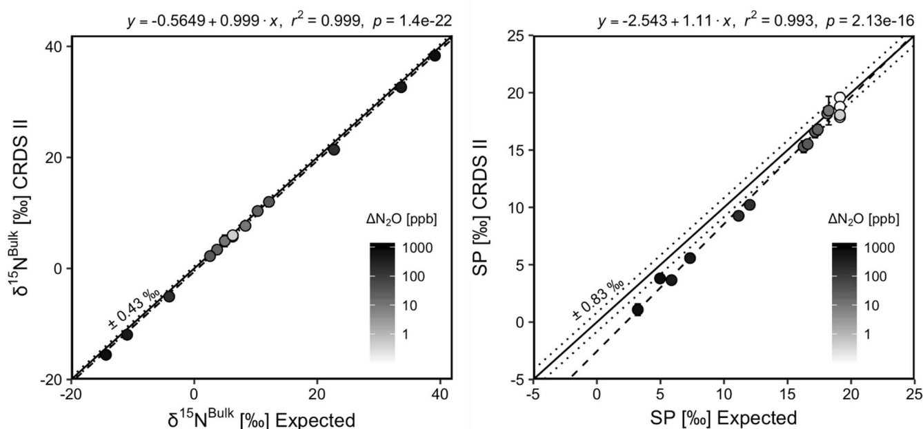
Fig. 11. Correlation diagrams for \delta^{15}N^{bulk} and SP measurements at various \Delta N_2O mole fractions analyzed by CRDS II plotted against expected values. The remaining plots for [N_2O] , \delta^{15}N^a , \delta^{15}N^b and \delta^{18}O are provided in Supplementary Material 4 (Fig. S4-12). The solid black line denotes the 1:1 line, while the dotted line indicates \pm 1\sigma of the residuals from the 1:1 line. The dashed black line represents a linear fit to the data. Individual equations, coefficients of determination ( r^2 ) and p -values are indicated above each plot. Each data point represents the mean and standard deviation ( 1\sigma ) of triplicate measurements. The inset plots indicate the standard deviation ( 1\sigma ) of the triplicate measurements achieved at different \Delta N_2O mole fractions, and the 1:1 line is similarly a solid line.
