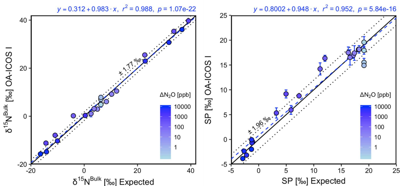
Fig. 9. Correlation diagrams for \delta^{15}\text{N}^{\text{bulk}} and SP measurements at various \Delta\text{N}_2\text{O} mole fractions analyzed by OA-ICOS I plotted against expected values. The remaining plots for [\text{N}_2\text{O}] , \delta^{15}\text{N}^a , \delta^{15}\text{N}^b and \delta^{18}\text{O} are provided in Supplementary Material 4 (Fig. S4-10). The solid black line denotes the 1:1 line, while the dotted line indicates \pm 1\sigma of the residuals from the 1:1 line. The dashed blue line represents a linear fit to the data. Individual equations, coefficients of determination ( r^2 ) and p -values are indicated above each plot. Each data point represents the mean and standard deviation ( 1\sigma ) of triplicate measurements. The inset plots indicate the standard deviation ( 1\sigma ) of the triplicate measurements achieved at different \Delta\text{N}_2\text{O} mole fractions, and the 1:1 line is similarly a solid line.
