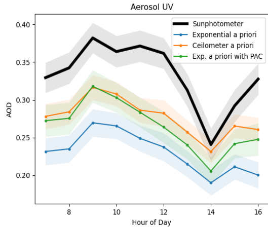
Figure 1: Time series of UV AOT (360 nm) over the day (2016-09-14) for different retrieval approaches compared to the sun photometer (in black). Blue: “standard” retrieval with an exponential a priori profile. Green: same retrieval, but with the PAC applied. Orange: Retrieval with scaled ceilometer profile as a priori.
