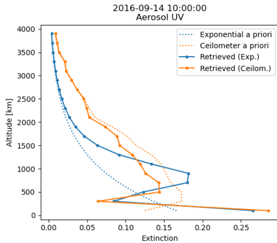
Figure 2: Example retrieved aerosol UV extinction profiles at 10h, together with the underlying a priori profiles. Colour coding is the same as in Fig. 1
