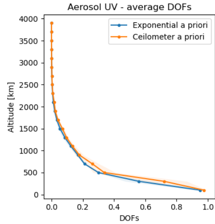
Figure 3: The average DOFs (AVK diagonal) for the aerosol UV extinction profile in the individual retrieved layers plotted over altitude. Colour coding is the same as in Fig. 1.
