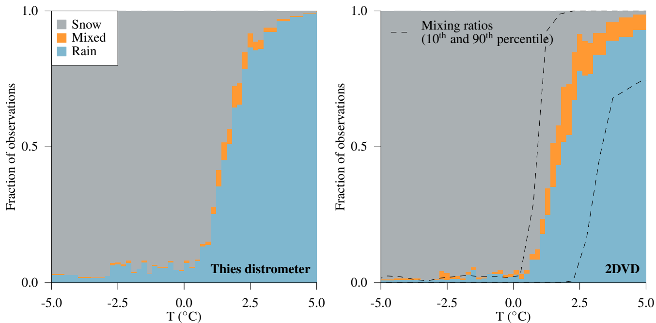
Figure 11. Relative frequency of the observed dominant precipitation phase by the Thies distrometer (left) and the two-dimensional video disdrometer (2DVD, right) as a function of air temperature during two years of measurements (2,533 h of precipitation). For the 2DVD, the mixing ratio of liquid precipitation obtained at different temperatures is indicated by the 10 th and 90 th percentile of its distribution (dashed lines).
