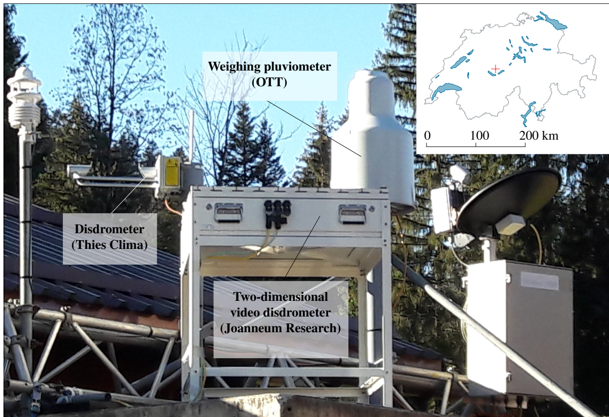
Figure 1. Measurement devices located in a pre-alpine area in Switzerland (Innereriz, 1060 m a.s.l.). In this study, the Thies disdrometer is evaluated using both the OTT pluviometer as well as a two-dimensional video disdrometer as a reference during two years of measurements.
