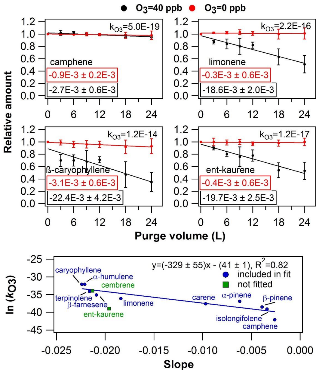
745 Figure 5. Results from ozone exposure experiments. In the upper panel plots are selected examples from the ozone exposure experiments presented as relative amount of compound in sorbent tube as a function of purge volume. The values embedded into the plots are the linear regression fit slopes ( \pm uncertainty) of corresponding conditions (either O 3 =0 ppb or O 3 =40 ppb). The compound specific k_{O_3} values are presented in the plots as well. The error bars represent reproducibility ( n=3 ). In the lower panel plot is presented the literature retrieved \ln(k_{O_3}) values (see Table S3) as a function of the linear regression fit slopes.
