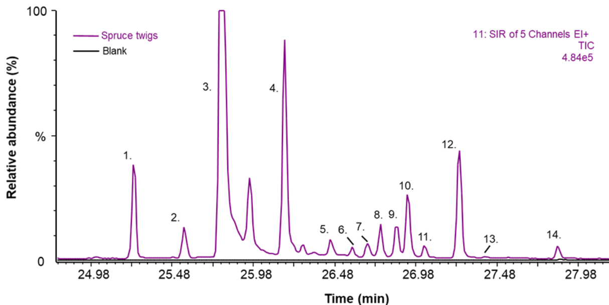
765 Figure 7. Selected ion recording (SIR) chromatograms from the TD-GC-MS1 analysis of spruce twigs and blank dynamic headspace sorbent tube samples (sampling at 60 °C for 20 min at flow rate of 100 mL/min). The five m/z ions included in the SIR were m/z 93, 229, 257, 272 and 275. The TIC is scaled for presentation purposes, peak number 3 is not showed in full height in order to visualize the other peaks more clearly. Peak identification: 1. Rimuene ( C_{20}H_{32} , DT), 2. Unknown ( C_{20}H_{32} , DT), 3. Cembrene ( C_{20}H_{32} , DT), 4. Cembrene A ( C_{20}H_{32} , DT), 5. Unknown ( C_{20}H_{32} , DT), 6. Unknown ( C_{20}H_{32} , DT), 7. Unknown ( C_{20}H_{32} , DT), 8. 13-epi-manool oxide ( C_{20}H_{34}O , DT), 9. Unknown ( C_{20}H_{32} , DT), 10. Unknown ( C_{19-20}H_{28-30} , BVOC), 11. Unknown ( C_{20}H_{34}O , DT), 12. Unknown ( C_{20}H_{32} , DT), 13. Abietatriene ( C_{20}H_{30} , DT) and 14. Unknown ( C_{20}H_{32} , DT). See Table S4 for further information on peak identification.
