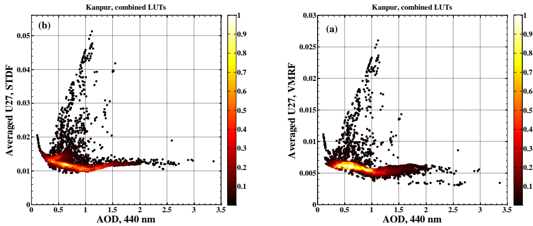
Figure 29. Uncertainties for a) volume median radius of fine mode and b) width of size distribution for fine mode estimated at Kanpur site.
