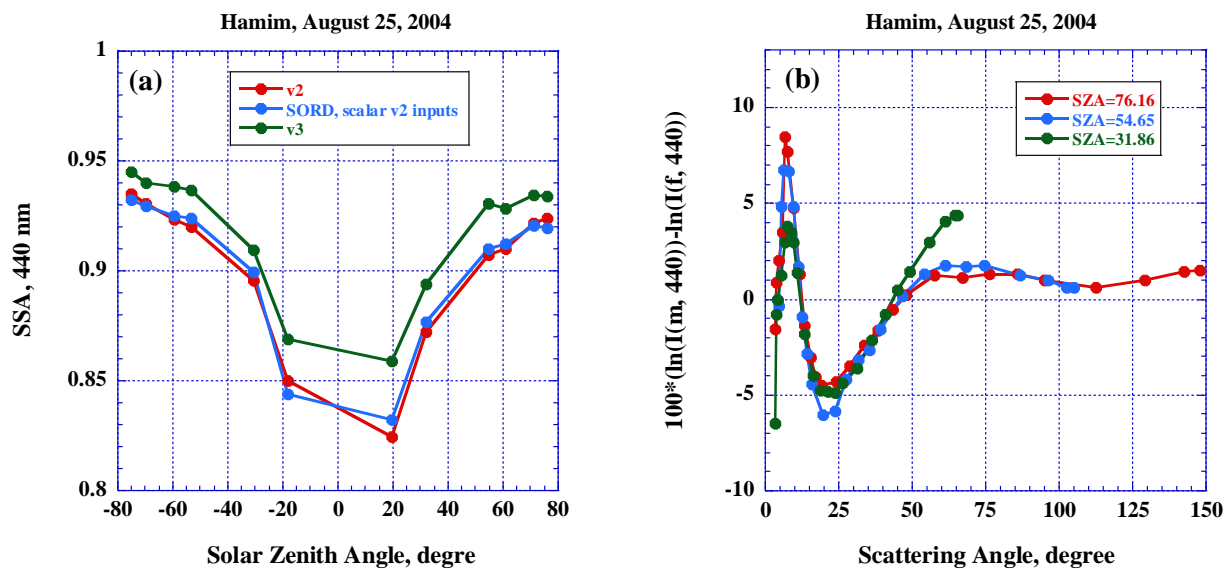
Figure 7. Data from Hamim (UAE) on 25 August 2004 showing a) diurnal variability of SSA at 440 nm retrieved from almucantars by the V2 and V3 algorithms and algorithm of V3 in scalar mode using inputs of V2 b) the relative percent difference between measured and fitted NSR at 440 nm for three different SZA.
