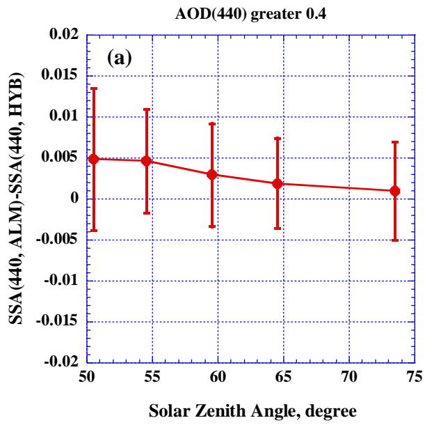
1925 Figure 17. Difference in SSA retrieved from HYB and ALM scans. a) 440 nm, b) 675 nm.
