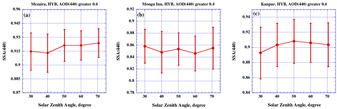
1830 Figure 13. Dependence of 440 nm SSA hybrid scan retrievals on SZA for three AERONET sites: a) Mezaira, b) Mongu Inn, c) Kanpur.
