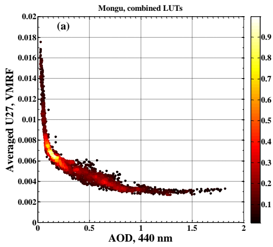
Figure 27. Uncertainties for a) volume median radius of fine mode and b) width of size distribution for fine mode estimated at Mongu site.
