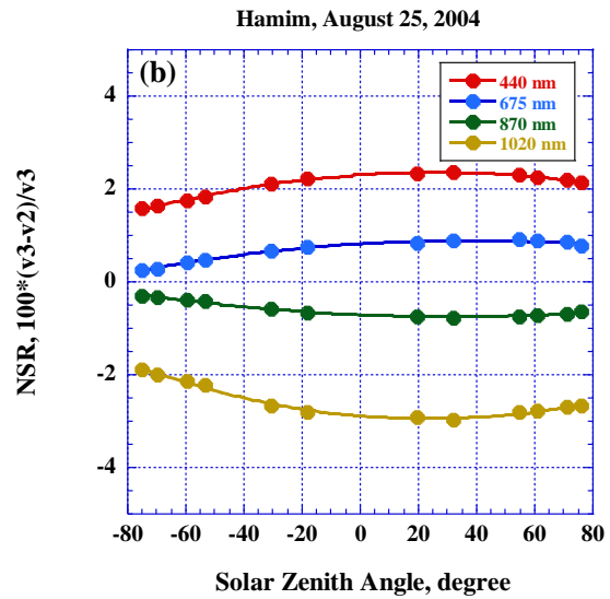
1690 Figure 6. Effect of solar flux and temperature correction on relative percent difference in normalized sky radiances for Hamim: a) joint effect of temperature correction and solar flux b) the effect of solar flux is subtracted.
