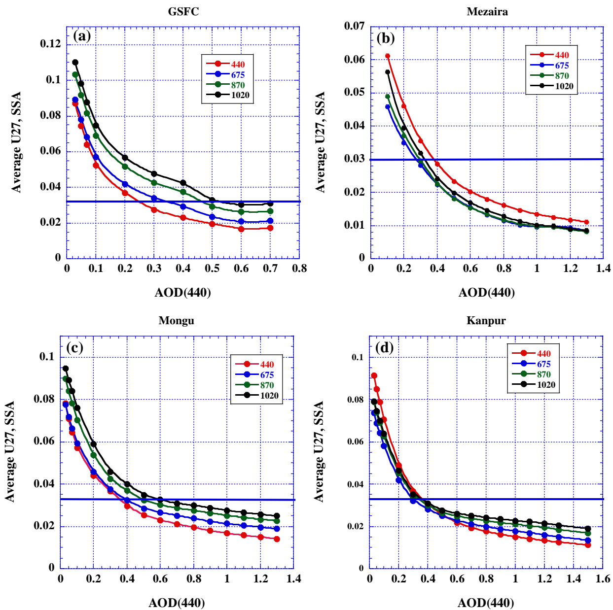
2010 Figure 22. SSA uncertainties generated by averaging over AOD bins with subsequent interpolation to the regularly spaced AOD grid; a) GSFC, b) Mezaira, c) Mongu, d) Kanpur.
