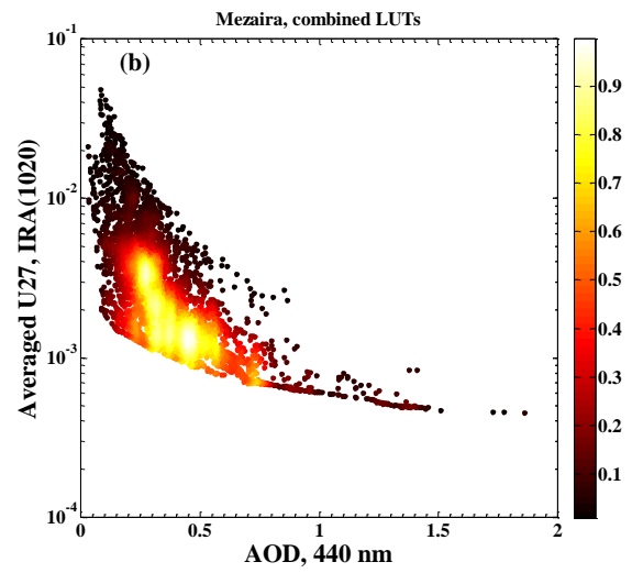
Figure 23 Uncertainties of the imaginary part of refractive index estimates, a) GSFC, b) Mezaira.
