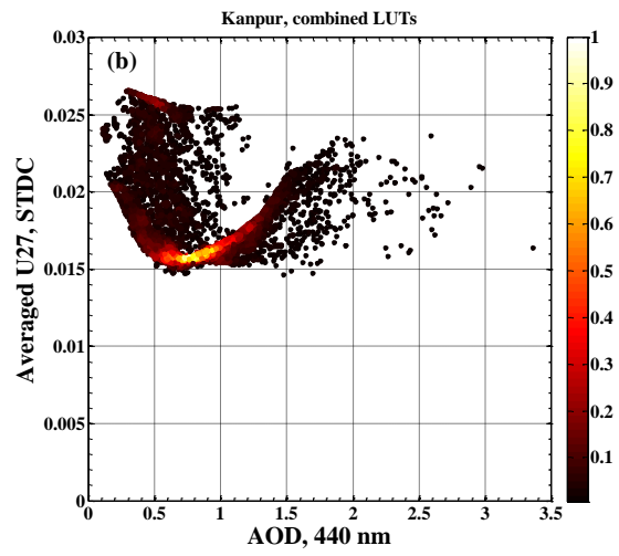
2180 Figure 30. Uncertainties for a) volume median radius of coarse mode and b) width of size distribution for coarse mode estimated at Kanpur site.
