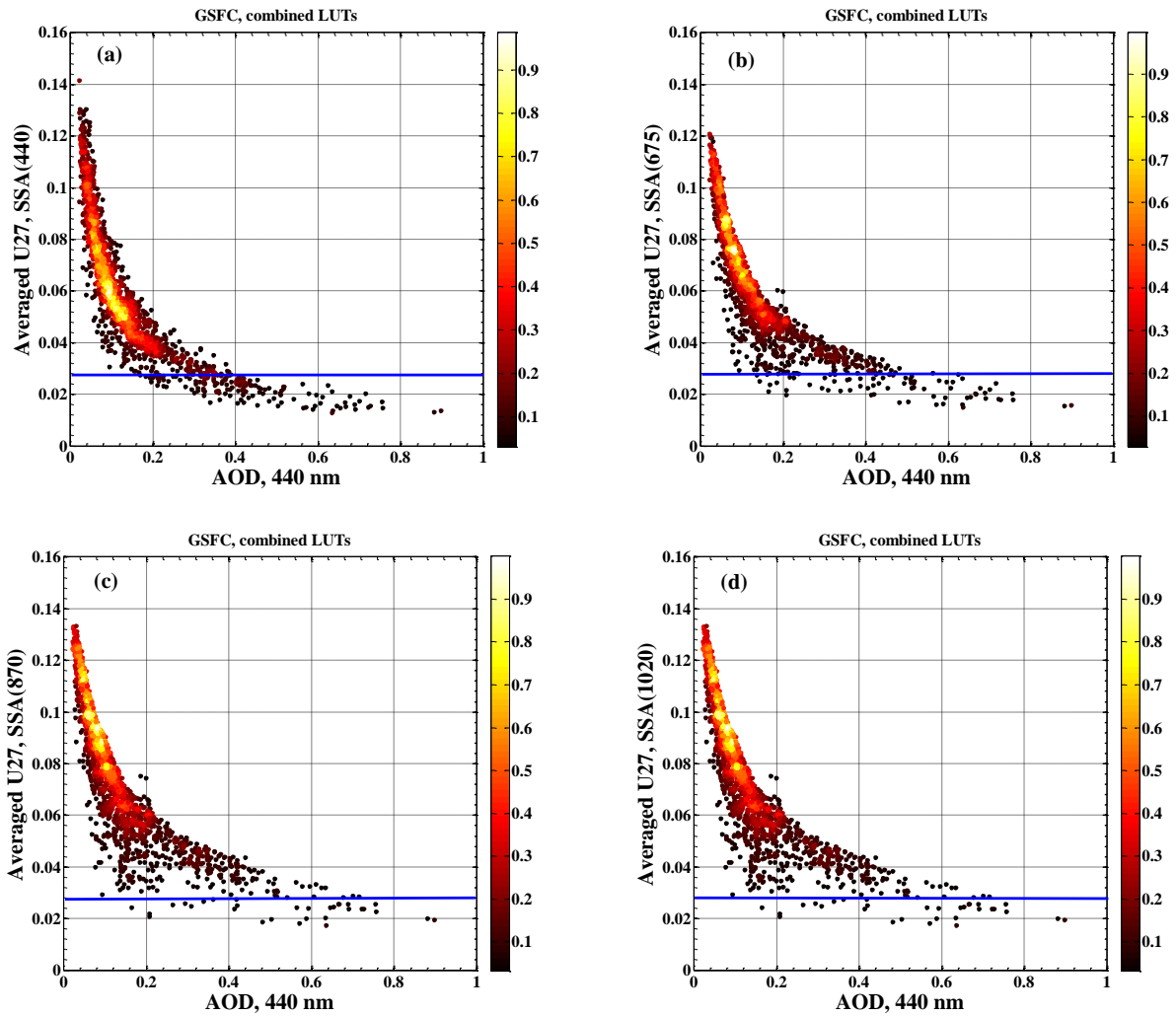
1990 Figure 20. Uncertainties for SSA retrievals at GSFC site, a) 440 nm, b) 675 nm, c) 870 nm, d) 1020 nm.
