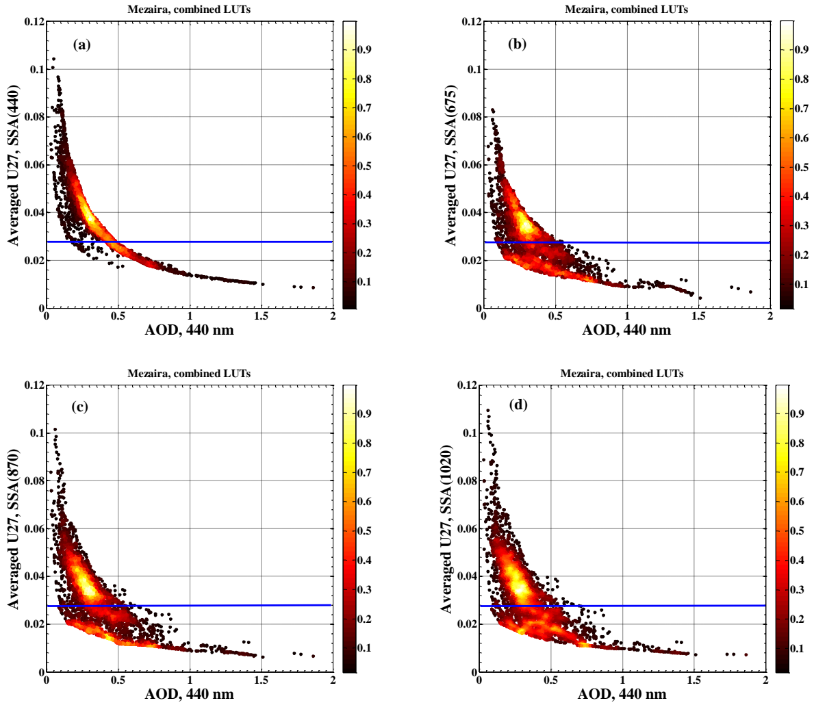
Figure 21. Uncertainties for SSA retrievals at Mezaira site, a) 440 nm, b) 675 nm, c) 870 nm, d) 1020 nm.
