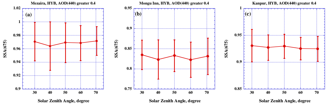
Figure 14. Dependence of 675 nm SSA hybrid scan retrievals on SZA for three AERONET sites: a) Mezaira, b) Mongu Inn, c) Kanpur.
