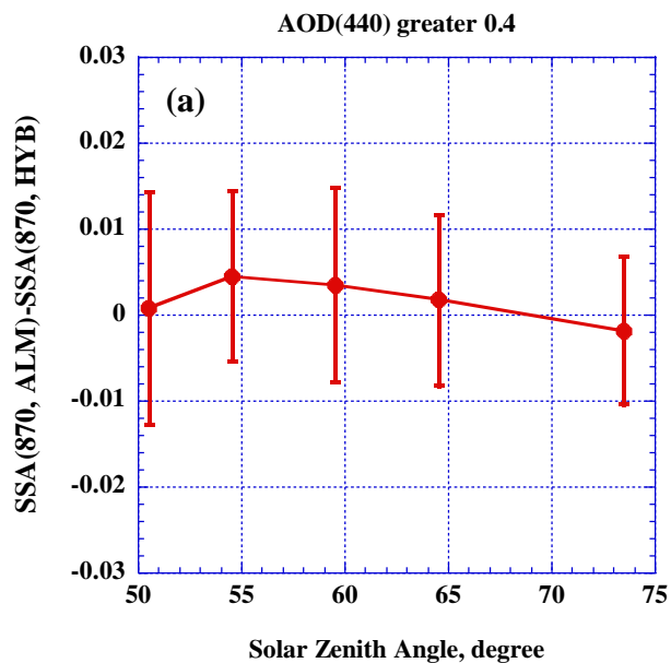
Figure 18. Difference in SSA retrieved from HYB and ALM scans. a) 870 nm, b) 1020 nm.
