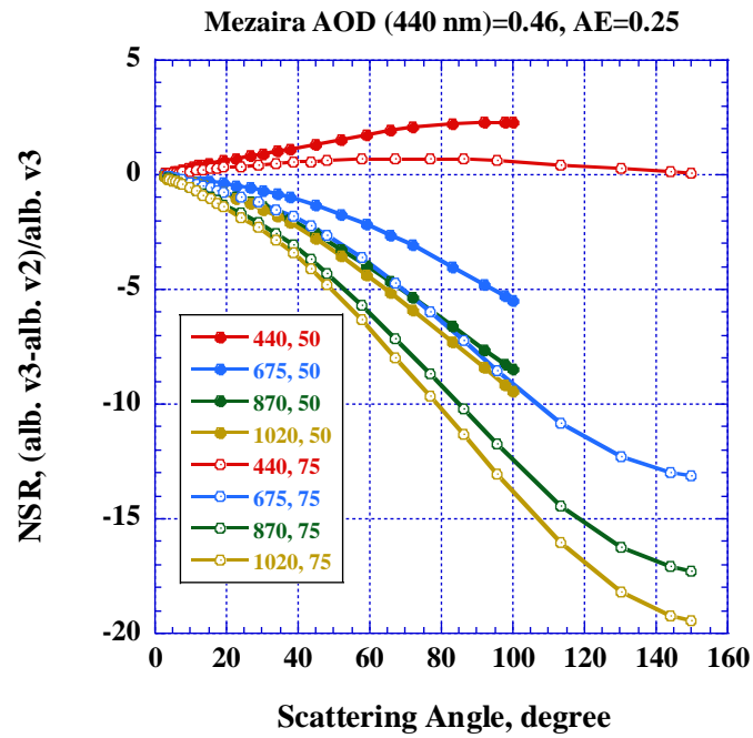
1630 Figure 3. The relative percent difference in normalized sky radiances (NSR) calculated with BRDF parameters from V2 and 1635 V3 for the Mezaira site.
