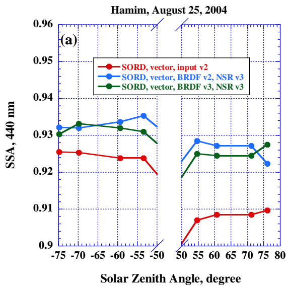
1750 Figure 9. Hamim on 25 August 2004. The diurnal variability of Level 2 SSA retrievals at 440 nm for three combinations of 1755 SORD and inversion inputs: V2 inputs (red), combined inputs with BRDF parameters of V2 and NSR of V3 (blue), and 1760 combined inputs with BRDF parameters of V3 and NSR of V3 (green) for a) 440 nm and b) 675 nm.
