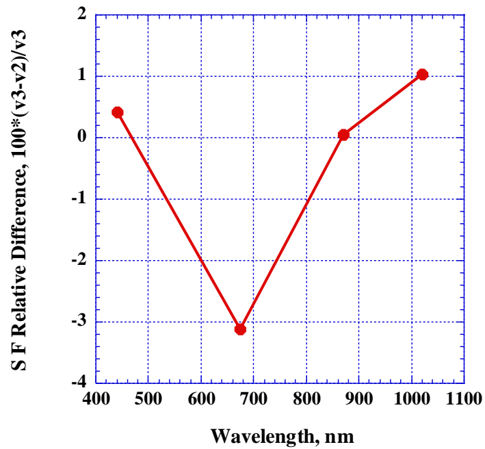
1650 Figure 4. The relative percent difference in spectral solar flux data used in V2 (ASTM E-490 https://www.nrel.gov/grid/solar-resource/spectra.html ) and V3 (Coddington et al., 2012) for four standard AERONET sky wavelengths (i. e. 440, 675, 870, and 1020 nm).
