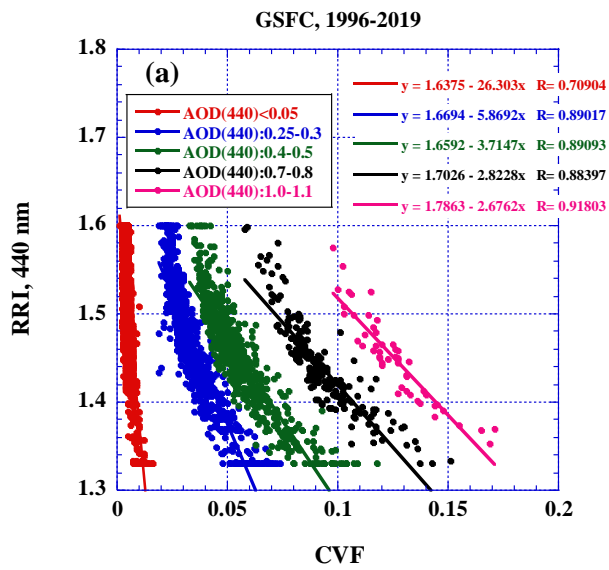
2065 Figure 25. Analysis of correlation between the real part of refractive index and fine mode concentration at GSFC site.
