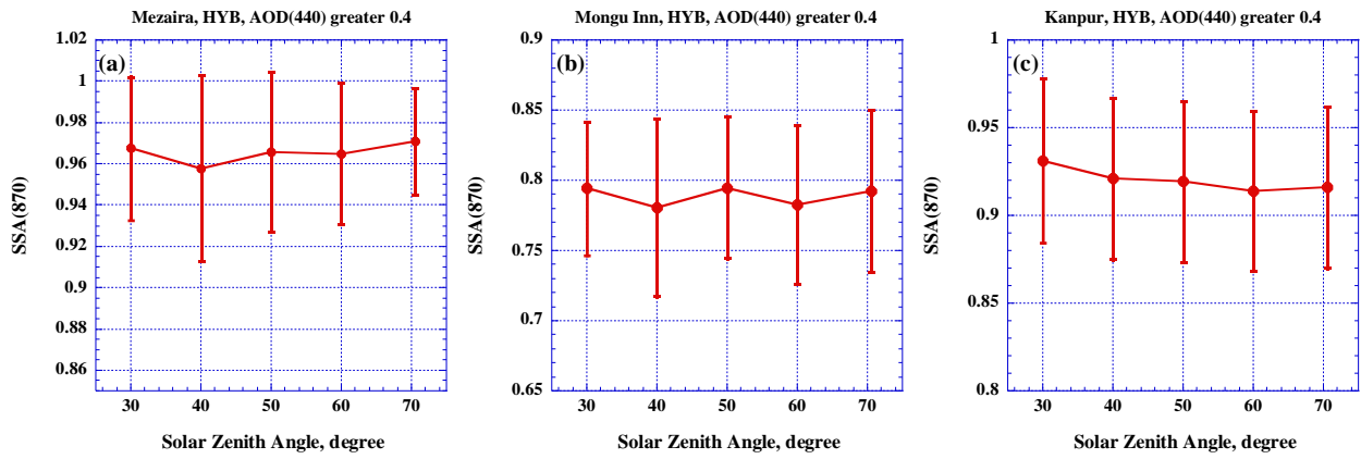
1880 Figure 15. Dependence of 870 nm SSA hybrid scan retrievals on SZA for three AERONET sites: a) Mezaira, b) Mongu Inn, 1885 c) Kanpur.
