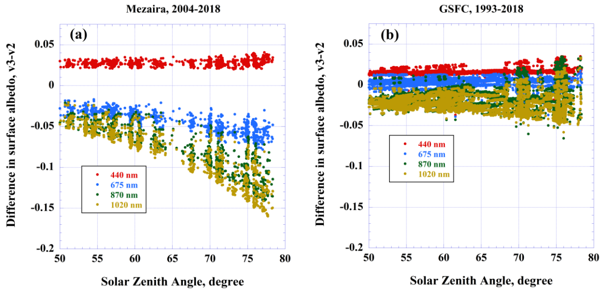
Figure 2. Difference in surface albedo calculated with BRDF from V2 and V3 for a) Mezaira (2004-2018) and b) GSFC (1993-2018).
