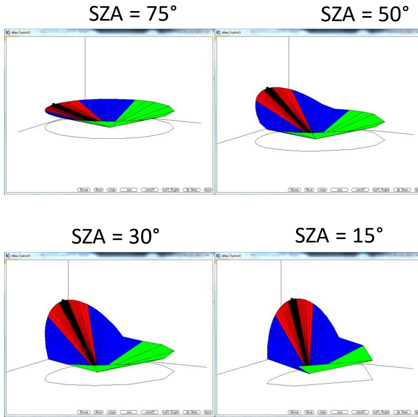
1815 Figure 12. Hybrid scan geometry depicted for four values of SZA. See explanations in text.
