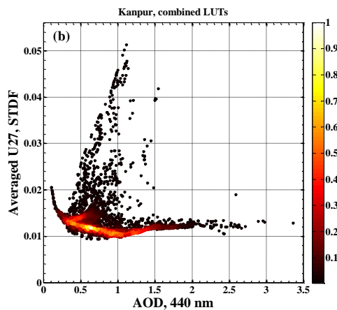
Figure 29. Uncertainties for a) volume median radius of fine mode and b) width of size distribution for fine mode estimated at Kanpur site.
