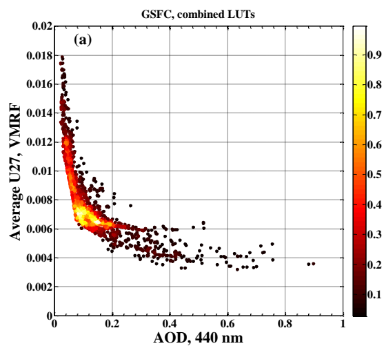
Figure 26. Uncertainties for a) volume median radius of fine mode and b) width of size distribution for fine mode estimated at GSFC site.
