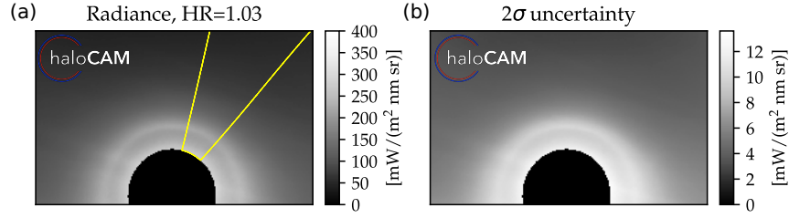
Figure 11. HaloCam RAW R-channel (a) radiance and (b) 2\sigma standard deviation from 21 April 2016, averaged over the period between 12 and 14 UTC. The 22^\circ halo ratio amounts to 1.03 and was calculated in the averaged azimuth segment, indicated here in yellow.
