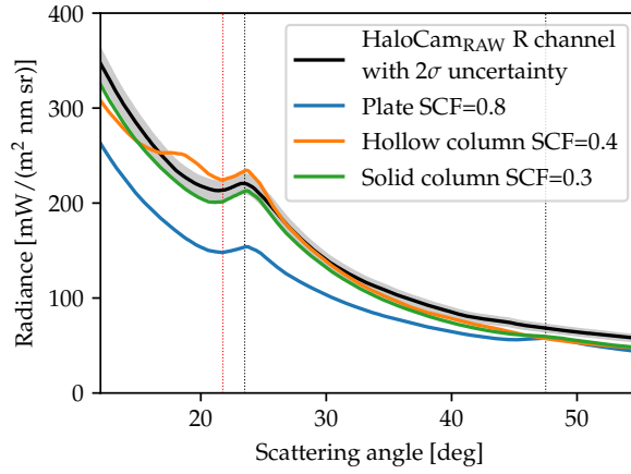
Figure 13. The black solid line displays the HaloCam RAW radiance in the principal plane above the sun from the scene shown in Fig. 11. The 2\sigma uncertainty of the HaloCam RAW radiance is represented by the gray shading around the black line. The scattering angle of the 22^\circ and 46^\circ halo peaks are indicated by the vertical black dashed lines. The red dashed line indicates the minimum of the 22^\circ halo. The 22^\circ halo ratio is computed by the ratio between the radiance values of the maximum and the minimum. The colored lines represent the radiance in the principal plane from the libRadtran simulations shown in Fig. 12 (central column) for ice crystal plates (blue), hollow columns (orange), and solid columns (green).
