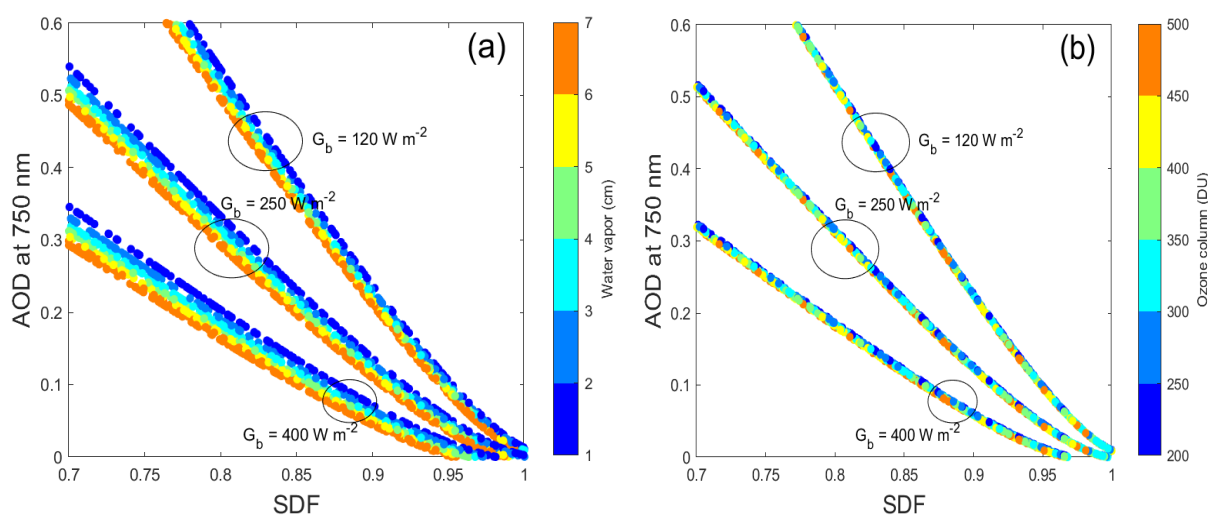
Figure 3: Same as Fig. 2 but varying (a) water vapor and (b) ozone contents.
