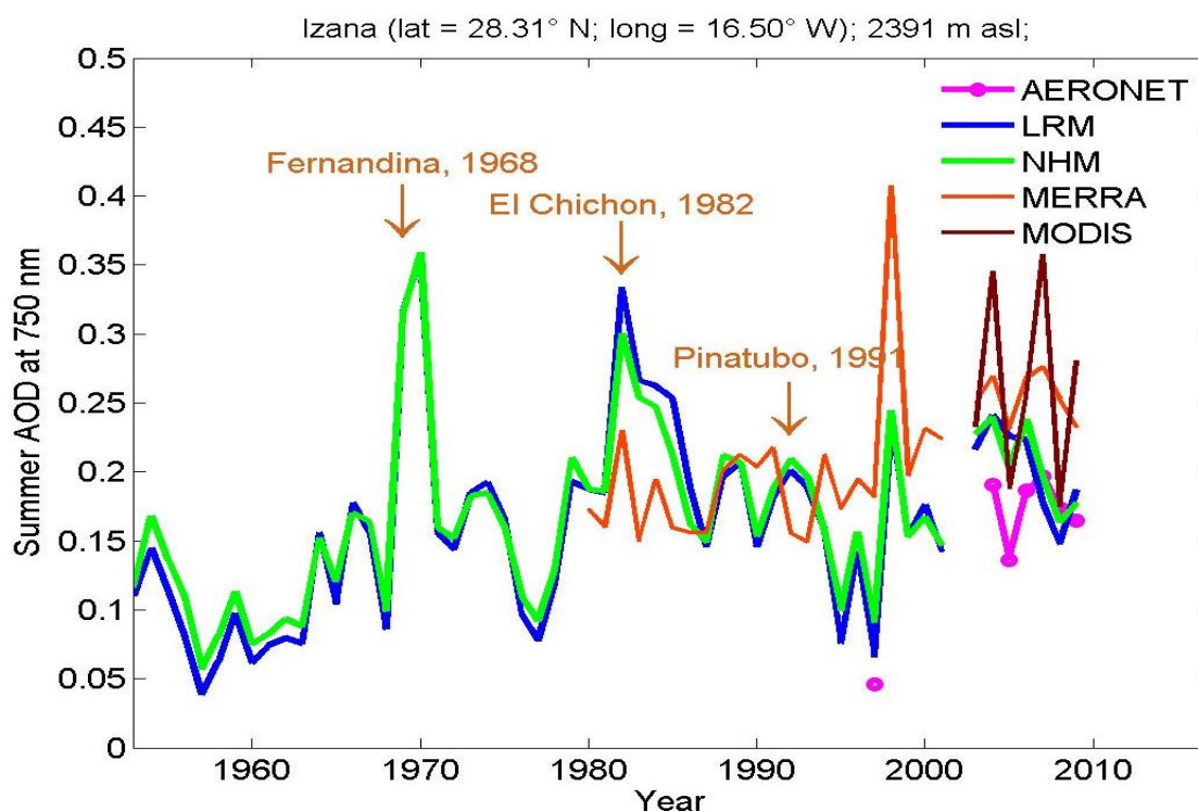
Figure 8: Time series of the summer means of AOD in Izana, Spain.
