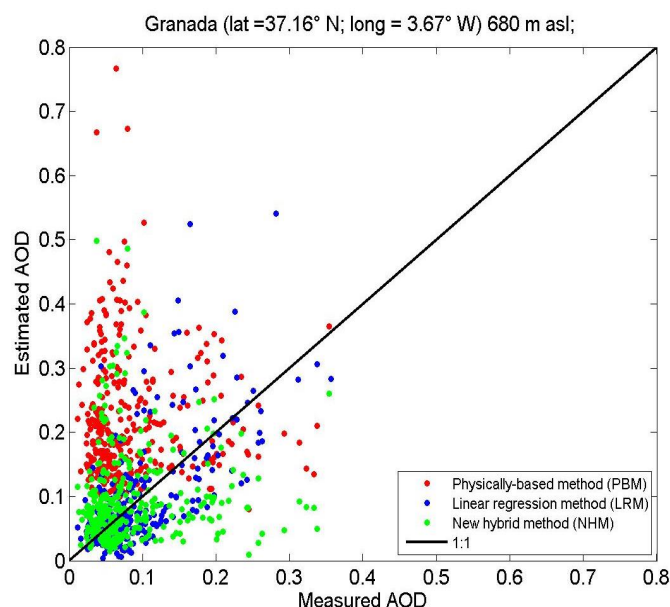
Figure 5: Scatterplot between measurements from AERONET and estimates from the PBM, LRM and NHM methods of daily AOD for Granada, Spain.
