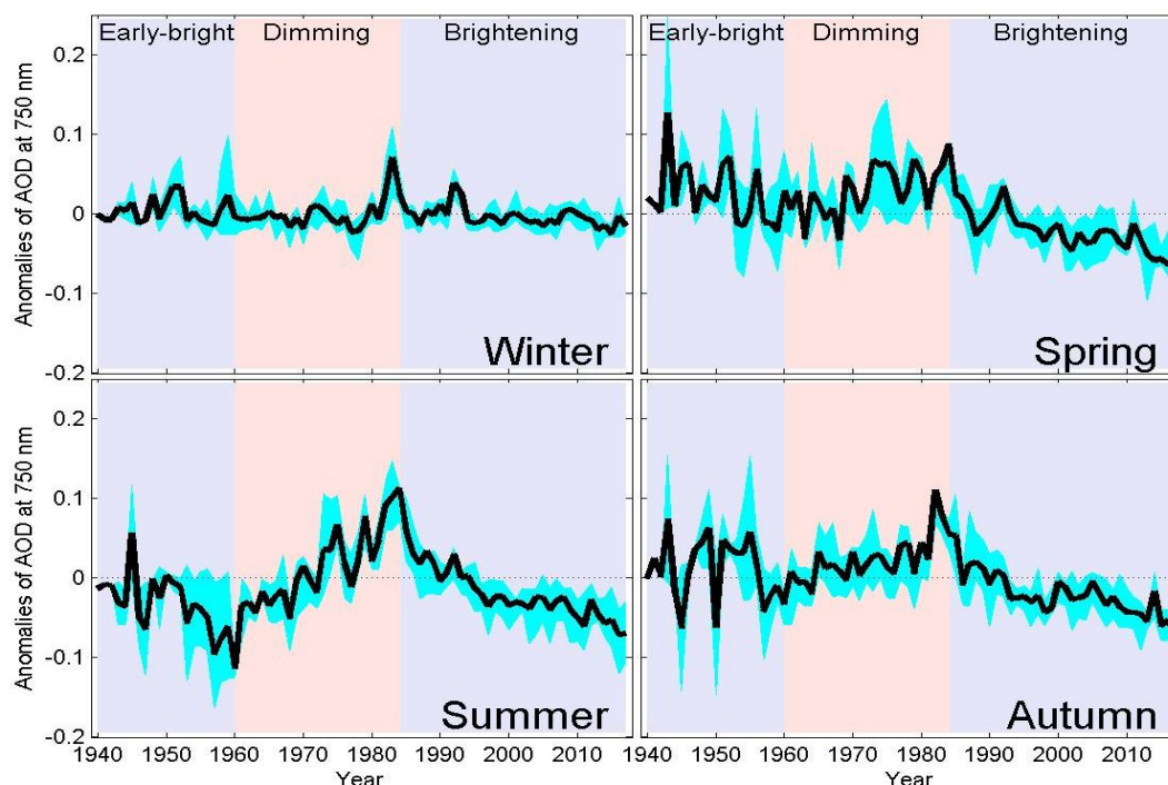
Figure 9: Evolution of the mean of seasonal anomalies of AOD for all stations given in Table 1. The cyan area refers to range between 1 st and 3 rd quartiles of the different series for each year. The light purple and misty rose bands indicate (early) brightening and dimming periods, respectively.
