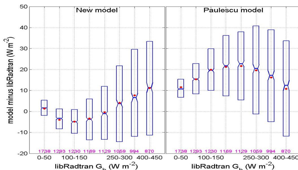
Figure 1: Dependence of deviations between estimated and libRadtran G_b for the new and Paulescu models. The red dot indicates the mean, the limits of the boxes are 1 st , 2 nd (median), 3 rd quartiles. The pink number is the number of data in a DNI range
