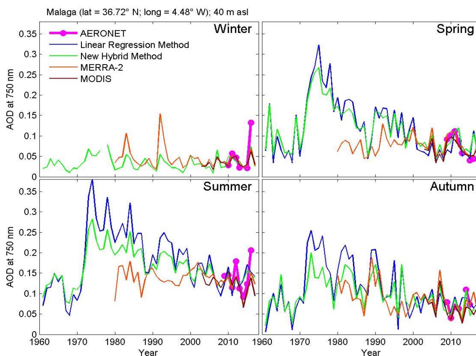
Figure 6: Time series of the seasonal mean AOD from five different data sources in Malaga, Spain.
