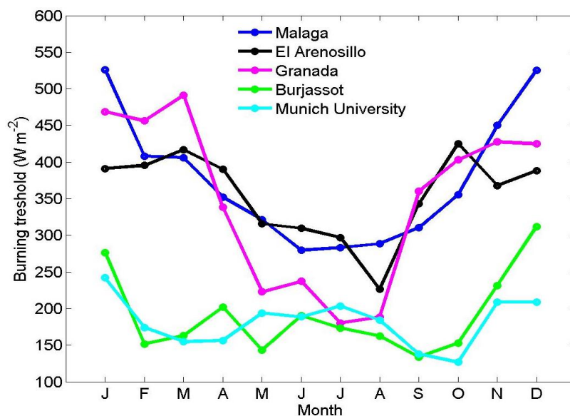
Figure 4. Monthly climatology of burning thresholds for 5 selected stations.
