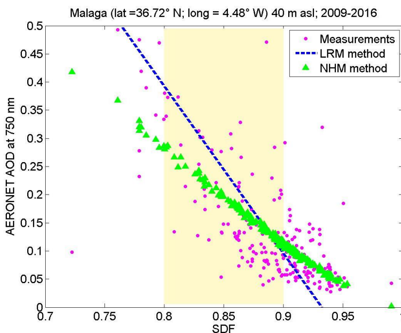
Figure 7: Scatterplot between SDF and AOD for Malaga, Spain. Regression line from LRM is in dash line. NHM estimates are in green triangle.
