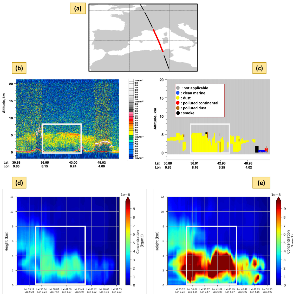
Figure 8. (a) : A measurement orbit of the CALIOP instrument during June 29, 2012 between 12:45 pm and 12:58 pm (red color corresponds to the part of the orbit which coincides with the desert dust airmass over the MB). (b) : The vertical profile of the total attenuated backscatter ( \text{km}^{-1} \text{sr}^{-1} ) as measured by CALIOP at the wavelength of 532 nm corresponding to the orbit presented in Figure 8-a. (c) : The aerosol classification corresponding to the vertical profiles showed in Figure 8-b (the majority of the aerosols are of dust origin). (d) : Vertical profiles of desert dust concentration in \text{kg m}^{-3} issued from MOCAGE model and corresponding to the CALIOP orbit of Figure 8-a issued from MOCAGE and CALIOP assimilation. (e) : Same as Figure 8-d but for the assimilation of the extinction coefficient from CALIOP lidar instrument. The white rectangle in (b), (c), (d) and (e) corresponds to the part of the orbit indicated in red color in (a).
