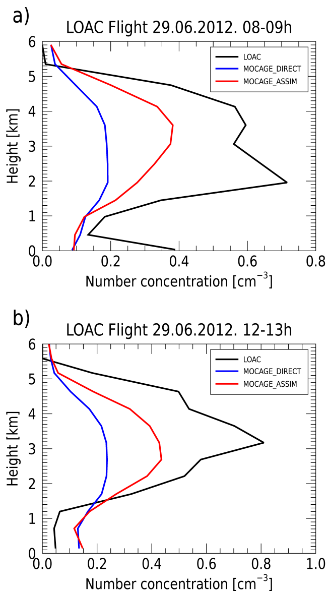
Figure 7. Vertical profile of aerosol number concentration in \text{cm}^{-3} obtained by the model free run (blue) and the CALIOP assimilation (red) both compared to the LOAC measurements (black). The comparison is done for two LOAC flights both performed on June 29, 2012: between 8 am and 9 am (a), and between 12 pm and 13 pm (b).
