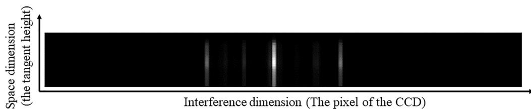
Figure 13. Graph of OH fluorescence emission radiance.
