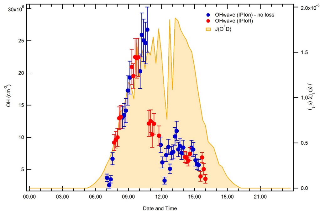
Figure 4. Time series of OH concentrations in Beijing on 17 th June 2017, a period of high OH levels in the summer 2017 AIRPRO (an integrated study of AIR pollution PROcesses in Beijing) campaign. Blue and red markers ( \pm 1\sigma ) denote observations made with and without the IPI system, respectively.
