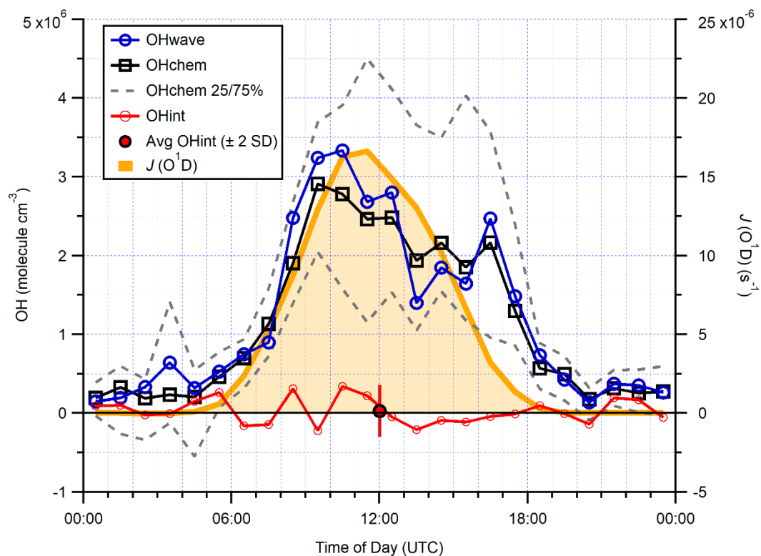
Figure 11. Hourly median diurnal profiles of OHwave, OHchem, and J(\text{O}^1\text{D}) (right axis) from the ICOZA campaign. Also shown (red line and markers) is the hourly median diurnal profile of OHint (= OHwave – OHchem), calculated from individual 4 min data points; the single red marker corresponds to the average ( \pm 2\sigma ) of this trace. The variability (interquartile range, IQR) in OHchem measurements is denoted by the grey dashed lines, not shown for others for clarity. OHwave data were corrected for the known interference from \text{O}_3 + \text{H}_2\text{O} .
