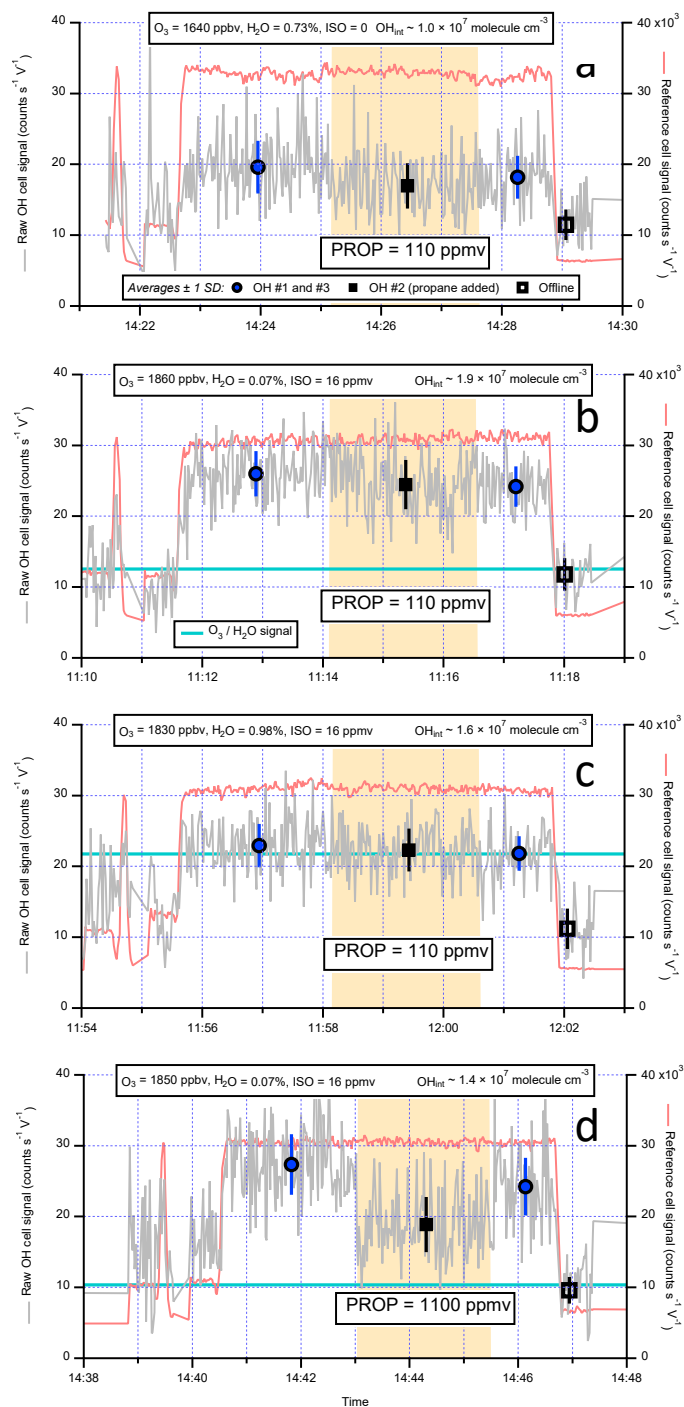
Figure 8. Isoprene (ISO) ozonolysis interference tests: (a) O_3/H_2O only, (b) O_3 and ISO under dry conditions, (c) O_3 and isoprene with H_2O added, and (d) O_3 and isoprene under dry conditions, but with a higher concentration of propane (PROP) to remove any steady-state generated OH. Shaded areas are periods of propane addition, and the light blue lines correspond to the calculated signals from O_3 + H_2O only (for experiments with isoprene present). The interference signals (“OH #2” – “offline”) were used to derive equivalent OH concentrations ( OH_{int} ), which are on the order of \sim 1\text{--}2 \times 10^7 molecule cm^{-3} . These experiments are summarised in Table 3. See text for further details.
