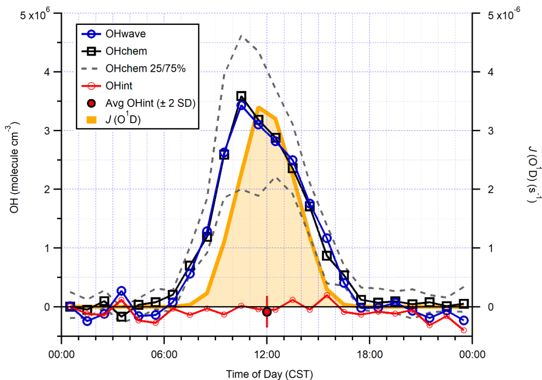
Figure 13. Hourly median diurnal profiles of OHwave, OHchem, and J(\text{O}^1\text{D}) (right axis) from the winter 2016 AIRPRO campaign. Also shown (red line and markers) is the hourly median diurnal profile of OHint, calculated from individual 4 min data points; the single red marker corresponds to the average ( \pm 2\sigma ) of this trace. The variability (IQR) in OHchem measurements is denoted by the grey dashed lines, not shown for others for clarity. OHwave data were corrected for the known interference from \text{O}_3 + \text{H}_2\text{O} .
