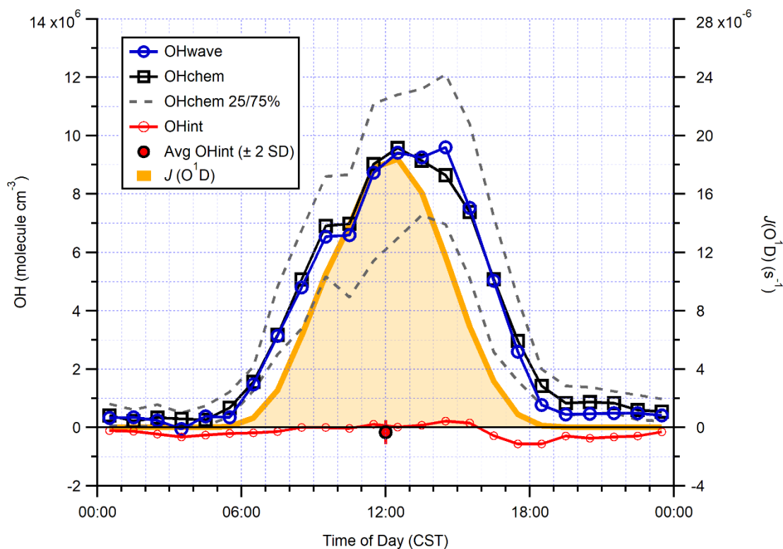
Figure 15. Hourly median diurnal profiles of OHwave, OHchem, and J(\text{O}^1\text{D}) (right axis) from the summer 2017 AIRPRO campaign. Also shown (red line and markers) is the hourly median diurnal profile of OHint, calculated from individual 4 min data points; the single red marker corresponds to the average ( \pm 2\sigma ) of this trace. The variability (IQR) in OHchem measurements is denoted by the grey dashed lines, not shown for others for clarity. OHwave data were corrected for the known interference from \text{O}_3 + \text{H}_2\text{O} .
