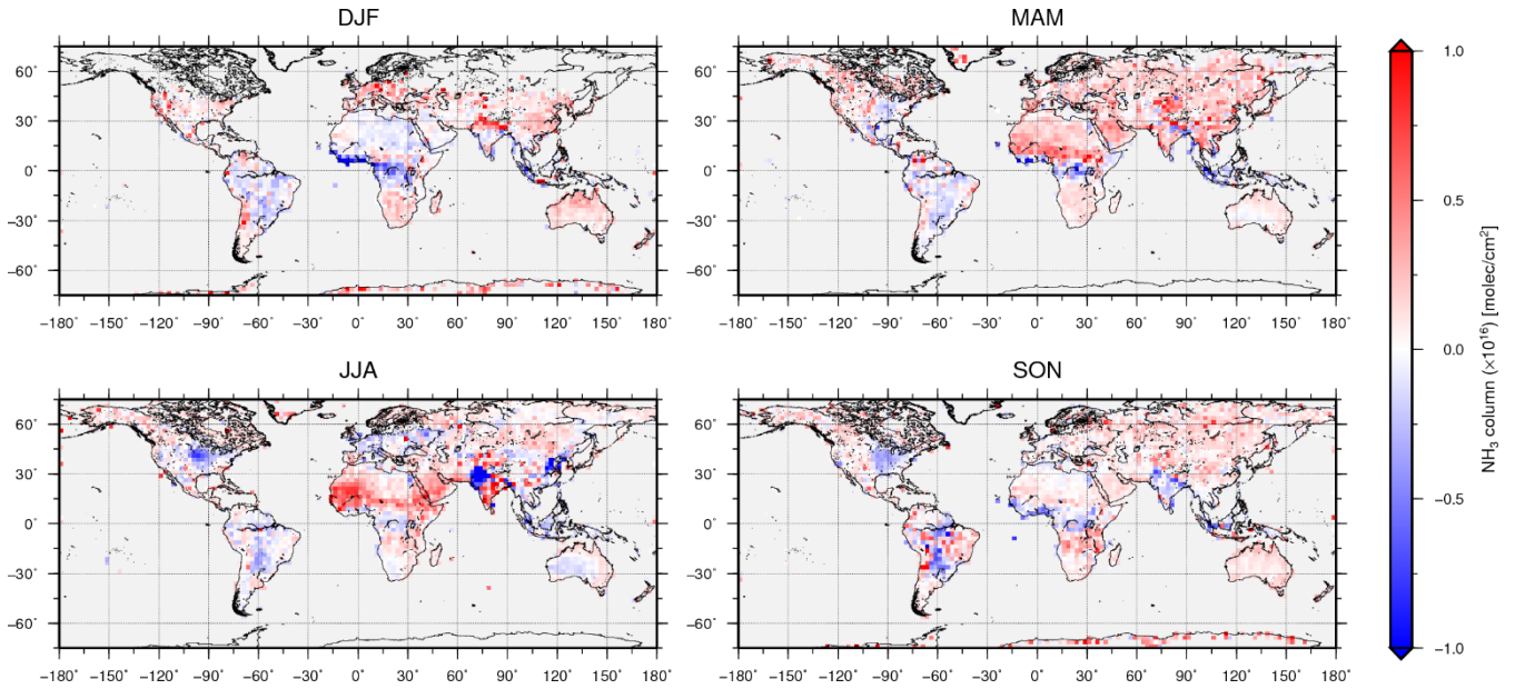
Figure 8: Same as Figure 3, but for the difference between the GOSAT and the IASI ammonia column amounts. The red color indicates that the GOSAT data are higher than that from the IASI.
