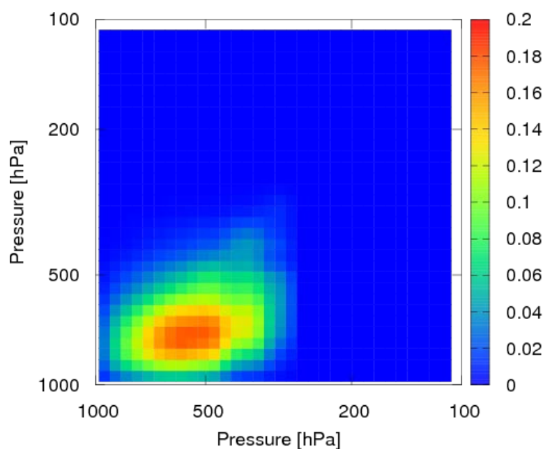
Figure S1. An example of the averaging kernel matrix for the GOSAT TIR ammonia profile retrieval using the AFGL ammonia profile and mid-latitude summer atmosphere.
