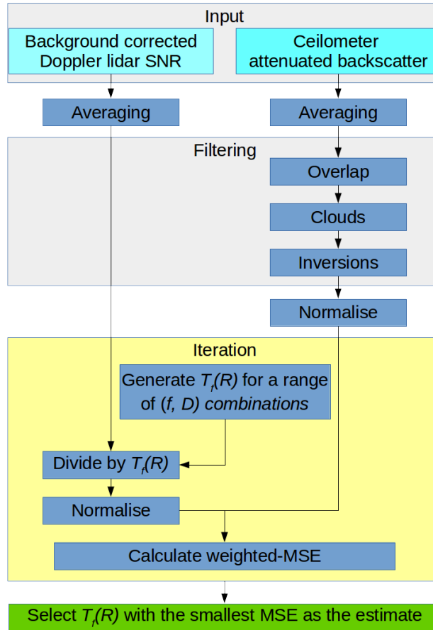
Figure 2. Process diagram of the telescope focus function parameter estimation.
