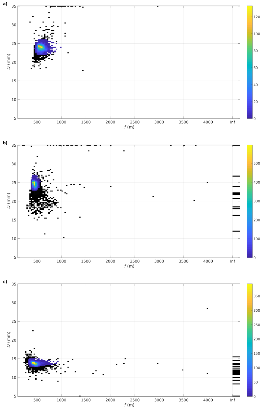
Figure 3. Distributions of T_f(R) parameter estimates from a) Darwin 21 June 2011 to 22 July 2012, b) SGP 1 January 2015 to 2 May 2016, c) SGP 3 May 2016 to 5 June 2017. Outliers filtered using \text{MAD} \geq 3 are marked in black.
