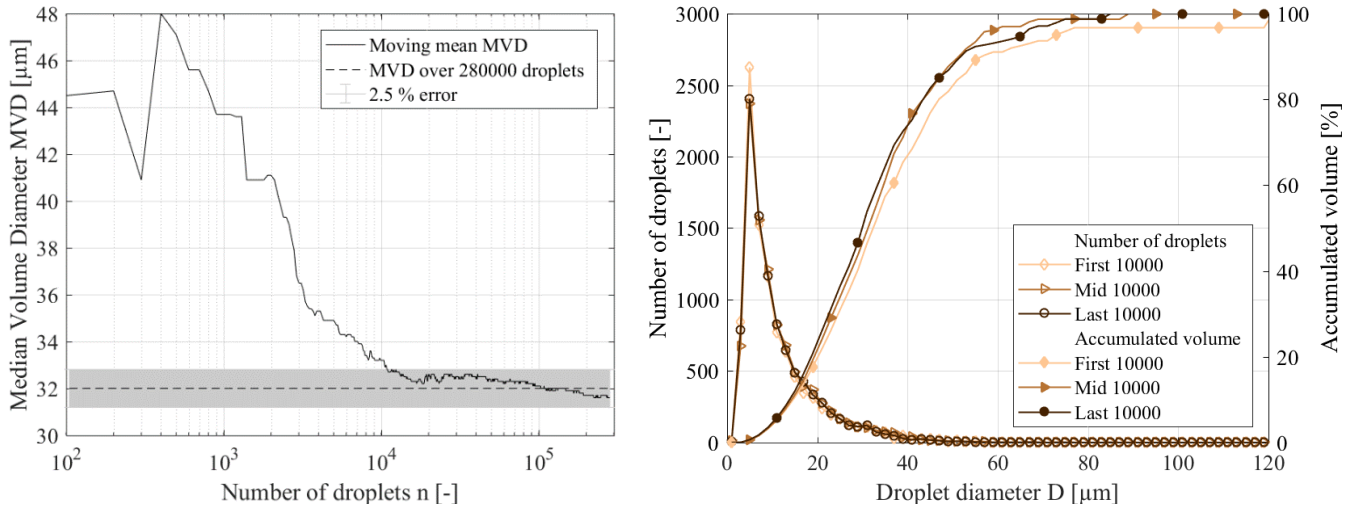
Figure 6: Convergence of MVD over number of droplets at 40 \text{ m s}^{-1} and Temporal Stability (PDI Run 09/08/17 17:59).
