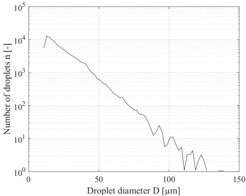
875 Figure 8: Number of droplets over diameter (PDI Run 18/04/19 18:25), total number of counts >95000.
