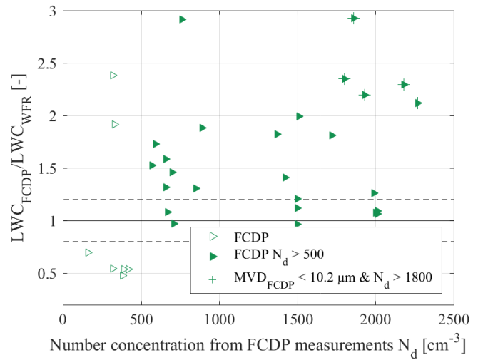
Figure 15: Effect of MVD on LWC measurements from the FCDP (left) and effect of number concentration (right).
