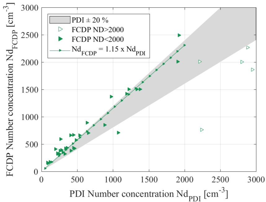
900 Figure 12: Comparison of Number Concentrations of PDI and FCDP.
