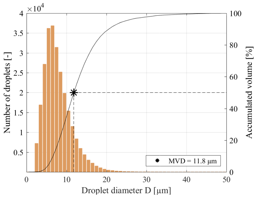
865 Figure 3: Droplet diameter histogram and cumulative volume curve at 20 \text{ m s}^{-1} (PDI Run 18/04/19 17:19).
