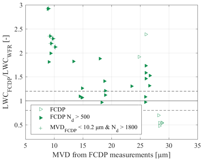
Figure 15: Effect of MVD on LWC measurements from the FCDP (left) and effect of number concentration (right).
