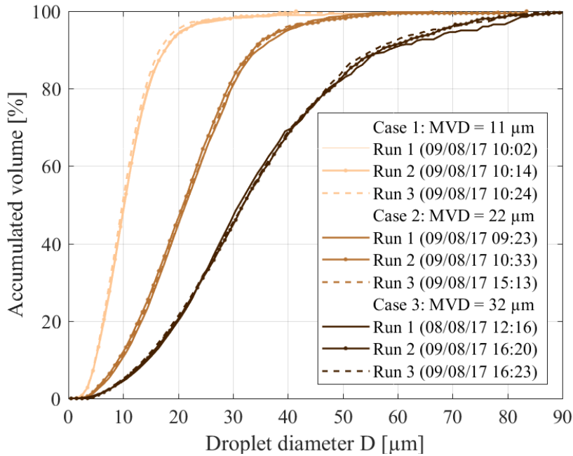
875 Figure 5: Wind tunnel repeatability shown with PDI measurements at 40 \text{ m s}^{-1} , correlation coefficients R^2 : Case 1: Run 1-2: R^2=1 ; Run 1-3: R^2=0,999 ; Run 2-3: R^2=0,999 ; Case 2: Run 1-2: R^2=0,926 ; Run 1-3: R^2=0,927 ; Run 2-3: R^2=1 ; Case 3: Run 1-2: R^2=0,999 ; Run 1-3: R^2=1 ; Run 2-3: R^2=1 .
