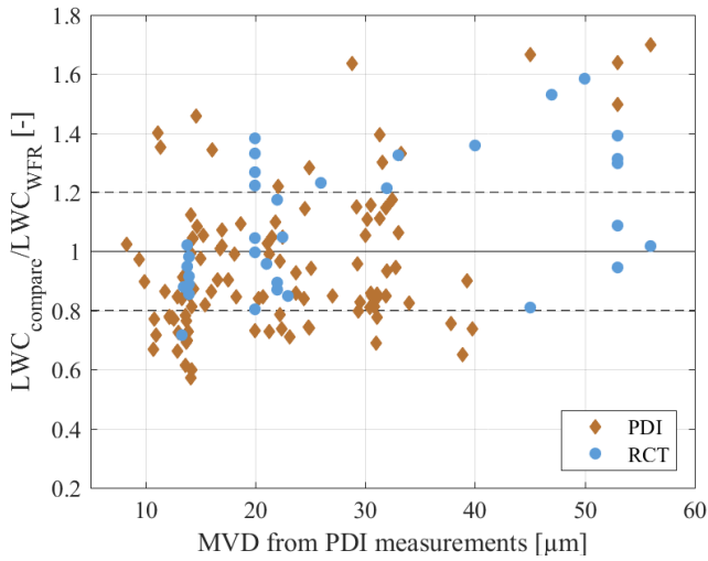
Figure 14: Effect of MVD (left) and effects of air velocity (right) on LWC measurements from the PDI and the RCT.
