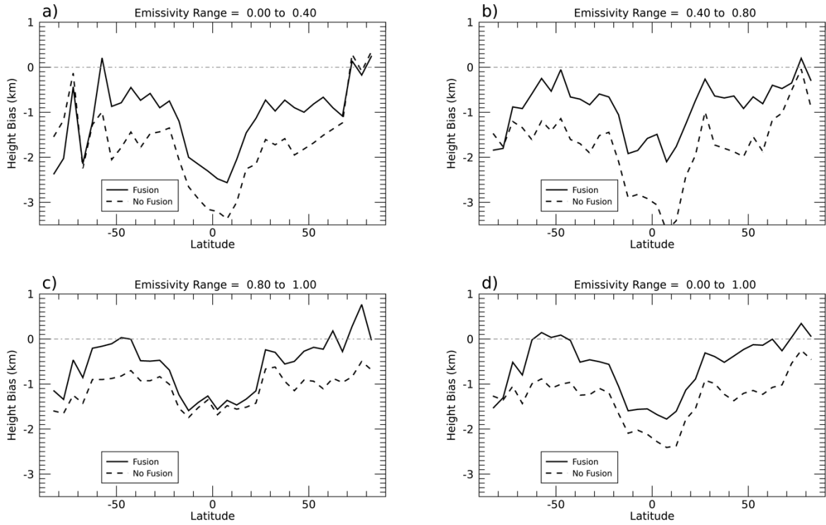
5 Figure 8. Zonal distribution of cloud height biases between S-NPP VIIRS and CALIPSO/CALIOP for emissivity range a) 0 to 0.4; b) 0.4 to 0.8; c) 0.8 to 1.0; and d) 0 to 1.0. Solid and dashed lines indicate data with/without fusion channels. Both 6.7- \mu\text{m} and 13.3- \mu\text{m} fusion channels are used for the fusion experiment.
