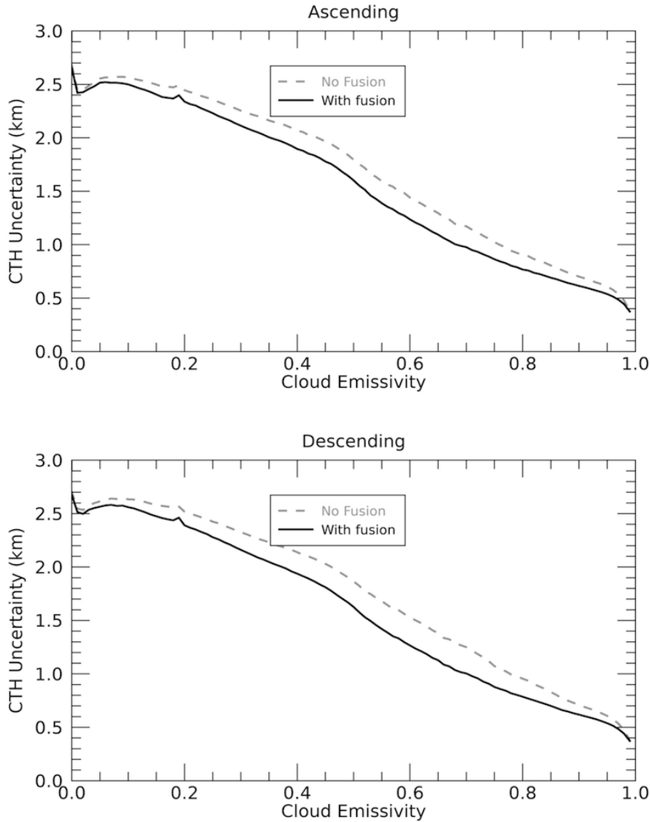
5 Figure 10. Ice cloud top height uncertainty as a function of cloud emissivity for the S-NPP VIIRS computed from two weeks of global Level 2b data in 2018.
