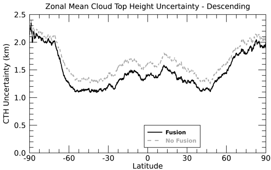
Figure 9. Zonal mean ice cloud top height uncertainty estimated from ACHA’s optimal estimation algorithm for S-NPP VIIRS computed from two weeks of global Level 2b data in 2018. The top panel shows the ascending track and the bottom panel shows the descending track.
