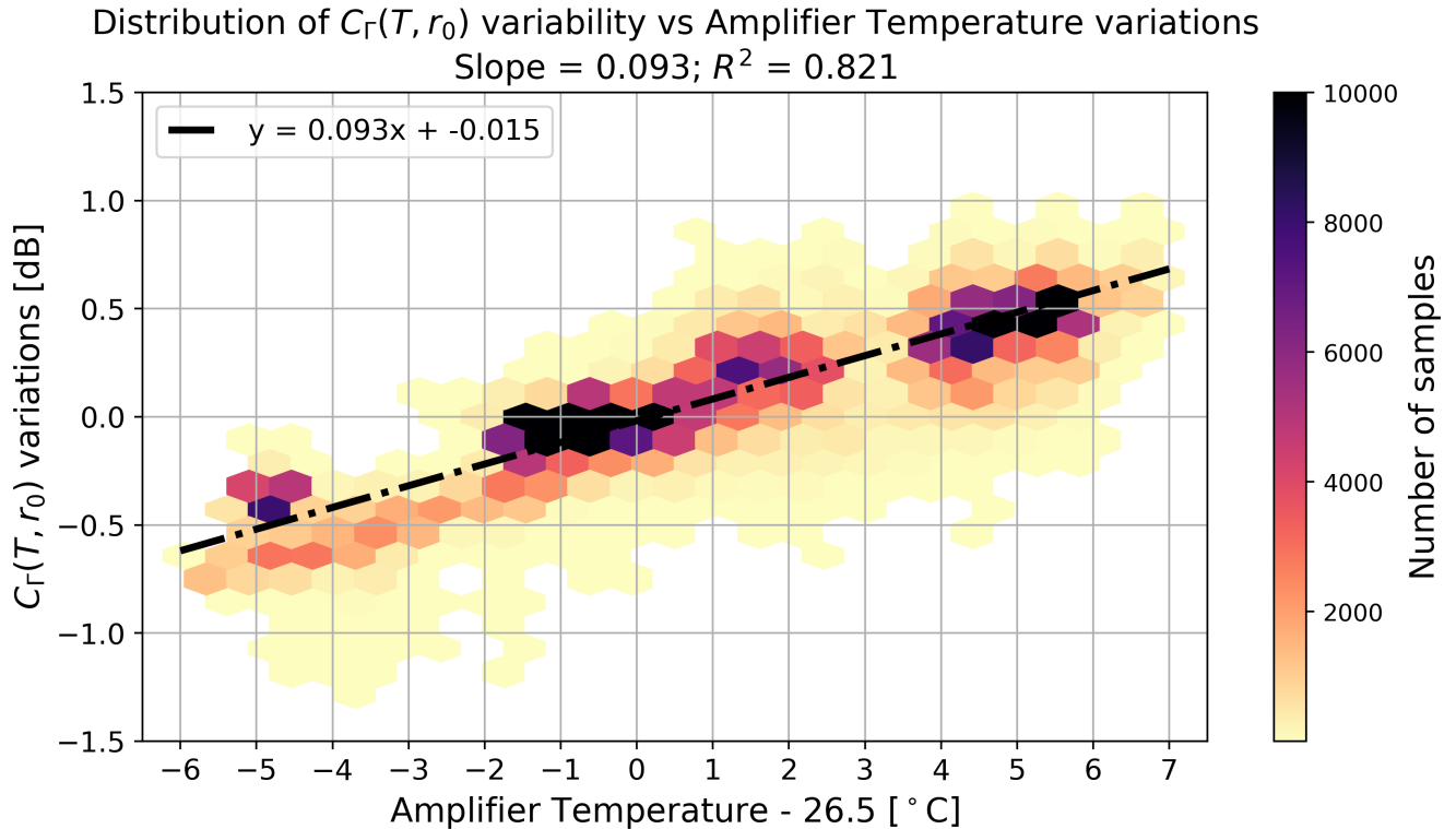
Figure 7. 2D histogram of the relative changes in C_{\Gamma}(T, r_0) with respect to changes in the amplifier temperature and its linear least squares fit. The histogram is plotted using all C_{\Gamma}(T, r_0) samples from 2018 and 2019 calibration campaigns.
