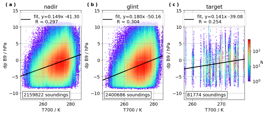
Figure 13. Correlations and linear regressions for the difference between retrieved and a priori surface pressure from GEOS5-FP-IT ( dp ) as a function of temperature at 700 hPa ( T_{700} ) for all retrievals over land north of 50^\circ\text{N} that pass Boreal QC, separated by viewing geometry.
