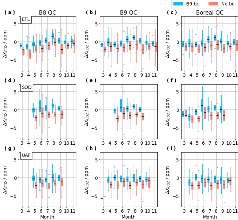
Figure 11. Box-plots of distributions of monthly biases for each Boreal Forest site and for each QC, showing results with and without the standard B9 bias correction. Box-plots show the median in the center of the box, the first and third quartile as the bottom and top of the box and the full range of data values as the bars extending above and below the box. Note that bias is defined as (\Delta X_{CO_2} \equiv (\text{OCO-2 retrieval})_i - (\tilde{X}_{\text{NNG}})_i) for each coincident OCO-2 sounding.
