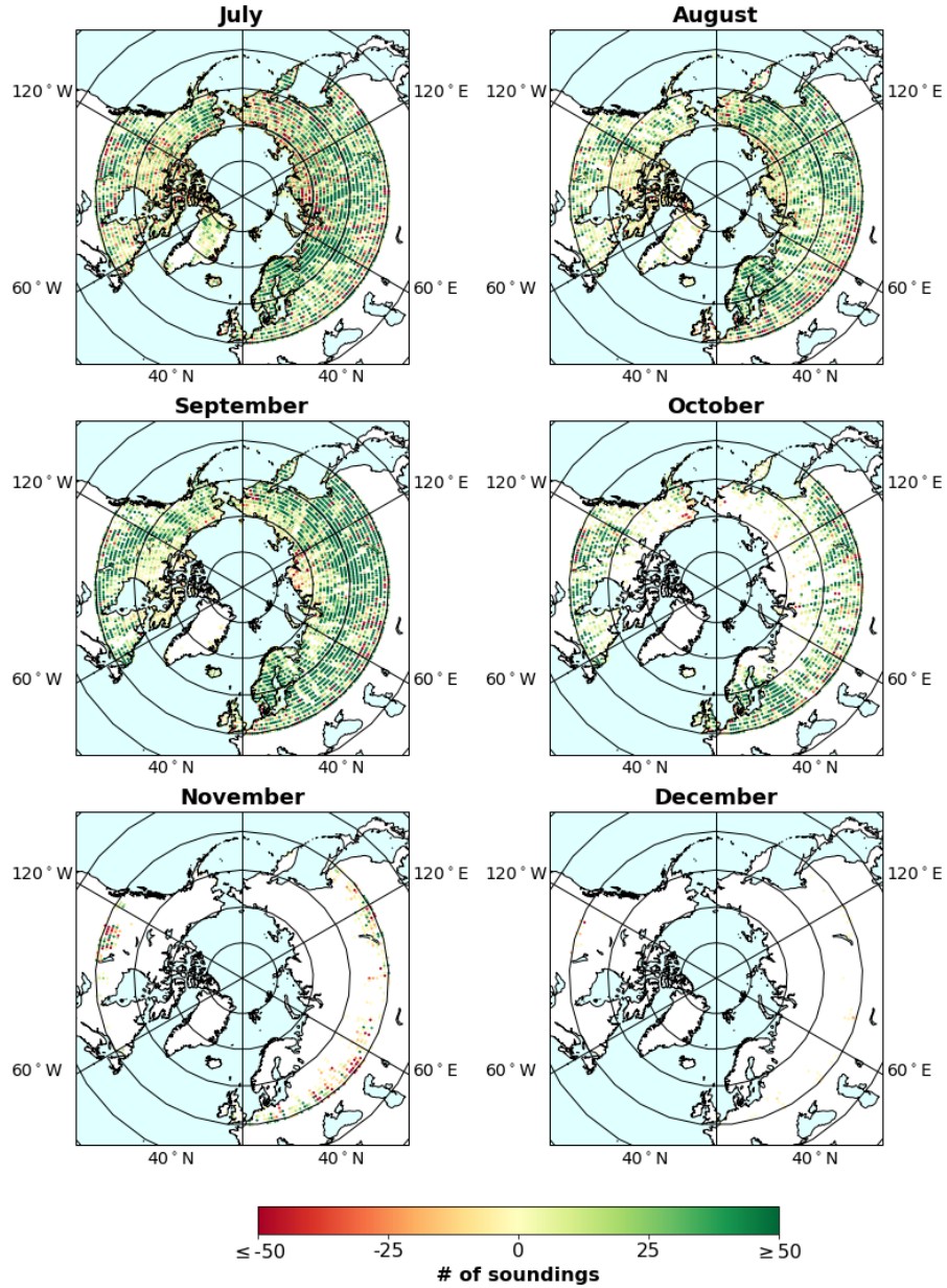
Figure 6. Maps of differences between the number of soundings passed by Boreal QC and the number of soundings passed by B9 QC in each 1^\circ latitude by 1^\circ longitude grid cell in each month (July to December, and summing all years 2014 to 2018).
