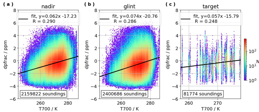
Figure 12. Correlations and linear regressions for dp_{frac} (defined in supplemental materials or by Kiel et al. (2019)) as a function of temperature at 700 hPa ( T_{700} ) for all retrievals over land north of 50^\circ\text{N} that pass Boreal QC, separated by viewing geometry.
