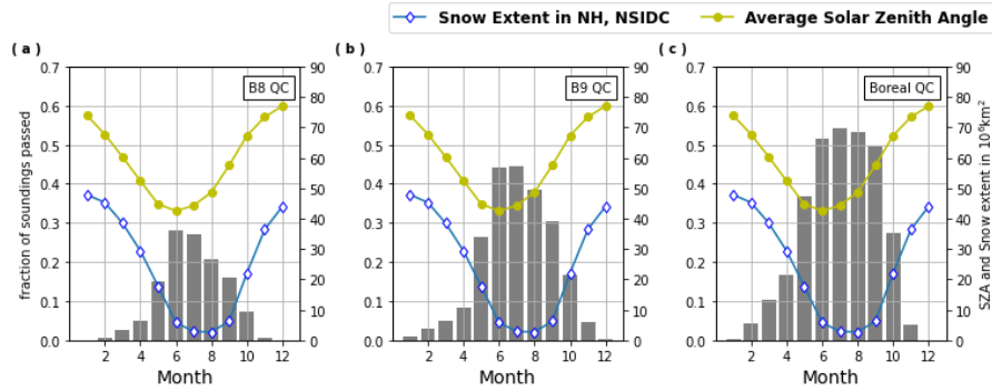
Figure 7. The fraction of soundings that pass each set of QC filters for each month out of all land soundings north of 50°N in the OCO-2 Lite files (note that OCO-2 observations are filtered by a preliminary cloud screening before being compiled in the Lite files). Also plotted are the average sza reported in OCO-2 retrievals that pass in each month and the monthly snow extent in the Northern Hemisphere averaged over 2014-2018 as reported in the NOAA database (Robinson et al., 2012).
