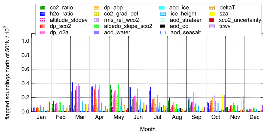
Figure 4. Total number of land soundings north of 50°N flagged by Boreal quality filters in each month.
