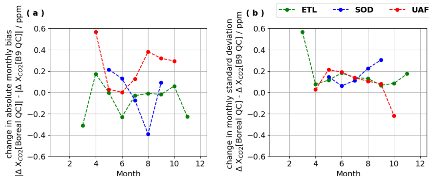
Figure 18. Differences between average monthly biases (left) or standard deviation in monthly biases (right) when comparing Boreal QC to B9 QC. Note that Fig. 10 shows typical average monthly bias ranges from -1 ppm to 1 ppm.
