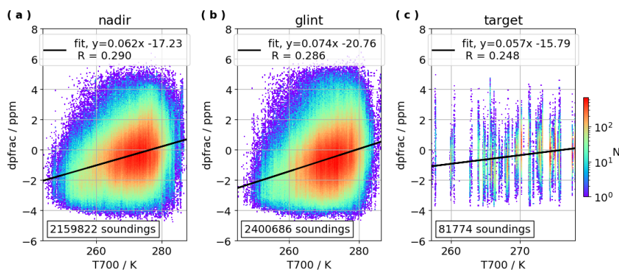
Figure 13. Correlations and linear regressions for dpfrac (defined in supplemental materials or by Kiel et al. (2019)) as a function of temperature at 700 hPa (T700) for all retrievals over land north of 50°N that pass Borealis QC, separated by viewing geometry.
