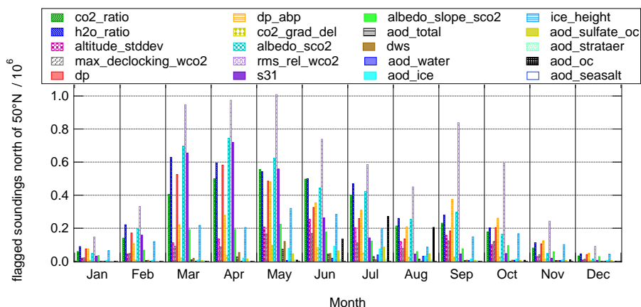
Figure 2. Total number of land soundings north of 50°N flagged by B8 quality filters in each month.
