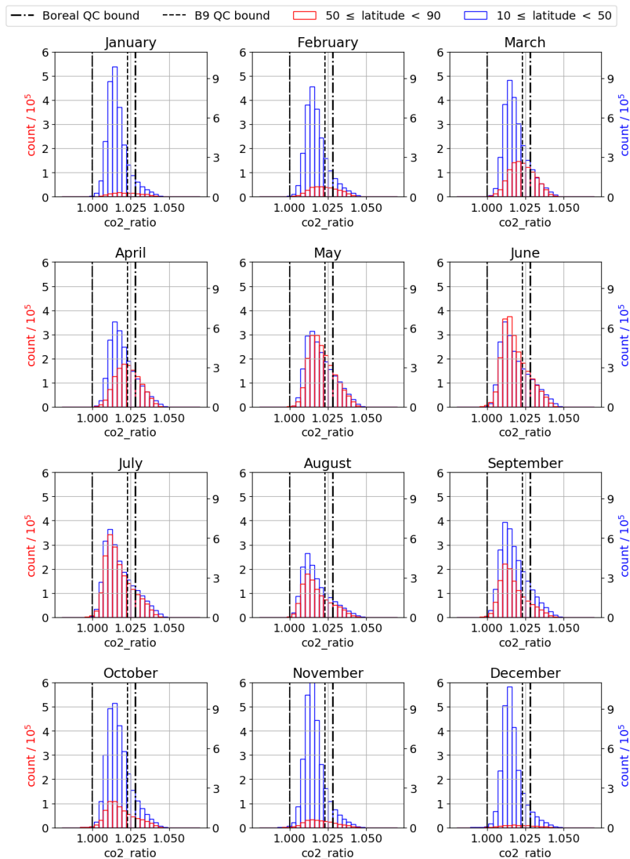
Figure 21. Monthly histograms of the ratio in single band retrievals of CO 2 (co2_ratio) for all unfiltered OCO-2 retrievals over land (land_fraction=100) split into two latitude bands, 10°N to 50°N and 50°N to 90°N.
