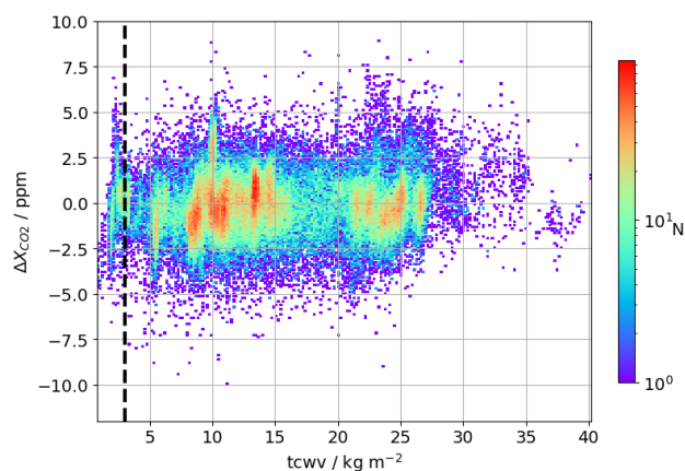
Figure 24. Bias in coincident retrievals of X_{CO_2} ( \Delta X_{CO_2} \equiv \text{OCO-2} - \text{NNG} ) with all Boreal QC filtering except the bound on total column water vapor (tcwv) against retrieved tcwv, plotted as a density map. The lower bound placed on tcwv in the Boreal QC ( 3 \text{ kg m}^{-2} ) is shown as a black, dashed vertical line.
