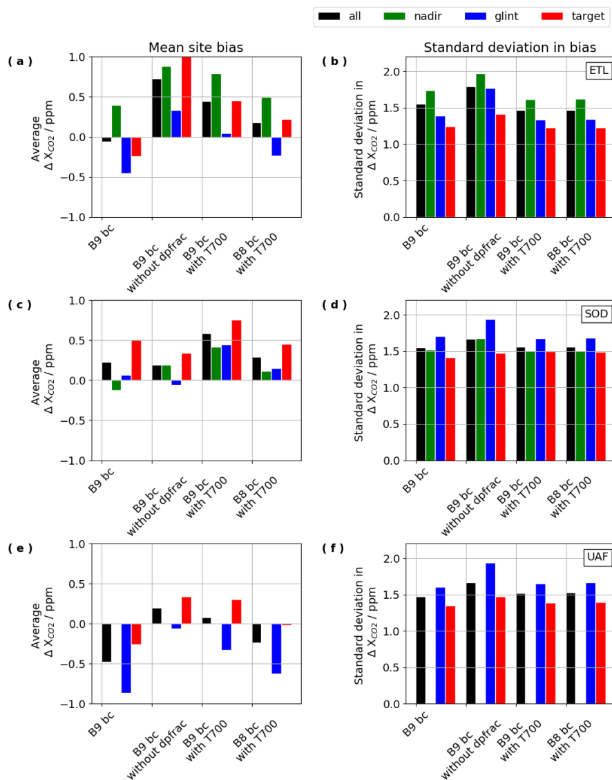
Figure 17. Average bias and standard deviation in bias, sorted by viewing geometry and bias correction modification for all coincident soundings at each of the three Boreal forest sites with Boreal QC. Note that there are no coincident nadir soundings for Fairbanks due to the satellites operational design, which favors glint observations in orbits primarily over oceans.
