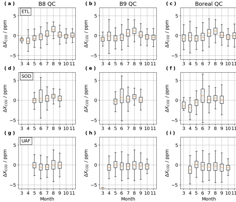
Figure 11. Box-plots of distributions of monthly biases for each Boreal Forest site and for each QC. Box-plots show the median in the center of the box, the first and third quartile as the bottom and top of the box and the full range of data values as the bars extending above and below the box. Note that bias is defined as (\Delta X_{CO_2} \equiv (\text{OCO-2 retrieval})_i - (\tilde{X}_{\text{NNG}})_i) for each coincident OCO-2 sounding.
