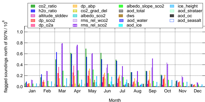
Figure 3. Total number of land soundings north of 50°N flagged by B9 quality filters in each month.
