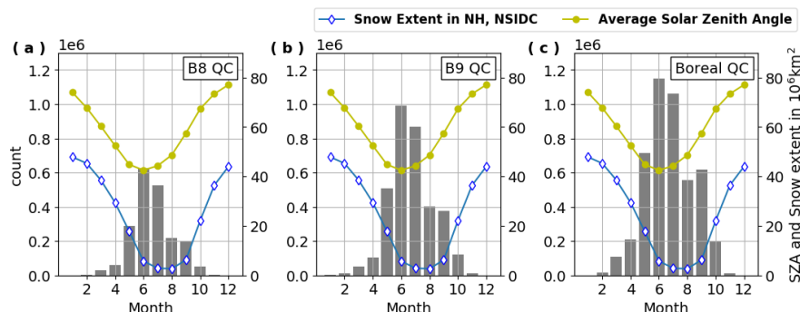
Figure 7. Total number of land soundings north of 50°N that pass QC filters in each month, plotted along with the average sza reported in OCO-2 retrievals that pass in each month and the monthly snow extent in the Northern Hemisphere averaged over 2014–2018 as reported in the NOAA database (Robinson et al., 2012).
