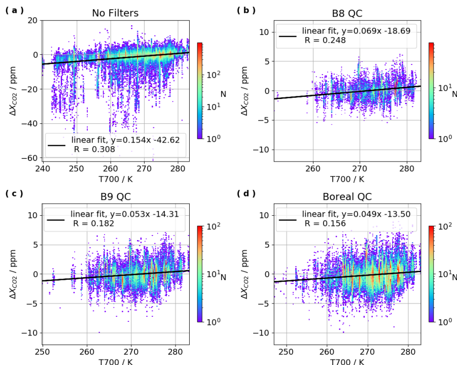
Figure 27. Bias in coincident retrievals of X_{CO_2} ( \Delta X_{CO_2} \equiv \text{OCO-2} - \text{NNG} ) as a function of mid-tropospheric temperature ( T_{700} \equiv temperature at 700 hPa) for all data without QC filters, and each of the three QC methods presented in this paper.
