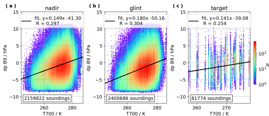
Figure 14. Correlations and linear regressions for the difference between retrieved and a priori surface pressure from GEOS5-FP-IT ( dp ) as a function of temperature at 700 hPa ( T700 ) for all retrievals over land north of 50^\circ\text{N} that pass Boreal QC, separated by viewing geometry.
