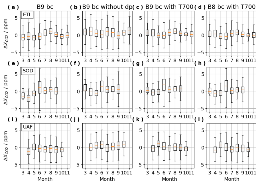
Figure 15. Box-plots of distributions of monthly biases at each Boreal Forest site, and filtered by Boreal QC, given the standard B9 bc (Eq. 4), given the B9 bc without the dp term, given the B9 abc (Eq. 6), or given the B8 abc (Eq. 8). Note that bias is defined as (\Delta X_{CO_2} \equiv (\text{OCO-2 retrieval})_i - (\tilde{X}_{\text{NNG}})_i) for each coincident OCO-2 sounding.
