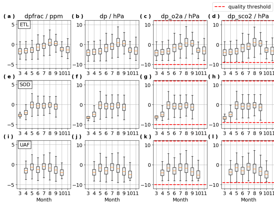
Figure 28. Seasonal box-plots of dp_{frac} , dp , dp_{o2a} , and dp_{sco2} at (top) East Trout Lake, (center) Sodankylä, and (bottom) Fairbanks given Boreal QC filters.
