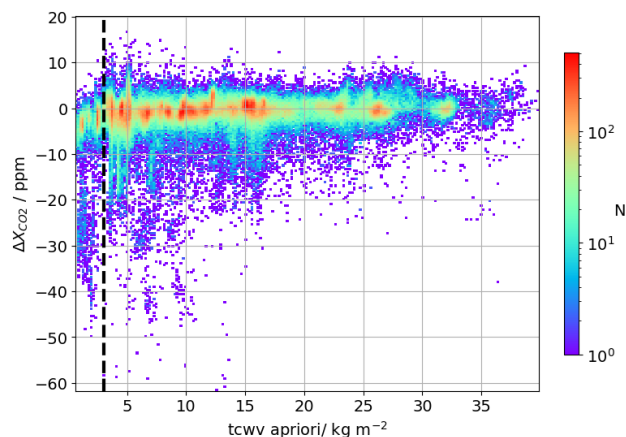
Figure 25. Bias in coincident retrievals of X_{CO_2} ( \Delta X_{CO_2} \equiv \text{OCO-2} - \text{NNG} ) with no QC filtering against a priori tcwv (total column water vapor), plotted as a density map. A priori tcwv is defined by ECMWF reanalysis data. The lower bound placed on tcwv in the Boreal QC ( 3 \text{ kg m}^{-2} ) is shown as a black, dashed vertical line.
