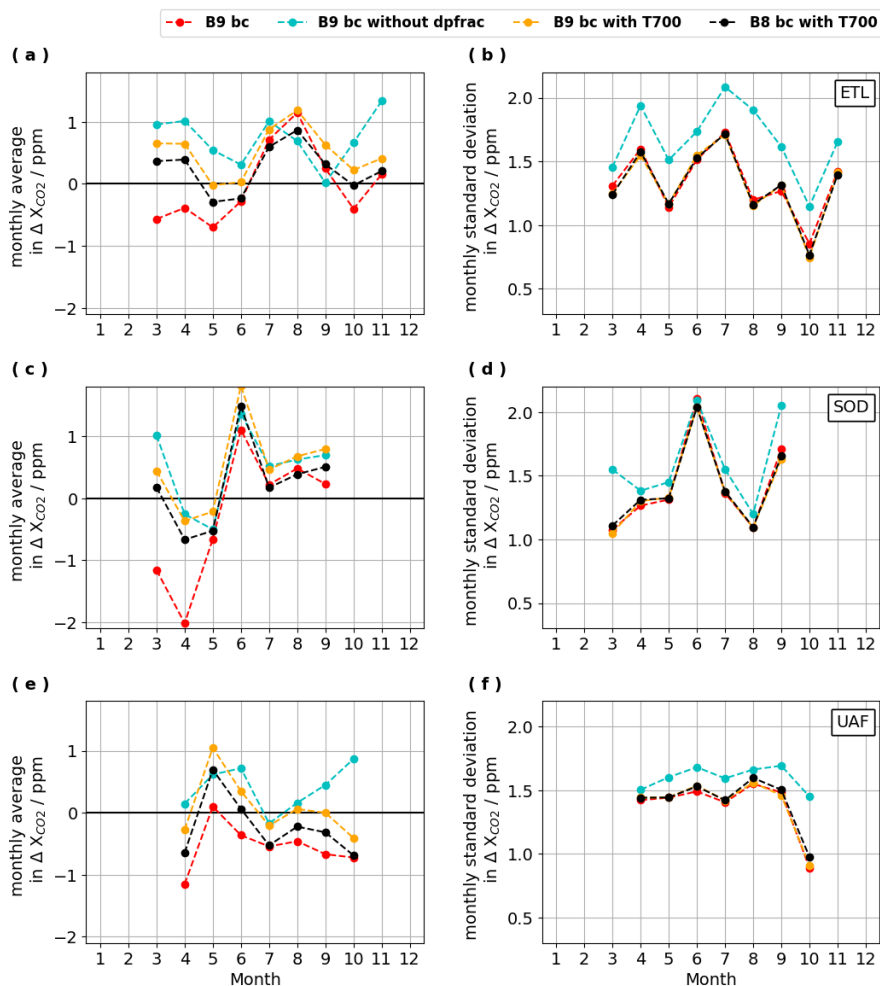
Figure 16. Monthly average bias (left) and standard deviation in biases (right) of coincident OCO-2 soundings at each of the three Boreal Forest sites with Boreal QC filtering and given each bias correction modification: the standard B9 bc (Eq. 4), the B9 bc without the dpfrac term, B9 abc with a term for temperature at 700hPa (T700; Eq. 6), and B8 bc with a term for T700 (Eq. 8).
