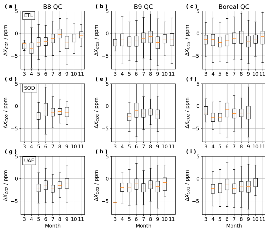
Figure 12. Box-plots of distributions of monthly biases for each Borealis site and for each QC, without the OCO-2 bias correction. Note shift in y-axis scaling relative to Fig. 11.
