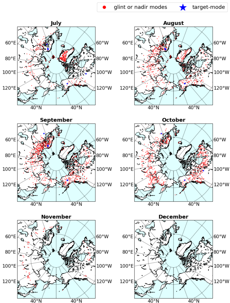
Figure 6. Maps of additional data coverage gained in each month (July to December, 2014 to 2018) from applying Boreal QC instead of B9 QC, with 1^\circ resolution.
