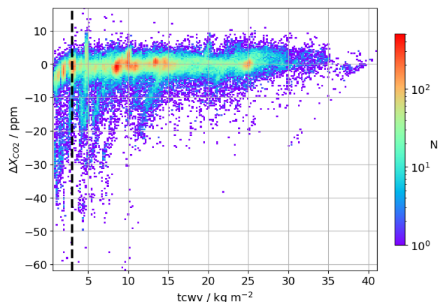
Figure 23. Bias in coincident retrievals of X_{CO_2} ( \Delta X_{CO_2} \equiv \text{OCO-2} - \text{NNG} ) with no QC filtering against retrieved tcwv (total column water vapor), plotted as a density map. The lower bound placed on tcwv in the Boreal QC ( 3 \text{ kg m}^{-2} ) is shown as a black, dashed vertical line.
