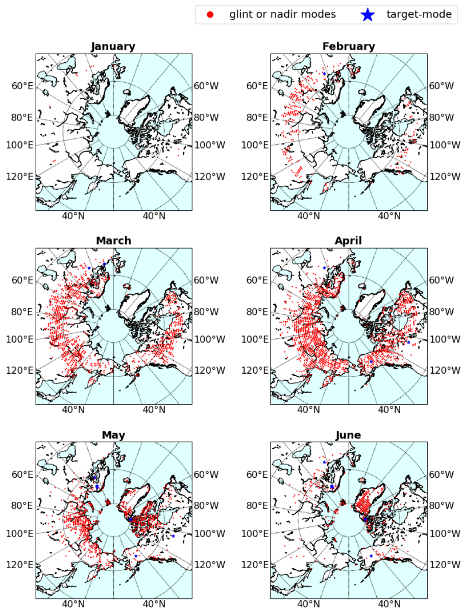
Figure 5. Maps of additional data coverage gained in each month (January to June, 2014 to 2018) from applying Boreal QC instead of B9 QC, with 1^\circ resolution.
