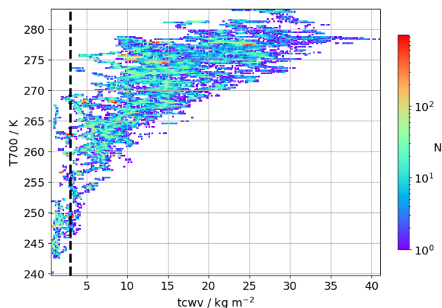
Figure 26. Mid-tropospheric temperature ( T_{700} \equiv temperature at 700 hPa) as a function of total column water vapor (tcwv) for all coincident retrievals without QC filters.
