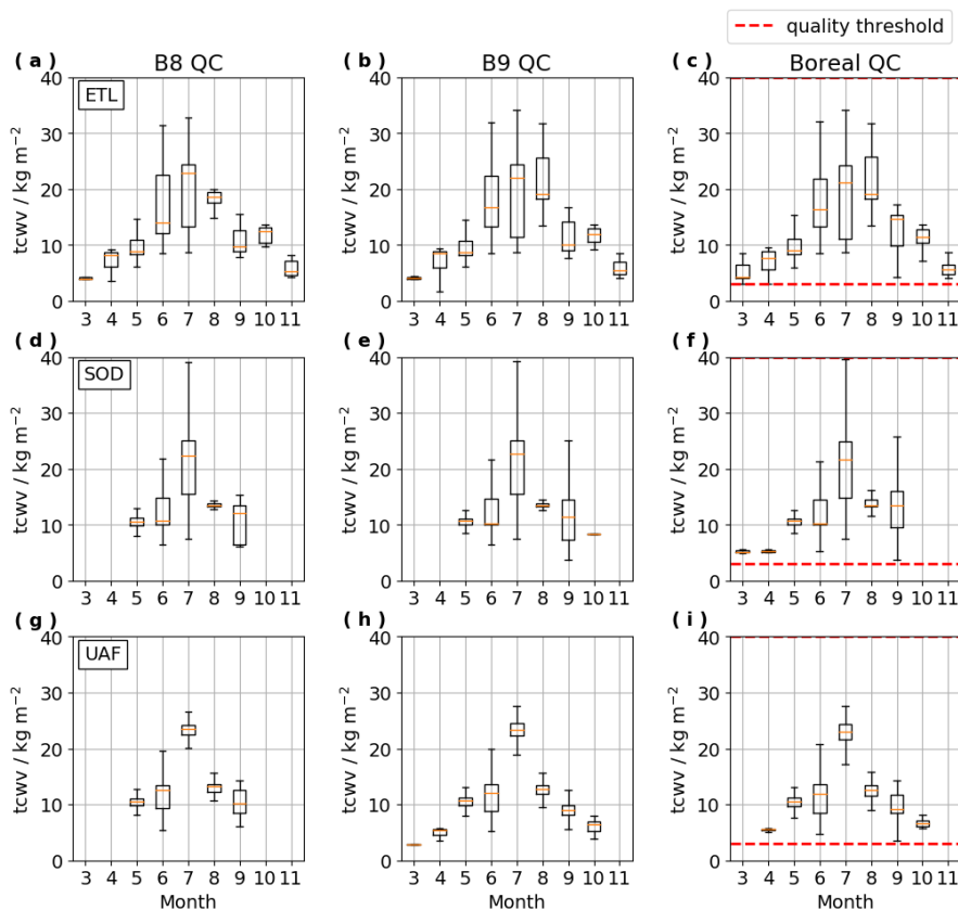
Figure 22. Seasonal box-plots of retrieved tcwv (total column water vapor) at (top) East Trout Lake, (center) Sodankylä, and (bottom) Fairbanks given each of the three quality control methods.
