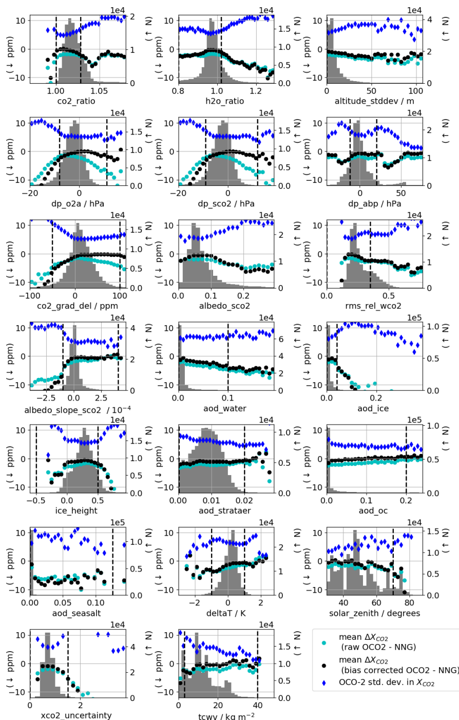
Figure A1. Quality control histograms in the same style as those presented by O'Dell et al. (2018), presented for QC parameters used in the selection of Boreal QC and considering only retrievals coincident to the Boreal Forest sites in this paper. Also shown are biases in X_{CO_2} with raw OCO-2 retrieved X_{CO_2} , biases in X_{CO_2} with OCO-2 retrieved X_{CO_2} bias corrected to TCCON, standard deviation in OCO-2 retrieved X_{CO_2} with the bias correction to TCCON and the quality control thresholds selected in the Boreal QC.
