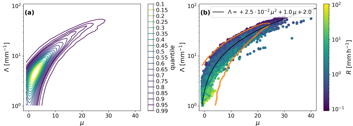
Figure 4. a) Density plot of gamma DSD parameters retrieved with the TS96 method, where density contours are given as quantiles enclosed within the contour. Results are for the complete 9-month set of path-averaged disdrometer data. b) Polynomial fit of the \Lambda and \mu parameters in the gamma distribution function fitted to parameter values obtained from the TS96 method of moments, based on the 9 months of path-averaged disdrometer data from Wageningen. The colors indicate the corresponding rain intensities. The 0.95 quantile contour that is used as a masked is overlaid in orange.
