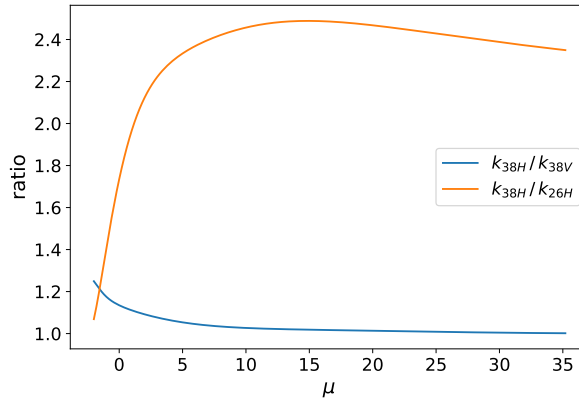
Figure 5. Ratios of attenuations as a function of the \mu parameter for the two-parameter retrieval method. the blue lines indicates the attenuation ratio for the dual-polarization method (38 GHz) and the orange line indicates the attenuation ratio of the dual-frequency method (38 GHz and 26 GHz).
