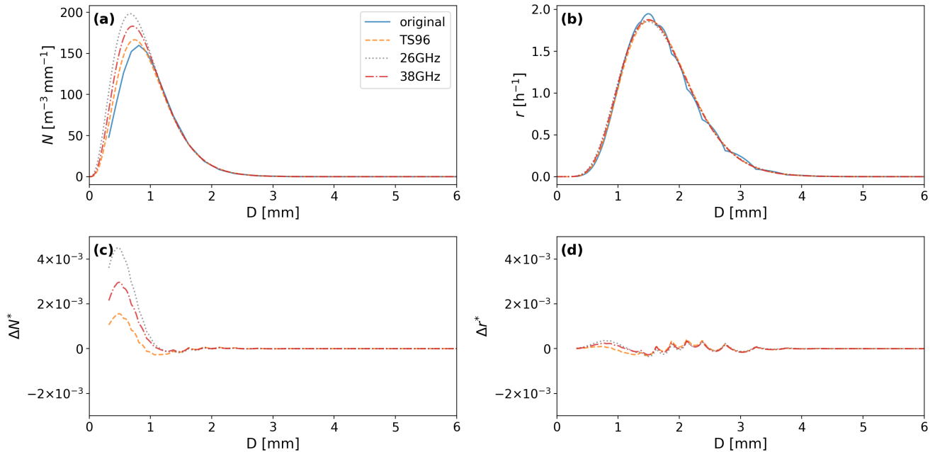
Figure 6. a) DSD retrieved from a single timestep in the first Ardèche event using several different microwave frequencies. b) Specific rain intensity for the same timestep. c) Relative difference in DSD compared to the original DSD. d) Relative difference in specific rain intensity compared to original DSD.
