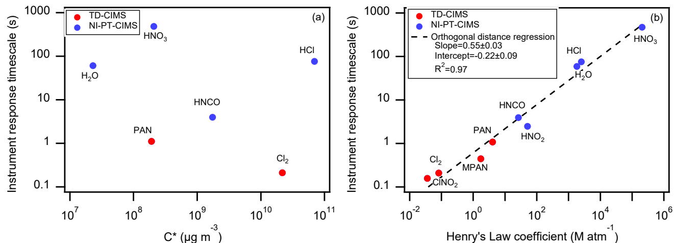
430 Figure 6. Instrument response timescales as a function of (a) saturation concentration and (b) Henry's Law coefficient for several inorganic compounds measured using TD-CIMS and NI-PT-CIMS. The dashed line is an orthogonal distance regression of the logarithm of the response timescale against the logarithm of Henry's Law coefficient. Peroxyacetyl nitrate and peroxyacryloyl nitrate are abbreviated as PAN and MPAN. No delay would be expected for these compounds due to partitioning to 435 Teflon, as they all have C^* > 10^7 \mu\text{g m}^{-3} .
