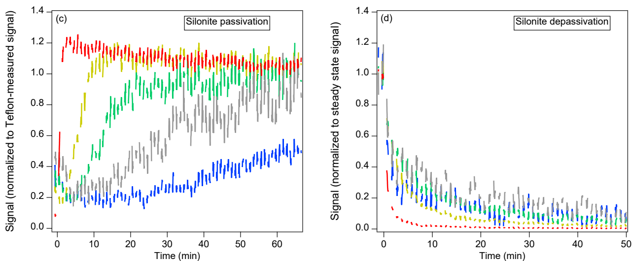
Figure 4. Examples of passivation and depassivation of stainless steel ((a) and (b)) for C_6 - C_{10} HNs and DHNs and Silonite ((c) and (d)) for C^* > 10^2 \mu\text{g m}^{-3} HNs and DHNs, where curves were binomially smoothed across 10 points for visual clarity. The stainless steel data were measured by the CU (Ziemann) CIMS. The Silonite data were measured with the UW CIMS, and the gaps were due to periodic background sampling. Note that the starting signals for (c) are not zero, due to compounds that remained in the instrument.
