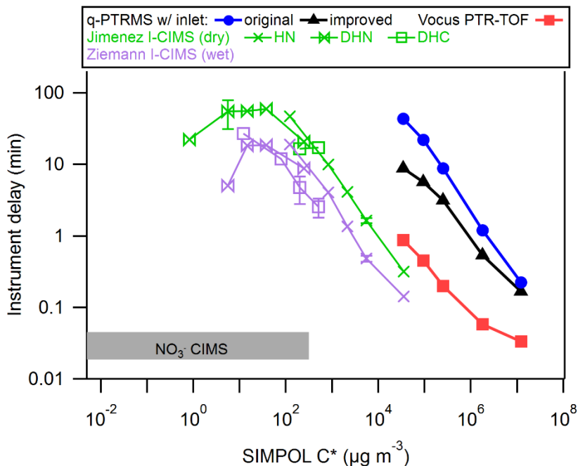
Figure 2. Measured instrument delay times as a function of SIMPOL C^* for five instruments. The q-PTRMS data are from Pagonis et al. (2017) and the Vocus PTR-TOF data are from Krechmer et al. (2018). Error bars are shown for some data points (the size would be similar for the rest of the points, not added to reduce figure clutter), calculated as standard deviations of two or three repeated measurements. Also shown are approximate delays (shaded area) observed with the \text{NO}_3 -CIMS in Krechmer et al. (2016).
