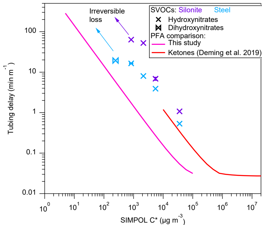
395 Figure 5. Stainless steel and Silonite depassivation delay times measured for a series of HNs and DHNs after equilibration with a chamber filled with alkanols and S/IVOCs, and compared with PFA modeled delays for 4 \text{ L min}^{-1} flows. Only compounds with 100% transmission efficiency through stainless steel and Silonite compared to Teflon tubing are shown. DHCs were not included in delay calculation due to relatively low S/N ratios in these experiments. The transmission became lower than 100% for DHCs with C^* < 10^2 \mu\text{g m}^{-3} through steel and C^* < 10^3 \mu\text{g m}^{-3} through Silonite. Example error bars (smaller than marker) were propagated from exponential fits.
