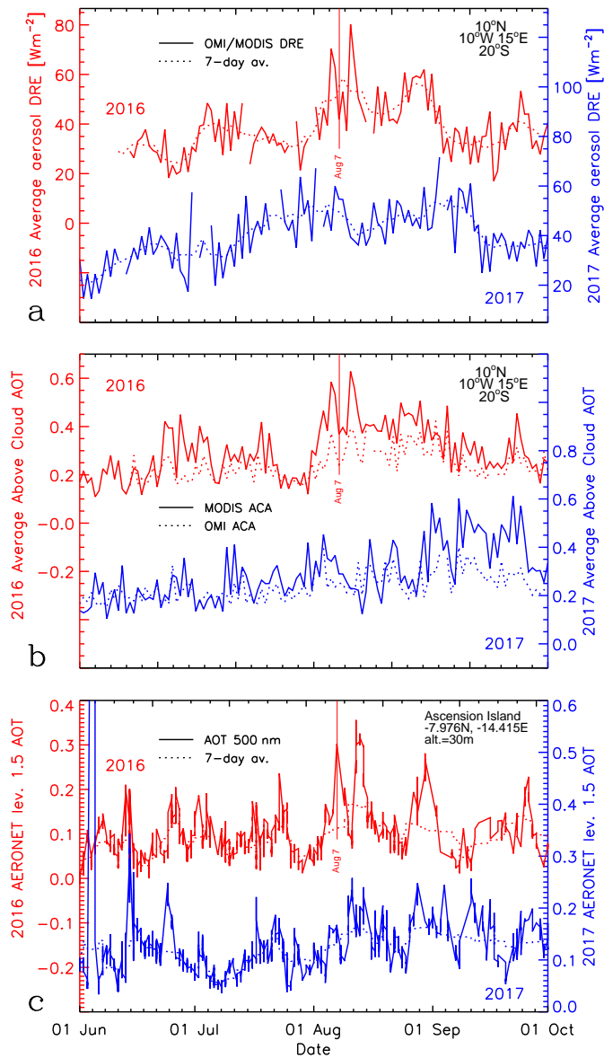
Figure 9. (a) OMI/MODIS aerosol DRE over clouds, averaged over the Atlantic Ocean ( 10^{\circ}\text{N} – 20^{\circ}\text{S} ; 10^{\circ}\text{W} – 15^{\circ}\text{E} ) in 2016 (red) and 2017 (blue). The solid line shows the area-average instantaneous DRE, the dashed line shows a 7-day running mean; (b) Above-cloud AOT (ACA) derived from MODIS (solid line) and OMI (dashed line) measurements during 2016 (red) and 2017 (blue), averaged over the same area as (a); (c): AERONET AOT at 500 nm from Ascension Island station at 7.98^{\circ}\text{S} , 14.42^{\circ}\text{W} in 2016 (red) and 2017 (blue). The solid line shows all available level 1.5 data, the dashed line shows a 100 point running mean.
