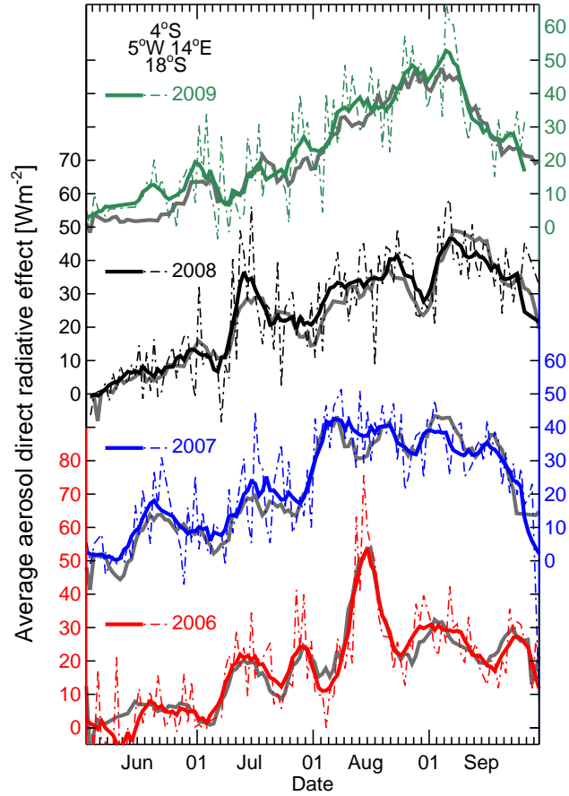
Figure 5. Area-averaged instantaneous aerosol DRE in \text{Wm}^{-2} for the region 4 to 18° S; 5° W to 14° E (local overpass times from about 9:00–10:30 UTC) in 2006–2009 (thin lines) and its 7-day running mean (bold lines) in colored lines for all OMI/MODIS pixels with \text{CF} > 0.3 and \text{CP} > 800 hPa. In bold grey the SCIAMACHY area averaged aerosol DRE is plotted for \text{CF} > 0.3 , \text{CP} < 800 hPa, which was published in de Graaf et al. (2014).
