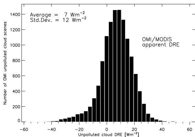
Figure 7. Frequency distribution of the apparent aerosol effect of all OMI aerosol-unpolluted marine water cloud scenes in June–Sept. 2006 over the south-east Atlantic Ocean ( 20^{\circ} S to 10^{\circ} N; 10^{\circ} W to 20^{\circ} E). The OMI/MODIS DRE for each pixel with OMI AI < 0, CF > 0.3 and CP > 800 hPa was considered. The offset (apparent DRE) for these pixels is 7 \text{ Wm}^{-2} , which is taken as the bias of the OMI/MODIS DRE method. The standard deviation of the DRE for these unpolluted scenes is 12 \text{ Wm}^{-2} , which is a measure of the random error of the DRE.
