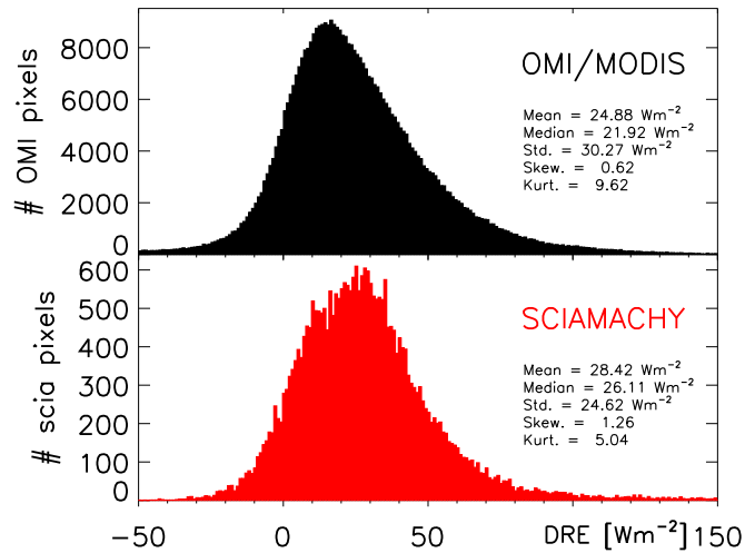
Figure 6. Histograms of SCIAMACHY and OMI/MODIS DRE in June to September 2006 over the south-east Atlantic Ocean (20° S to 10° N; 10° W to 20° E).
