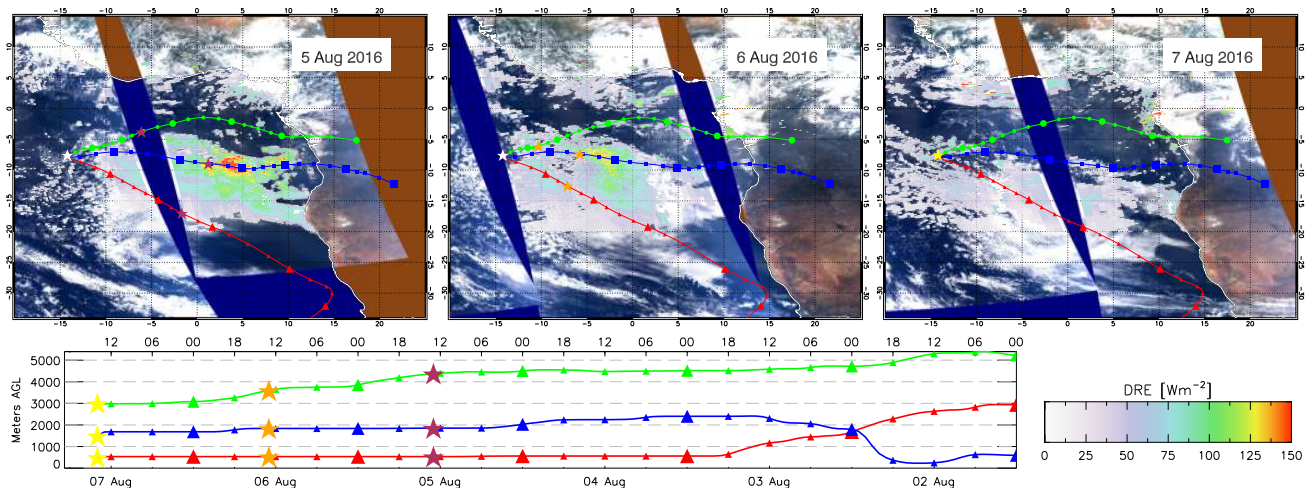
Figure 10. Aerosol DRE over clouds from OMI/MODIS overlaid over MODIS RGB images for three consecutive days (5,6,7 August), and backtrajectories from Ascension Island of air parcels ending at 500 m (red), 1500 m (blue) and 3000 m (green). The position of the air in the backtrajectories during the satellite overpasses is indicated by the coloured stars (yellow on 7 Aug. (at Ascension Island), orange on 6 Aug. and brown on 5 Aug.)
