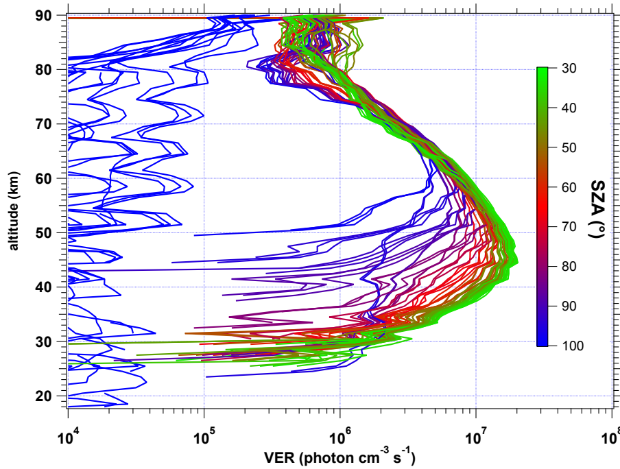
Figure 6. Volume emission rate (VER) profiles of airglow at 1.27 \mu m retrieved from SCIAMACHY limb data for the first of January 2007 (80 profiles). The colour scale represents the SZA (Solar Zenith Angle). For the lowest SZA values probed by SCIAMACHY ( 33^\circ ), the peak VER is 2 \times 10^7 photons cm^{-3} s^{-1} around 45 km. At large SZA values, the emission is present only at high altitudes ( >80 km). Above 90^\circ , there is almost no signal for inversion.
