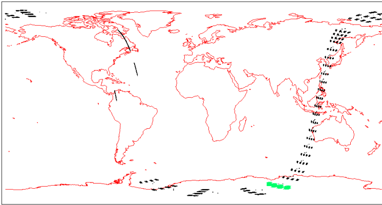
Figure F5. Geographic positions of SCIAMACHY LOS tangent points at the limb (by groups of four) for ENVISAT orbit 25293, starting 1th January 2007 at 01h 12mn. The green points are the locations of the limb spectra which are compared with our theoretical derivation in Section 3.
