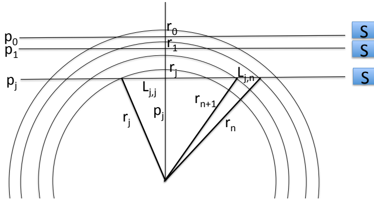
Figure B1. Geometry of the lines of sight LOS at the limb of an emission organized in spherical layers. The various LOS are obtained either by drifting the observer S into an orbit with a fixed inertial direction (case of GOMOS/ENVISAT), or by angular scanning (case of SCIAMACHY/ENVISAT).
