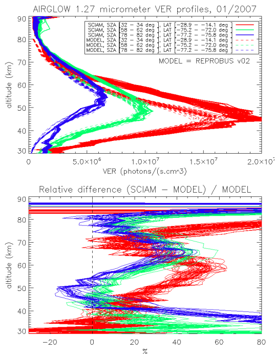
Figure 13. Top: Comparisons of all SCIAMACHY and REPROBUS airglow VER profiles for the first 3 days of January 2007 in three SZA domains: SZA =[32 - 34 °] (red curves), SZA =[58 - 62 °] (green curves) and SZA =[78 - 82 °] (blue curves). Only profiles from the southern hemisphere were selected. Bottom: for each profile, relative difference (SCIAMACHY -REPROBUS)/REPROBUS.
