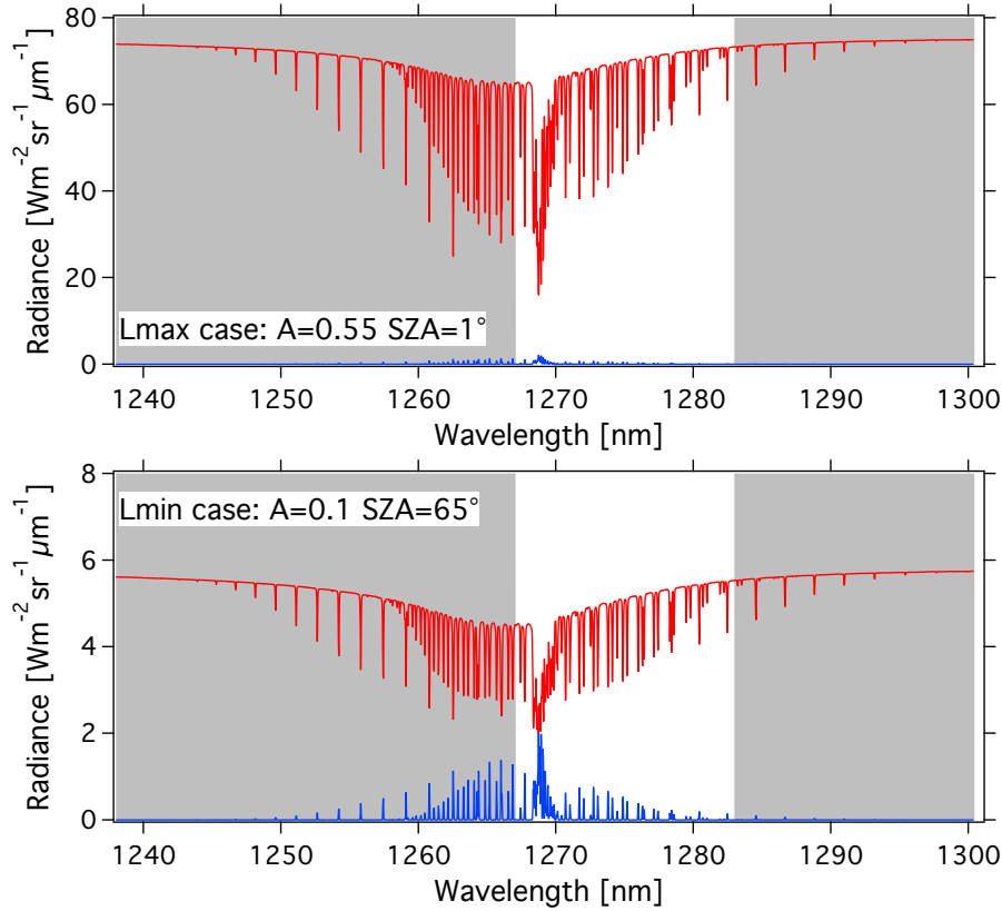
Figure 15. Airglow (blue) and scattered sunlight (red) absolute intensities and radiances (in W m^{-2} sr^{-1} \mu m^{-1} ) for two cases: Top: high albedo A=0.55 and almost sub solar SZA=1^\circ (referred as Lmax case (maximum luminance for instrument SNR estimates) and bottom: low albedo A=0.1 and high SZA=65^\circ (referred as Lmin case for SNR estimates for minimum luminance). The depression on the continuum of reflected sunlight is due to the O_2 CIA (Collision Induced Absorption, now included in HITRAN 2016, Gordon et al. 2017). Water vapour absorption lines are not represented here, which would be on the right part of the spectra. The white area corresponds to the MicroCarb wavelength coverage.
