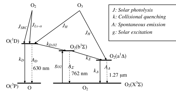
Figure 9. Energy diagram of O and O 2 molecule showing both O 2 bands at 762 nm (A) and 1.27 μm. Only the O 2 photo-dissociation ( J_{SRC} (Schumann-Runge continuum) and J_{Ly-a} ) is not taken into account in our model, since this represents only about 1% of the integrated emission (reproduced from Wiensz, 2005).
