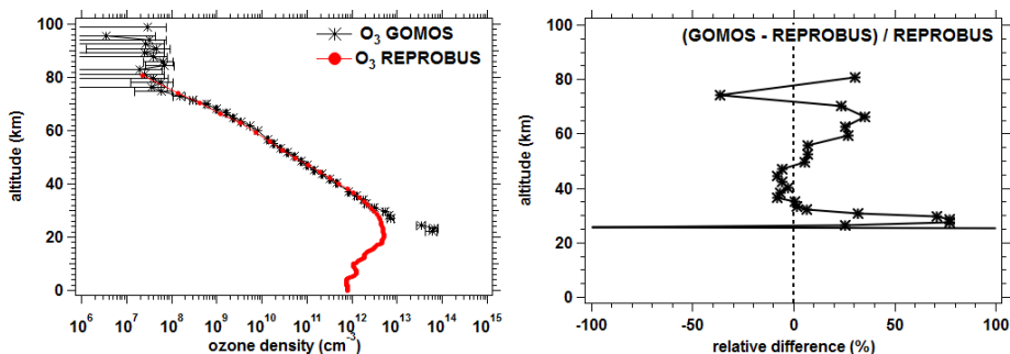
Figure C3 Left: One example of comparison of a GOMOS vertical dayside ozone profile (black curve) vs. REPROBUS prediction (red curve). The GOMOS profile was observed on August 5 2007, at an SZA angle of 38°. Right: relative difference (GOMOS-REPROBUS)/ REPROBUS .
