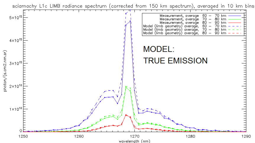
Figure 4a. SCHIAMACHY limb spectra (solid lines, absolute units are photons/(s cm 2 nm sr)), binned by altitudes (60-70 km, 70-80 km, and 80-90 km), along with our model spectra computed for the same scans and binned in the same way.
