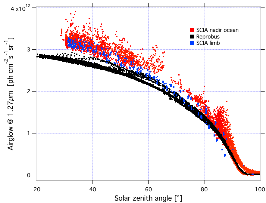
Figure 18: Airglow intensity at nadir according to the SZA for the month of April 2007: in red SCIAMACHY measurements at nadir with a reflected solar spectral radiance < 5 \text{ W} \cdot \text{m}^{-2} \cdot \text{sr}^{-1} \cdot \mu\text{m}^{-1} , in blue nadir intensities retrieved from SCIAMACHY measurements at the limb, in black simulations with REPROBUS v02. The airglow intensity at its maximum reaches 3.2 \times 10^{12} \text{ photons cm}^{-2} \text{ s}^{-1} \text{ sr}^{-1} which corresponds to 5 \text{ mW m}^{-2} \text{ sr}^{-1} (spread over a few nanometers of wavelength), to be compared to a solar backscattered luminance (radiance) of \sim 5 \text{ to } 70 \text{ Watt m}^{-2} \text{ sr}^{-1} \cdot \mu\text{m}^{-1} (see Fig. 16).
