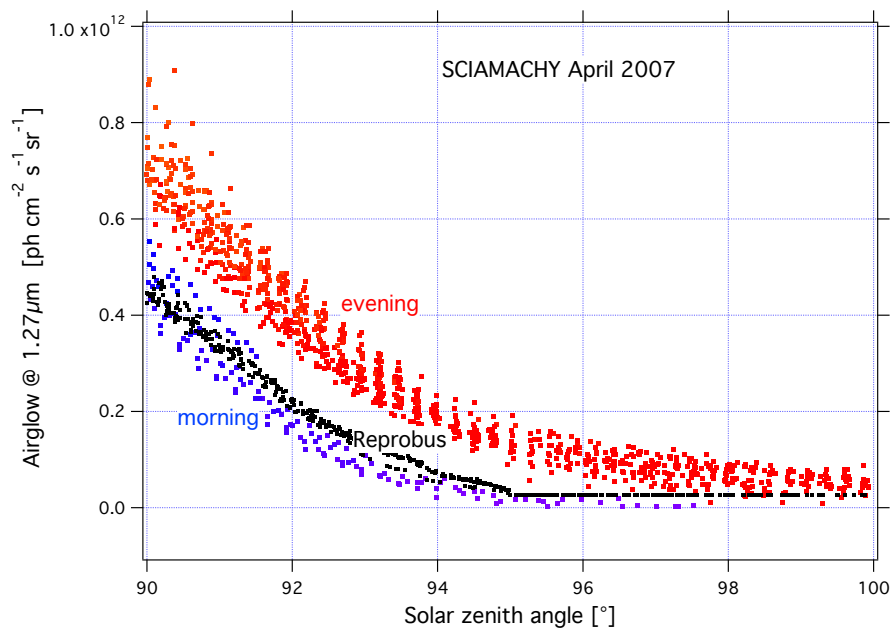
Figure 19: Airglow nadir intensity versus SZA for SZA > 90°; SCIAMACHY measurements in red during evening and in blue during morning; REPROBUS v02 simulations in black. The observed difference between morning and evening values is due to the long lifetime of O_2(a^1\Delta_g) .
