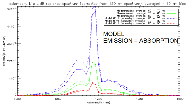
Figure 4b. Same as Fig. 4a, but with the crude model in which the shape of the emission of O_2^* is identical to the absorption by O_2 . This crude model shows an excess of emission in the R branch (left) and a deficit in the P branch.
