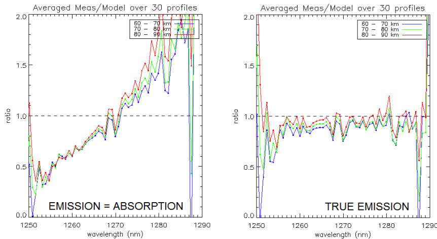
15 Figure 5: Ratios of measured spectra/model spectra of limb spectra, averaged over a whole ENVISAT orbit, and binned by altitudes (60-70 km, 70-80 km, and 80-90 km). Left: crude model in which the shape of the emission of O_2^* is identical to the absorption by O_2 . Right: same ratios with our new model described in Appendix A. The ratios are
