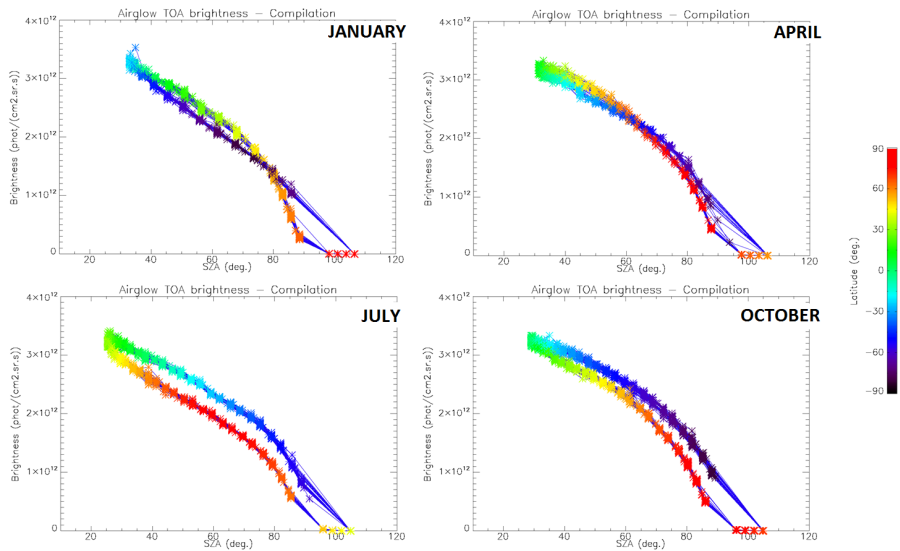
Figure 8. O_2^* airglow intensities that would be seen at nadir as a function of SZA for the months of January, April, July and October 2007 (first 3 days of each month only), retrieved from the processing of SCIAMACHY limb data. The colour scale represents the latitude. There is a geometrical correlation between the latitude and SZA imposed by the polar orbit of ENVISAT. The airglow brightness is mostly correlated with SZA. The comparison of these intensities with those obtained by the REPROBUS airglow model is presented in subsection 4.2.1.
