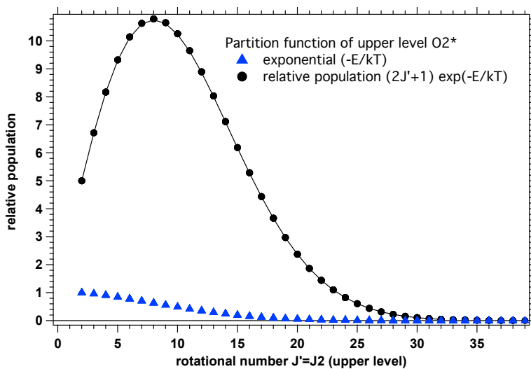
Figure A2. Partition function of the \text{O}_2^* molecule as a function of rotation state J' for T=296 \text{ K} . Blue triangles: exponential term for population, =1 for the lowest; Black circles: the relative population computed from informations contained in the HITRAN database of transitions. It allows to retrieve the allowed values of J' . The first point is for J'=2 with value 5=2J'+1 , and \exp(0)=1 . The sum of all relative populations is Q_{\text{tot}}^{\text{up}} by definition.
