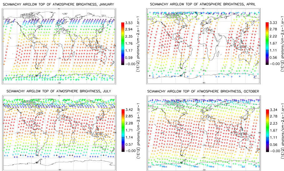
Figure 7. Airglow brightness maps as seen from space in nadir view, retrieved from SCIAMACHY limb viewing data for the months of January, April, July and October 2007 (first 3 days of each month only). The colour scale represents brightness. Zones without data (holes), particularly numerous in April, are corrupted products that have been eliminated. SZA points > 90^\circ have been eliminated.
