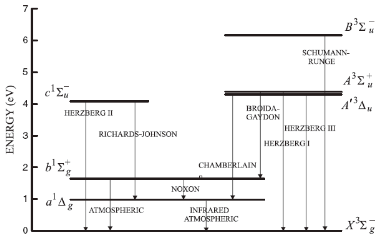
Figure A1. Energy levels of the various electronic states of the di-oxygen molecule O 2 , and name of electronic transitions between them (reprinted by permission from Springer Nature Customer Service Centre GmbH: Springer Verlag, Processes Responsible for the Occurrence of the Airglow by Vladislav Yu. Khomich, Anatoly I. Semenov, Nicolay N. Shefov, copyright 2008). The present study is relevant to the so-called «infrared atmospheric» transition.
