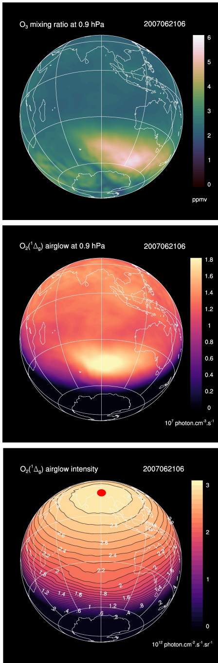
Figure 10. Simulations of the REPROBUS model for June 21, 2007 06:00 UT. This is the geographical distribution of
