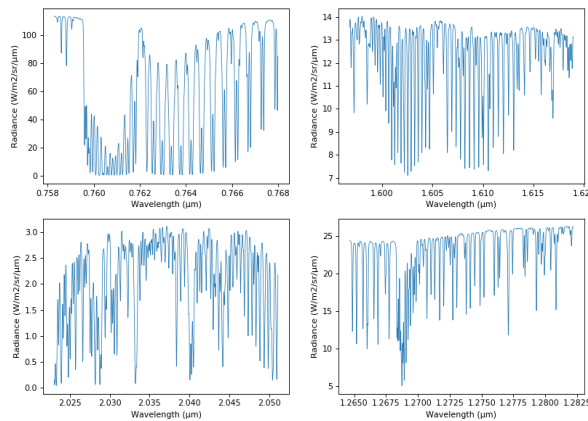
Figure 14: Example of MicroCarb simulated spectra of the strong O 2 band B1 (left upper panel), the weak CO 2 band B2 (upper right panel), the strong CO 2 band B3 (lower left panel) and the weak O 2 band B4 (lower right panel).
