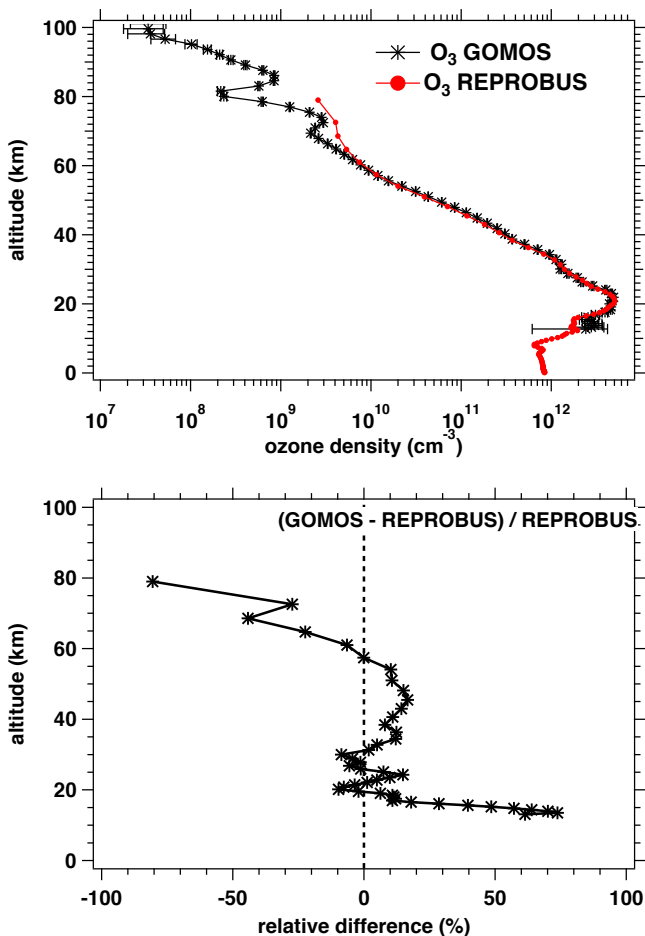
5 Figure C1 Top: One typical example of comparison of a GOMOS vertical ozone profile (black curve) vs. REPROBUS prediction (red curve). The GOMOS profile was observed during the night on January 8, 2007. Bottom: relative difference (\text{GOMOS} - \text{REPROBUS}) / \text{REPROBUS} .
