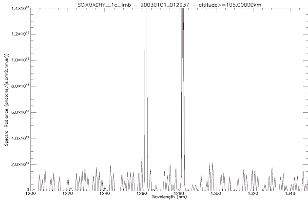
Figure F1. This high altitude spectrum recorded above 105 km contains some residual spectral (readout) patterns left from the calibration step and is subtracted from all measurements obtained at lower altitude in the same scan limb.
