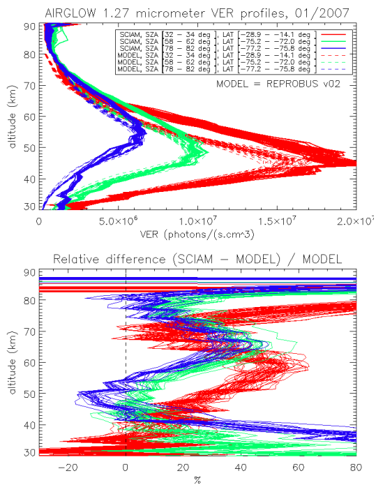
15 Figure 13. Top: Comparisons of all SCIAMACHY and REPROBUS airglow VER profiles for the first 3 days of January 2007 in three SZA domains: SZA = [32 - 34 °] (red curves), SZA = [58 - 62 °] (green curves) and SZA = [78 - 82 °] (blue curves). Only profiles from the southern hemisphere were selected. Bottom: for each profile, relative difference (SCIAMACHY -REPROBUS)/REPROBUS.
