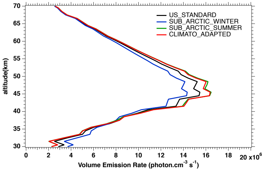
Figure B2: VER airglow profiles obtained by taking into account O 2 absorption using a climatological atmospheric profile SUBARCTIC_SUMMER (green curve), SUBARCTIC_WINTER (blue curve), US STANDARD (black curve), and CLIMATO_ADAPTED (red curve). In the case of this profile measured in January at latitude=-39.9 ° the adapted climatology corresponds to the MIDLAT-SUMMER climatology.
