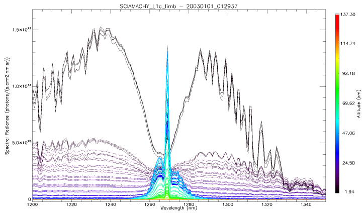
Figure F3: Same as Figure F2, after correction of the two bad pixels. In addition to the O_2^* airglow, there is the radiance of solar light scattered by air and aerosols, increasing when tangent altitude is decreasing. The strong absorption of O_2 in the 1.27 \mu m band becomes obvious at lowest altitudes.
