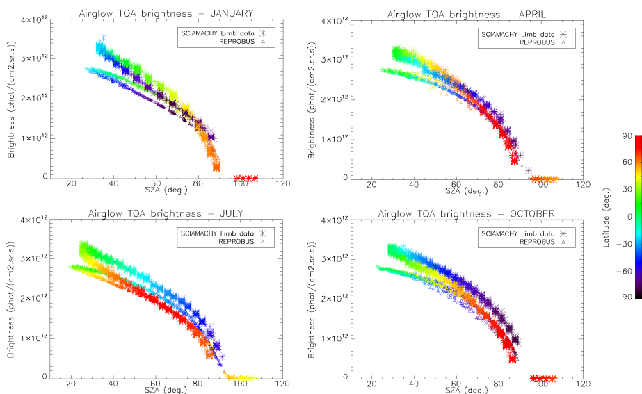
20 Figure 11. Airglow intensity seen at nadir as a function of SZA for the months of January, April, July and October 2007 (first 3 days of each month only). Data (star symbol) come from the SCIAMACHY limb data (retrieval of VER with onion-peel inversion and subsequent vertical integration); (Δ symbol) from the REPROBUS/airglow model. The colour scale for symbols represents latitude. The SZA for the SCIAMACHY curve was recalculated with an external tool. The data are systematically larger than the model but overall behaviours are similar.
