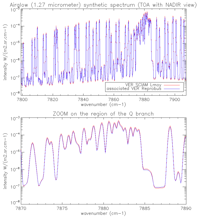
5 Figure D2: (Upper plot) synthetic airglow spectra corresponding to the (red) SCIAMACHY VER profile of Fig. D1, (blue) associated REPROBUS VER profiles of Fig. D1. For the 3 tests, the red spectrum is put in the simulated data to invert. For the test #1 it is also used as the jacobian of the inverse model. For the test #2, the blue spectrum is used as jacobian of the inverse model (blue). The jacobian spectra of test #3 are not represented here. (Bottom plot) zoom on the region of the Q branch.
