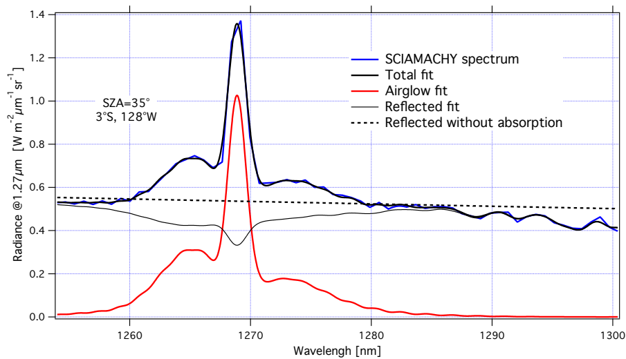
Figure 16: Two examples of SCIAMACHY spectra at nadir; (top) above thick clouds and (bottom) above clear ocean. SCIAMACHY spectrum is in blue, fitted spectrum in thick black, determined airglow spectrum in red, fitted reflected spectrum in light black, reflected spectrum without absorption in dotted black. The word “radiance” in the label axis means the spectral radiance or intensities.
