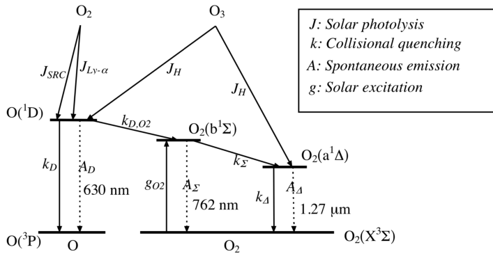
Figure 9. Energy diagram of O and O 2 molecule showing both O 2 bands at 762 nm (A) and 1.27 μm. Only the O 2 photo-dissociation ( J_{SRC} (Schumann-Runge continuum) and J_{Ly-\alpha} ) is not taken into account in our model, since this represents only about 1% of the integrated emission (reproduced from Wiensz, 2005).
