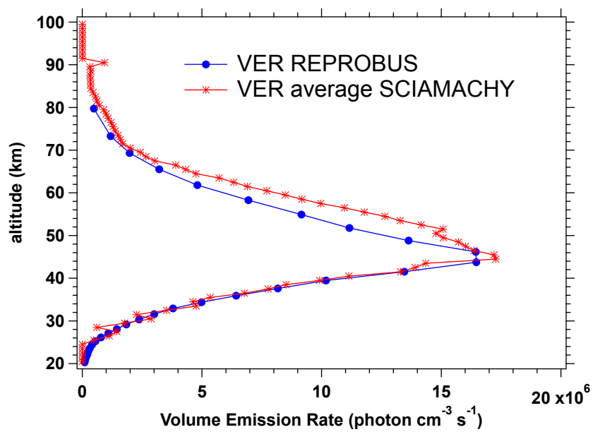
Figure D1: (In red) VER SCIAMACHY profile used to build the synthetic airglow spectrum put in the simulated spectrum to be inverted. (In blue) associated (co-located) REPROBUS VER profile, showing the underestimation of REPROBUS airglow modelling above 50 km. The airglow synthetic spectra associated to these two VER profiles are illustrated on Fig. D2. They are very similar.
