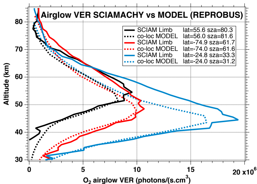
Figure 12. Comparison of SCIAMACHY and REPROBUS airglow VER profiles for January 3, 2007. Three profiles were drawn at SZAs of about 30°, 60° and 80°, indicated in the legend. The SCIAMACHY profiles are plotted as solid lines and the geo-located REPROBUS profiles are in dashed line.
