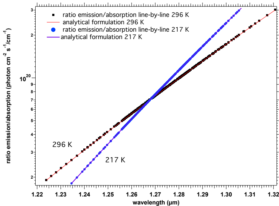
Figure A5: For two different temperatures: 296 and 217 K, the ratio of our calculated emission rate to the HITRAN line strength SS are plotted (respectively black and blue dots), for all 375 transitions of HITRAN table (between 1.2238 and 1.32068 μm). The solid lines (respectively red and blue) are computed from the analytical formula (A13) on a grid of wavelength/wavenumber using the same scale on the left as the ratio emission/line strength in units of photon cm -2 s -1 / cm -1 , where cm -1 is a wave number unit.
