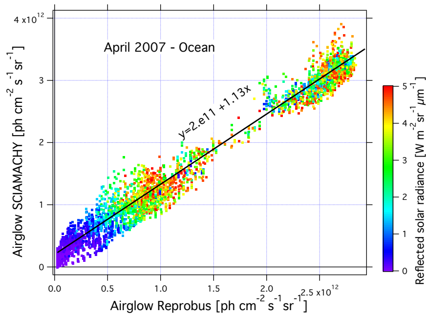
Figure 20: Nadir Airglow SCIAMACHY observed intensities versus REPROBUS v02 simulation (same units on both axes, photons \text{cm}^{-2} \text{s}^{-1} \text{sr}^{-1} ). The dots are coloured according to the reflected solar radiance from 0 in blue to 5 \text{ W m}^{-2} \text{sr}^{-1} \mu\text{m}^{-1} in red. Linear regression of the correlation is in black. Airglow intensity values are expressed in \text{ph} \cdot \text{cm}^{-2} \cdot \text{s}^{-1} \cdot \text{sr}^{-1} .
