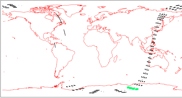
5 | Figure F5. Geographic positions of SCIAMACHY LOS tangent points at the limb (by groups of four) for ENVISAT orbit 25293, starting 1th January 2007 at 01h 12mn. The green points are the locations of the limb spectra which are compared with our theoretical derivation in Section 3.
