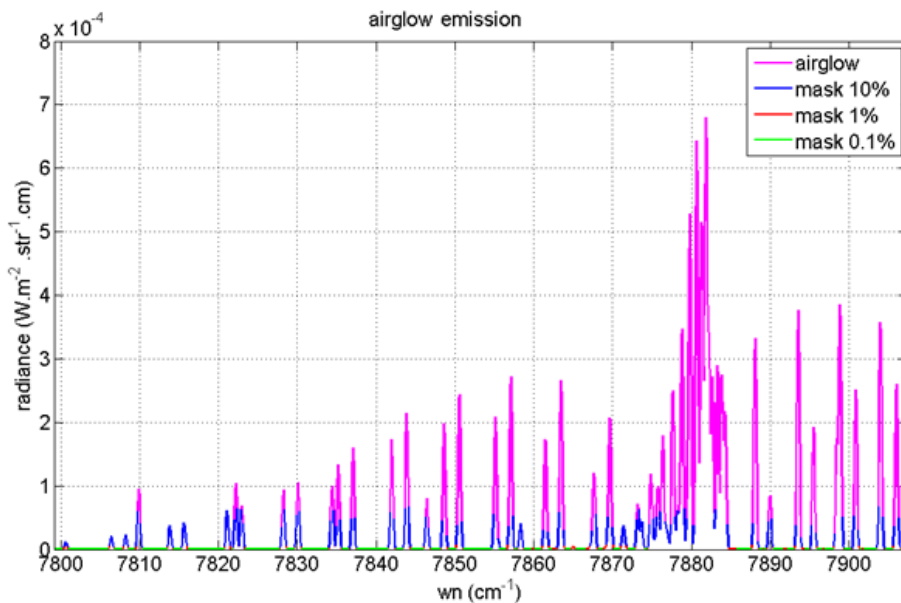
Figure D3: Airglow spectra at 1.27 \mu\text{m} , at Microcarb resolution, used in our tests of inversion of Psurf with method #2 for several values of the spectel mask: no mask (pink), 10% mask (blue), 1% mask (red), 0.1% mask (green). The three masks remove respectively 14%, 31% and 44% of the spectels in the B4 band.
