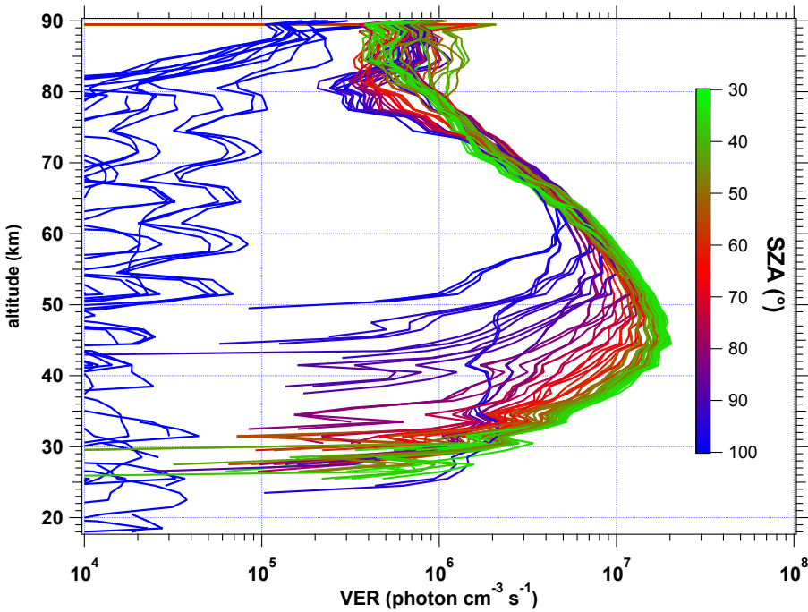
Figure 6. Volume emission rate (VER) profiles of airglow at 1.27 \mu\text{m} retrieved from SCIAMACHY limb data for the first of January 2007 (80 profiles). The colour scale represents the SZA (Solar Zenith Angle). For the lowest SZA values probed by SCIAMACHY (33 ^\circ ), the peak VER is 2 \times 10^7 photons \text{cm}^{-3} \text{s}^{-1} around 45 km. At large SZA values, the emission is present only at high altitudes (>80 km). Above 90 ^\circ , there is almost no signal for inversion.
