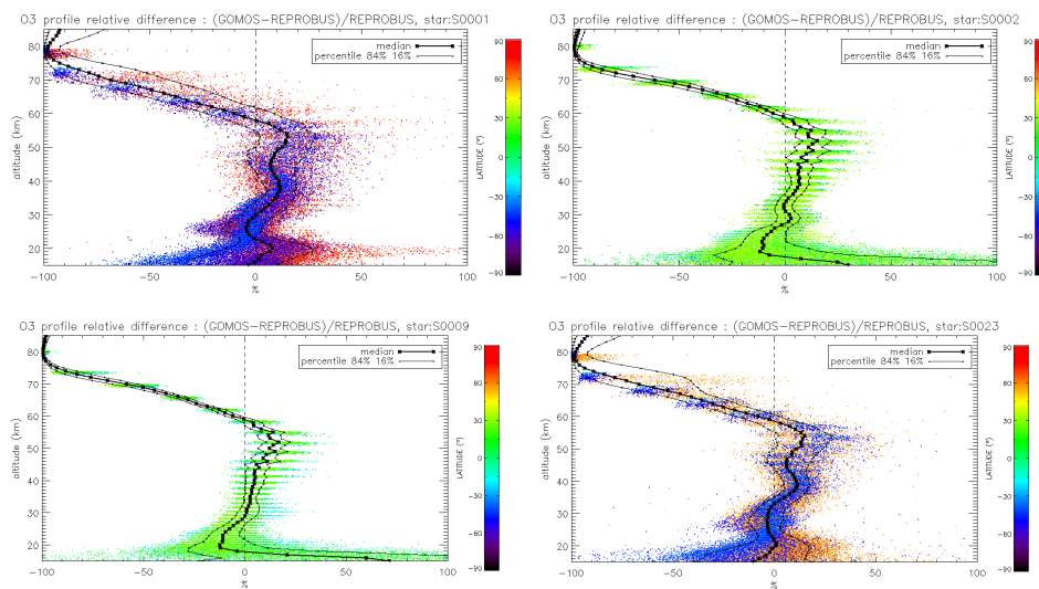
Figure C2. Relative difference between the GOMOS and REPROBUS ozone night-time profiles for all 2007 occultations of the four brightest stars represented here from left to right and top to bottom: S0001, S0002, S0009, S0023. Each dot represents one GOMOS measurement of ozone. The colour of the dot is related to the latitude of each profile (see colour scale). The thick black line represents the median and the thin black lines represent the percentiles 16% and 84% of the distribution of the relative difference.
