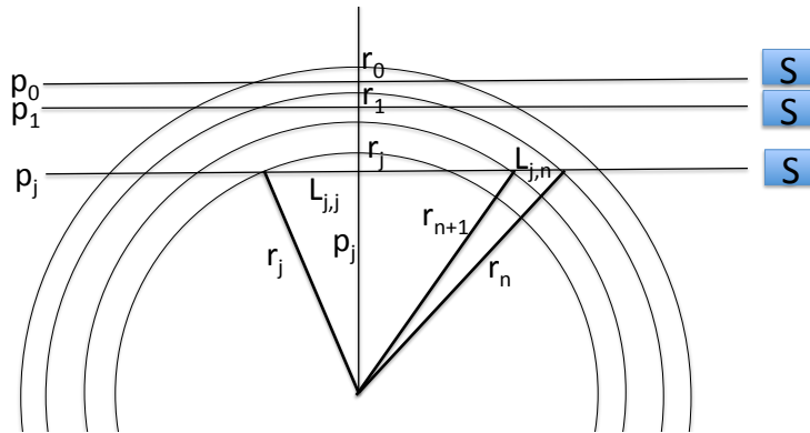
Figure B1. Geometry of the lines of sight LOS at the limb of an emission organized in spherical layers. The various LOS are obtained either by drifting the observer S into an orbit with a fixed inertial direction (case of GOMOS/ENVISAT), or by angular scanning (case of SCIAMACHY/ENVISAT).
