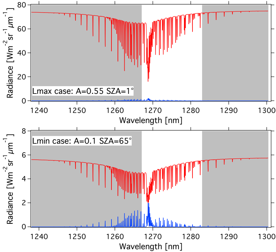
10 Figure 15. Airglow (blue) and scattered sunlight (red) absolute intensities and radiances (in \text{W m}^{-2} \text{sr}^{-1} \mu\text{m}^{-1} ) for two cases: Top: high albedo A=0.55 and almost sub solar \text{SZA}=1^\circ (referred as Lmax case (maximum luminance for instrument SNR estimates) and bottom: low albedo A=0.1 and high \text{SZA}=65^\circ (referred as Lmin case for SNR estimates for minimum luminance). The depression on the continuum of reflected sunlight is due to the O_2 CIA (Collision Induced Absorption, now included in HITRAN 2016, Gordon et al. 2017). Water vapour absorption lines are not represented here, which would be on the right part of the spectra. The white area corresponds to the MicroCarb wavelength coverage. 15
