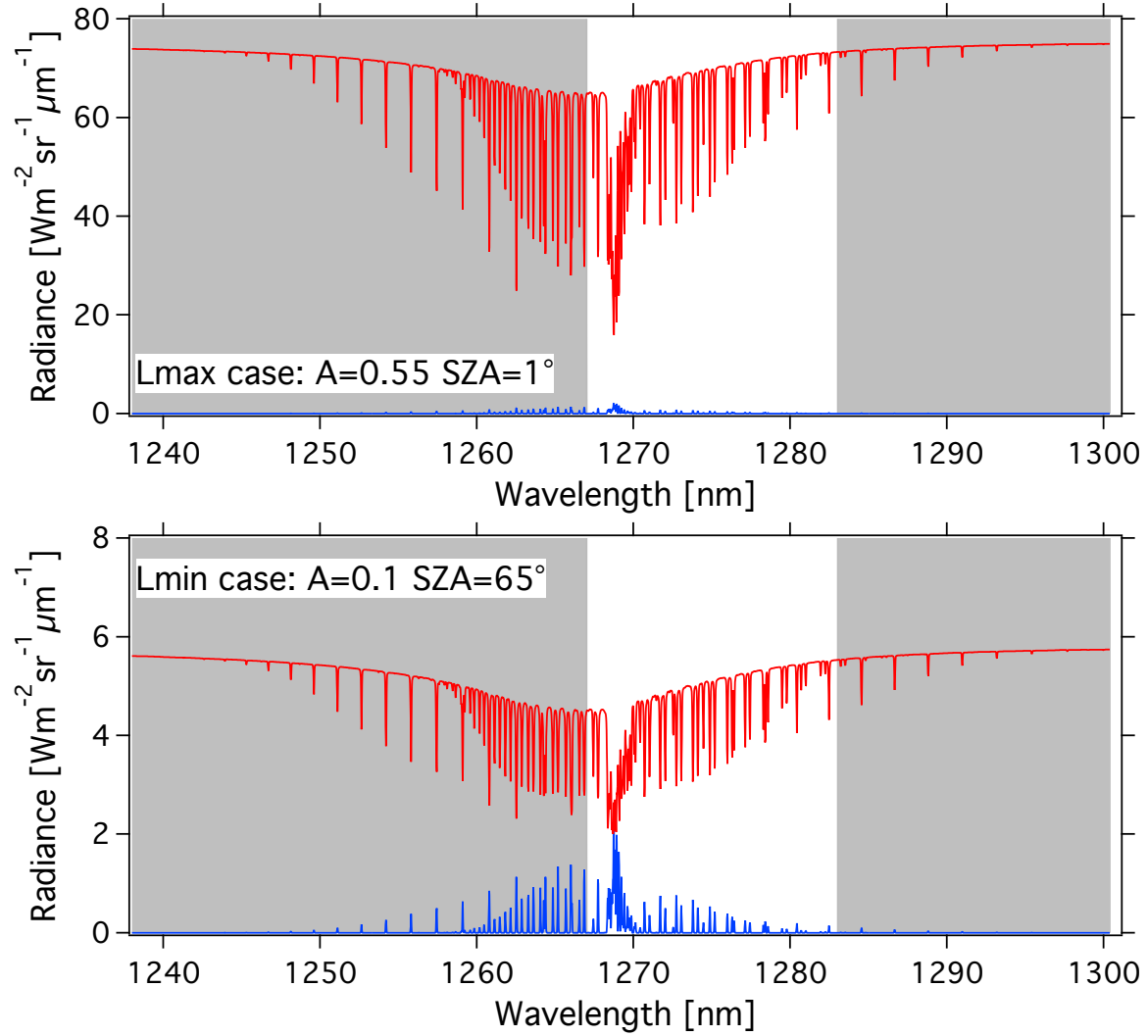
Figure 15. Airglow (blue) and scattered sunlight (red) absolute intensities and radiances (in W m^{-2} sr^{-1} \mu m^{-1} ) for two cases: Top: high albedo A=0.55 and almost sub solar SZA= 1^\circ (referred as Lmax case (maximum luminance for instrument SNR estimates) and bottom: low albedo A=0.1 and high SZA= 65^\circ (referred as Lmin case for SNR estimates for minimum luminance). The depression on the continuum of reflected sunlight is due to the O_2 CIA (Collision Induced Absorption, now included in HITRAN 2016 , Gordon et al. 2017). Water vapour absorption lines are not represented here, which would be on the right part of the spectra. The white area corresponds to the MicroCarb wavelength coverage.
