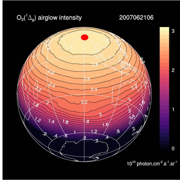
Figure 10. Simulations of the REPROBUS model for June 21, 2007 06:00 UT. This is the geographical distribution of three relevant quantities with their colour code. Top: Ozone mixing ratio (ppmv) at 0.9 hPa (about 50 km). Middle: Volume emission rate of O_2(a^1\Delta) at 0.9 hPa, in units of 10^7 \text{ photon.cm}^{-3}.\text{s}^{-1} . Bottom: Integrated vertical intensity of O_2(a^1\Delta) , in units of 10^{12} \text{ photon.cm}^{-2}.\text{s}^{-1}.\text{sr}^{-1} . Because of the particular time and date, the subsolar point is at latitude 23.5^\circ \text{ N} and on the meridian 90^\circ \text{ East} , which is the red spot plotted at the centre of bottom figure.
