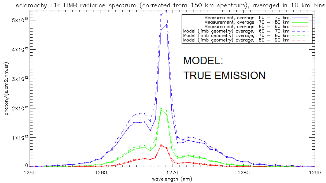
Figure 4a. SCIAMACHY limb spectra (solid lines, absolute units are photons/(s cm 2 nm sr)), binned by altitudes (60-70 km, 70-80 km, and 80-90 km), along with our model spectra computed for the same scans and binned in the same way.
