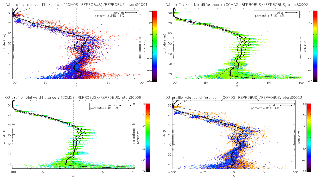
Figure C2. Relative difference between the GOMOS and REPROBUS ozone night-time profiles for all 2007 occultations of the four brightest stars represented here from left to right and top to bottom: S0001, S0002, S0009, S0023. Each dot represents one GOMOS measurement of ozone. The colour of the dot is related to the latitude of each profile (see colour scale). The thick black line represents the median and the thin black lines represent the percentiles 16% and 84% of the distribution of the relative difference.
