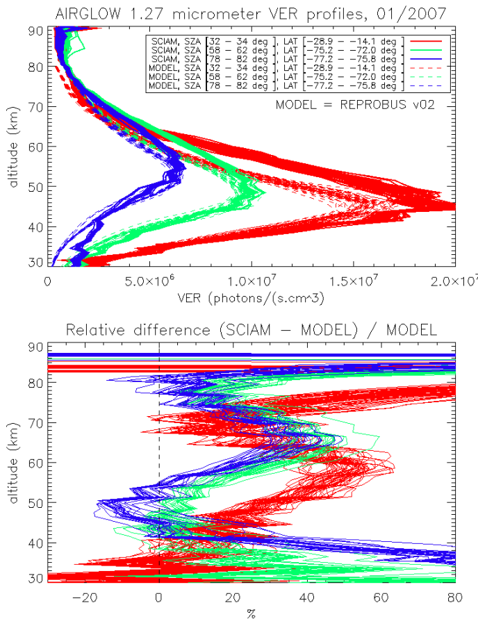
15 Figure 13. Top: Comparisons of all SCIAMACHY and REPROBUS airglow VER profiles for the first 3 days of January 2007 in three SZA domains: SZA =[32 - 34 °] (red curves), SZA =[58 - 62 °] (green curves) and SZA =[78 - 82 °] (blue curves). Only profiles from the southern hemisphere were selected. Bottom: for each profile, relative difference (SCIAMACHY -REPROBUS)/REPROBUS.
