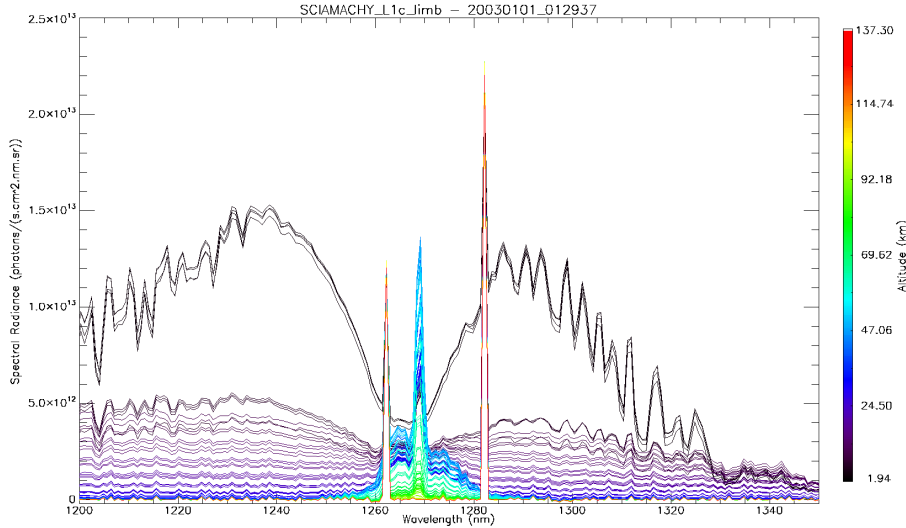
Figure F2. Spectra corrected from high altitude spectrum showing still two bad pixels at wavelength 1262.267 nm and 1282.128 nm. We replaced their value by the average of their two surrounding pixels to obtain spectra of Figure F3. The tangent altitude of the LOS is colour coding each spectrum.
