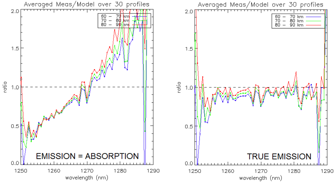
Figure 5: Ratios of measured spectra/model spectra of limb spectra, averaged over a whole ENVISAT orbit, and binned by altitudes (60-70 km, 70-80 km, and 80-90 km). Left: crude model in which the shape of the emission of O_2^* is identical to the absorption by O_2 . Right: same ratios with our new model described in Appendix A. The ratios are nearer 1 for larger altitudes because absorption by O_2 is neglected in this particular exercise.
