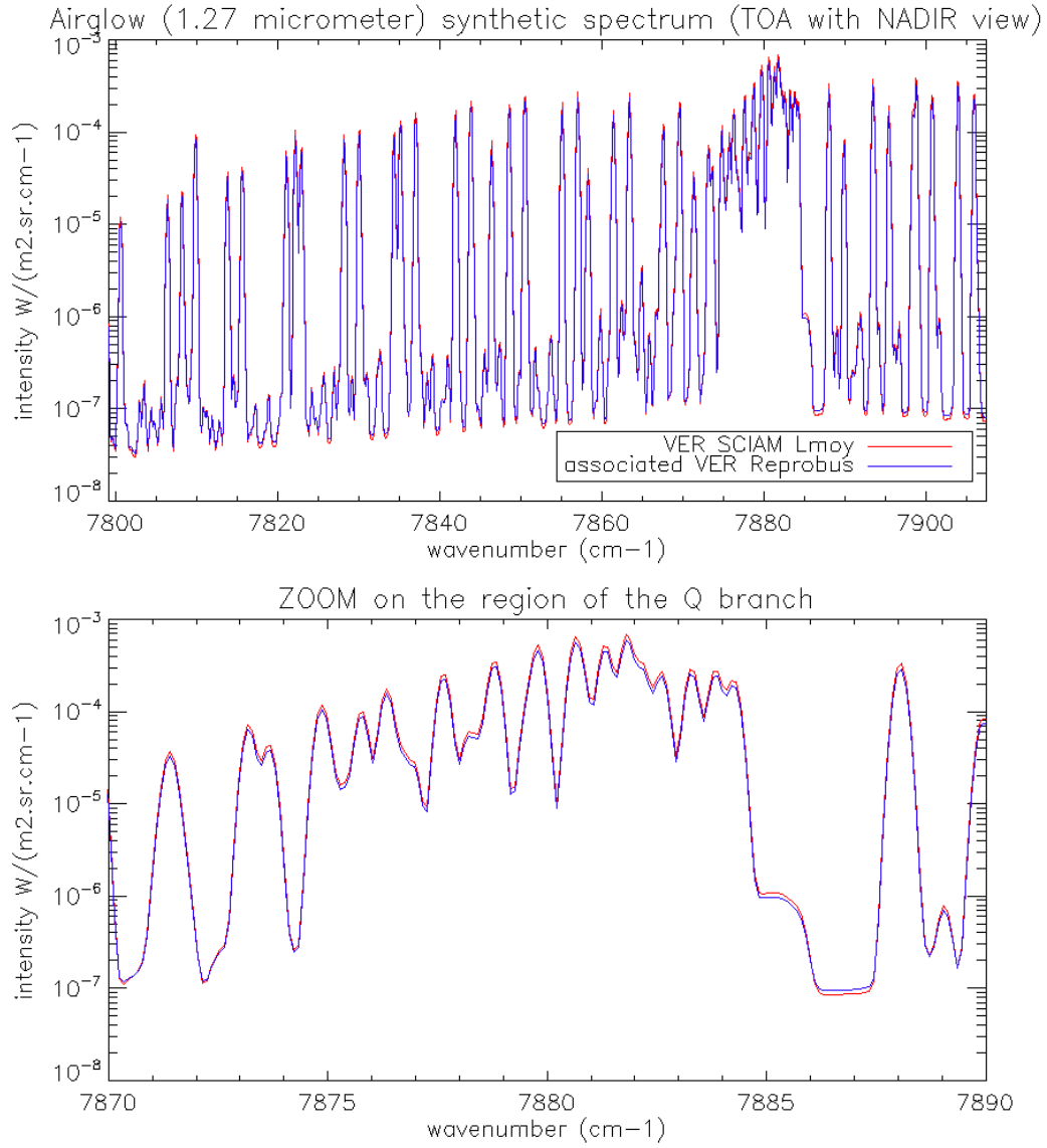
Figure D2: (Upper plot) synthetic airglow spectra corresponding to the (red) SCIAMACHY VER profile of Fig. D1, (blue) associated REPROBUS VER profiles of Fig. D1. For the 3 tests, the red spectrum is put in the simulated data to invert. For the test #1 it is also used as the jacobian of the inverse model. For the test #2, the blue spectrum is used as jacobian of the inverse model (blue). The jacobian spectra of test #3 are not represented here. (Bottom plot) zoom on the region of the Q branch.
