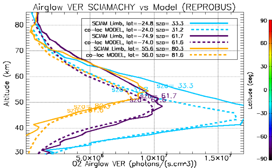
Figure 12. Comparison of SCIAMACHY and REPROBUS airglow VER profiles for January 3, 2007. Three profiles were drawn at SZAs of about 30^\circ , 60^\circ and 80^\circ , indicated in the legend. The SCIAMACHY profiles are plotted as solid lines and the geolocated REPROBUS profiles are in dotted line. The colour scale represents latitude.
