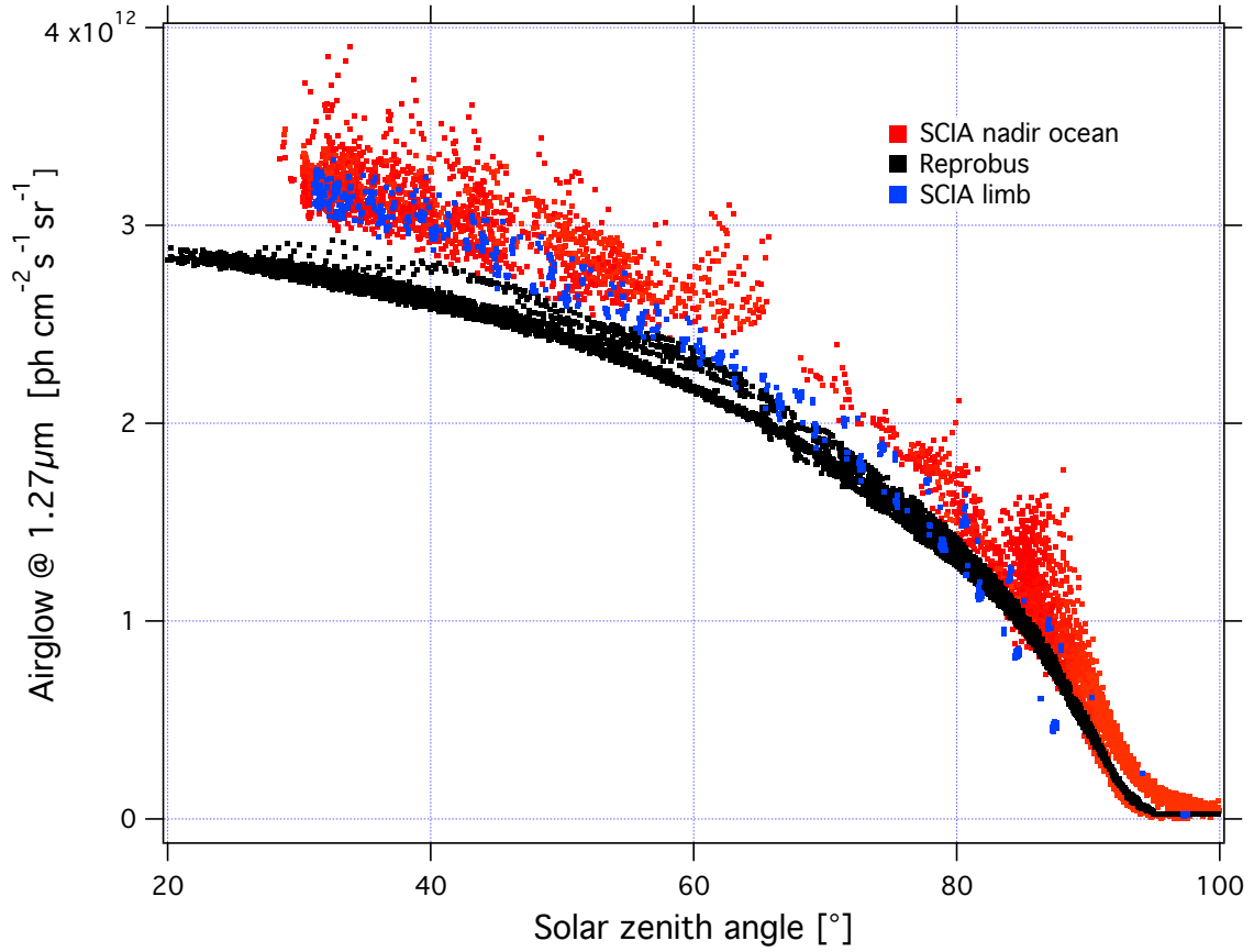
Figure 18: Airglow intensity at nadir according to the SZA for the month of April 2007: in red SCIAMACHY measurements at nadir with a reflected solar spectral radiance < 5 \text{ W.m}^{-2}.\text{sr}^{-1} \mu\text{m}^{-1} , in blue nadir intensities retrieved from SCIAMACHY measurements at the limb, in black simulations with REPROBUS v02. The airglow intensity at its maximum reaches 3.2 \times 10^{12} \text{ photons cm}^{-2} \text{ s}^{-1} \text{ sr}^{-1} which corresponds to 5 \text{ mW m}^{-2} \text{ sr}^{-1} (spread over a few nanometers of wavelength), to be compared to a solar backscattered luminance (radiance) of \sim 5 to 70 \text{ Watt m}^{-2} \text{ sr}^{-1} \mu\text{m}^{-1} (see Fig. 16).
