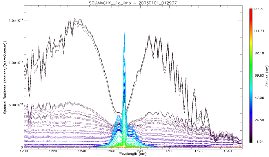
Figure F3: Same as Figure F2, after correction of the two bad pixels. In addition to the O_2^* airglow, there is the radiance of solar light scattered by air and aerosols, increasing when tangent altitude is decreasing. The strong absorption of O_2 in the 1.27 \mu m band becomes obvious at lowest altitudes.
