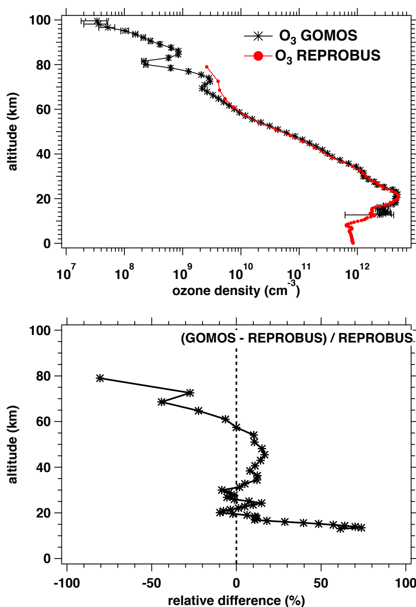
5 Figure C1 Top: One typical example of comparison of a GOMOS vertical ozone profile (black curve) vs. REPROBUS prediction (red curve). The GOMOS profile was observed during the night on January 8, 2007. Bottom: relative difference (GOMOS - REPROBUS)/ REPROBUS.
