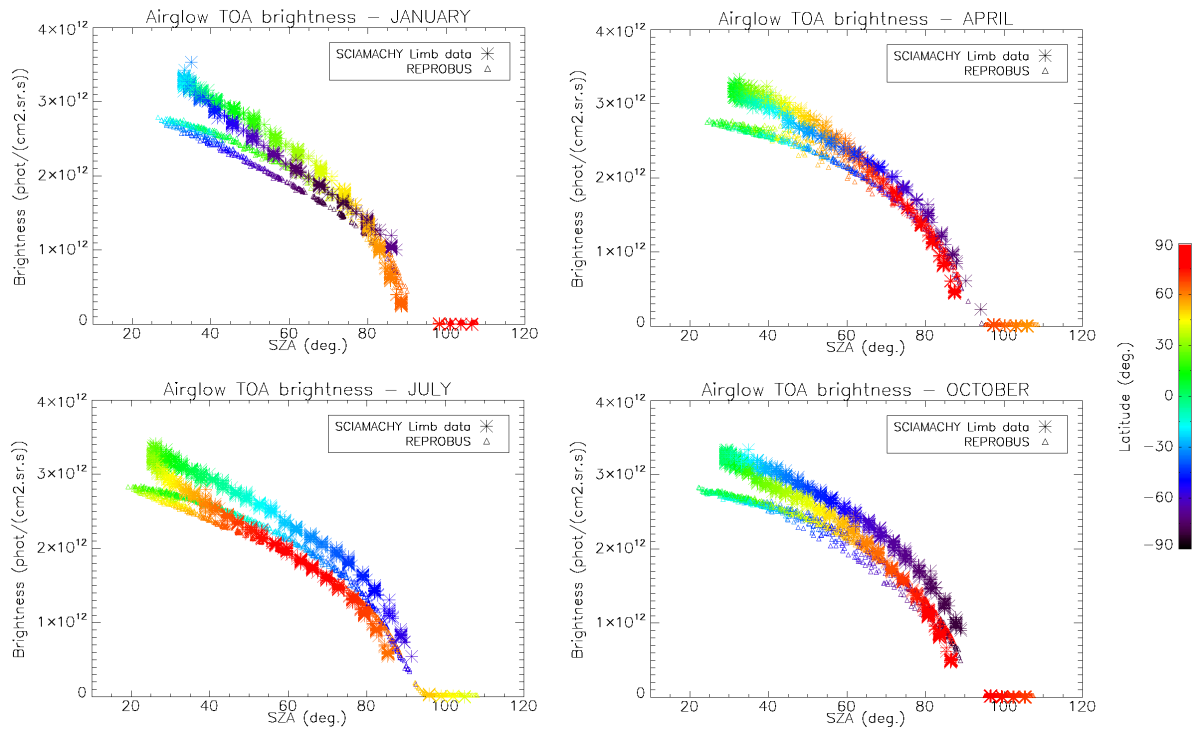
Figure 11. Airglow intensity seen at nadir as a function of SZA for the months of January, April, July and October 2007 (first 3 days of each month only). Data (star symbol) come from the SCIAMACHY limb data (retrieval of VER with onion-peel inversion and subsequent vertical integration); ( \Delta symbol) from the REPROBUS/airglow model. The colour scale for symbols represents latitude. The SZA for the SCIAMACHY curve was recalculated with an external tool. The data are systematically larger than the model but overall behaviours are similar.
