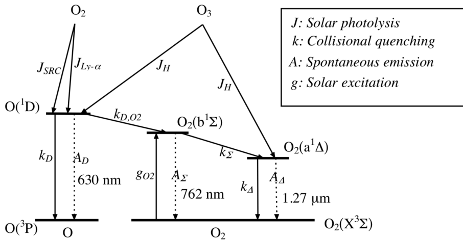
Figure 9. Energy diagram of O and O 2 molecule showing both O 2 bands at 762 nm (A) and 1.27 μm. Only the O 2 photo-dissociation (J SRC (Schumann-Runge continuum) and J Ly-α ) is not taken into account in our model, since this represents only about 1% of the integrated emission (reproduced from Wiensz, 2005).
