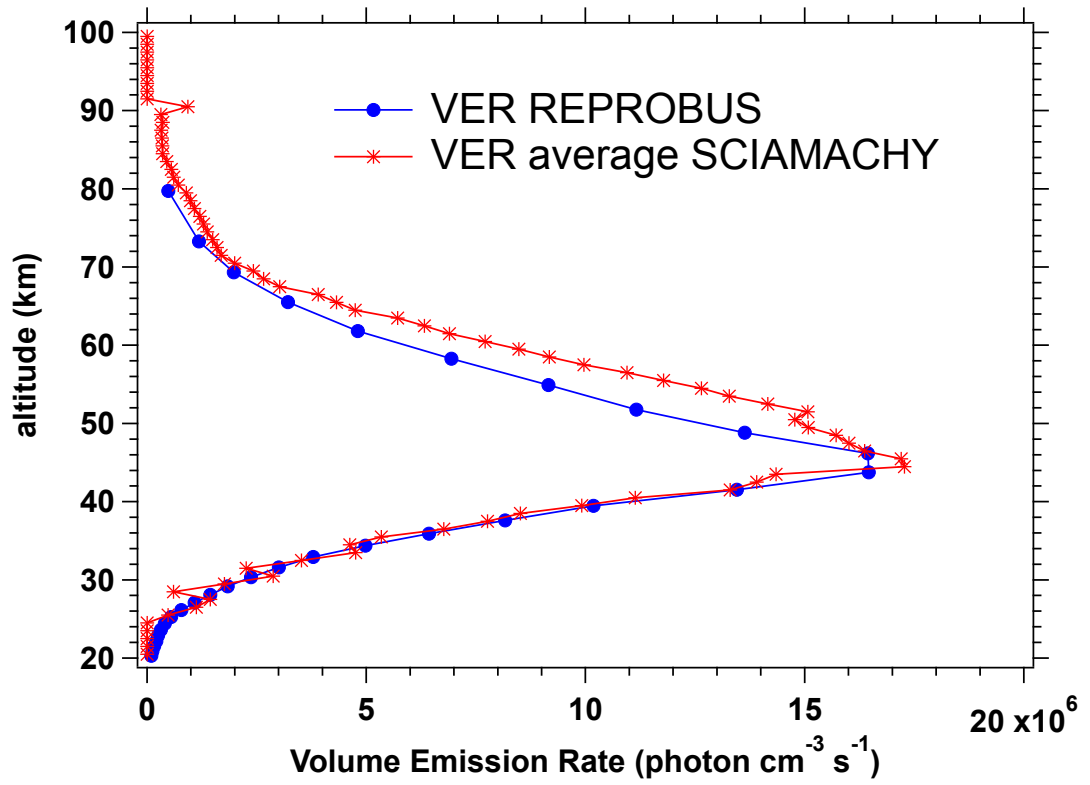
Figure D1: (In red) VER SCIAMACHY profile used to build the synthetic airglow spectrum put in the simulated spectrum to be inverted. (In blue) associated (co-located) REPROBUS VER profile, showing the underestimation of REPROBUS airglow modelling above 50 km. The airglow synthetic spectra associated to these two VER profiles are illustrated on Fig. D2. They are very similar.
