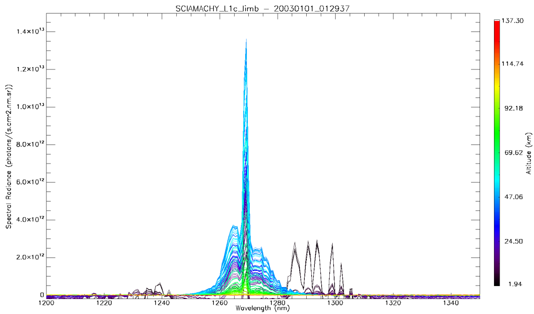
Figure F4. Airglow spectra obtained from Figure F3 by subtracting a linear interpolation based on the two constant values of the continuum (one on each side) estimated from the median value of all points outside the O_2^* band. This correction is valid above \sim 20 km of tangent altitude.
