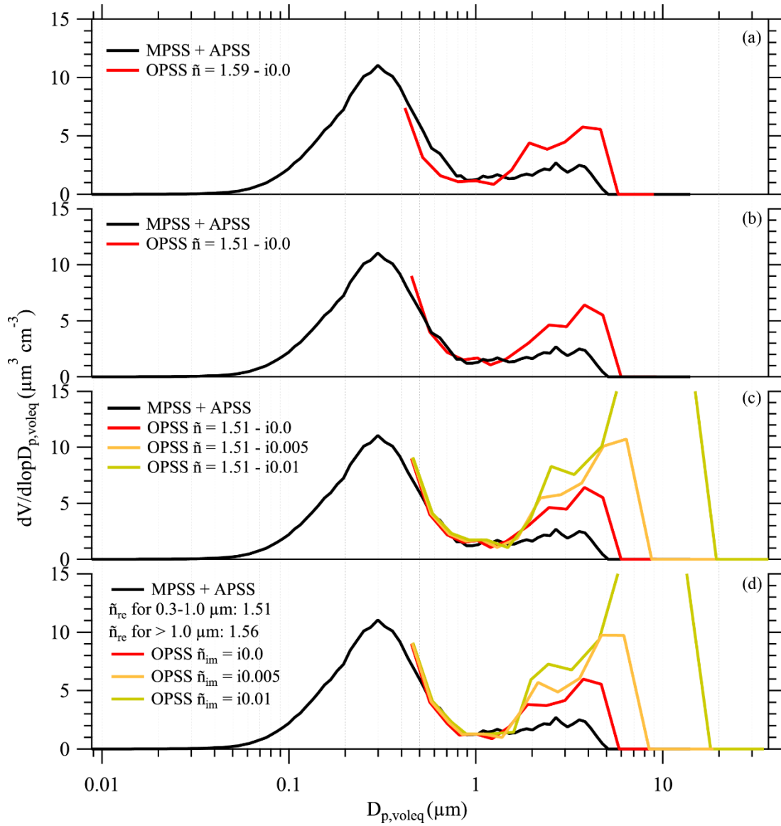
Figure 8. Demonstration of the complex refractive index correction done on the OPSS size distribution. In (a), the x-axis for the OPSS is optical diameter ( D_{p,opt} ). In the succeeding panels (b-d), the OPSS PVSD has been corrected and the x-axes are geometric mean volume equivalent diameters ( D_{p,vol}eq ).
