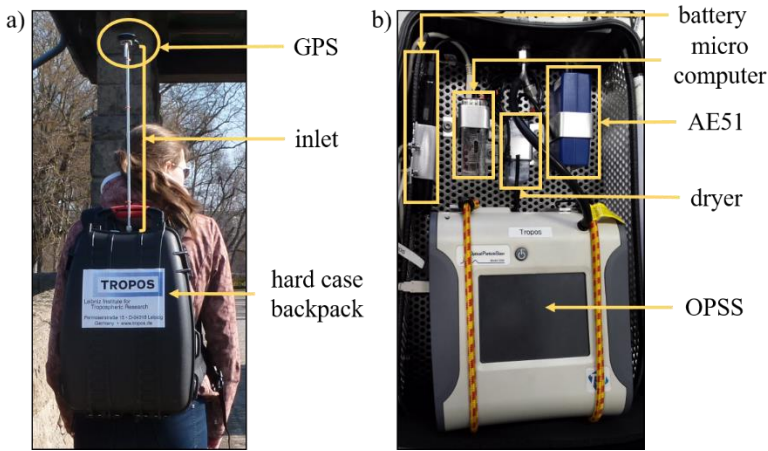
5 Figure A 1 The TROPOS aerosol backpack from outside (a) showing the GPS unit, inlet, and entire backpack; and from inside (b) showing the different components and main instruments: AE51 and OPSS. Image source: TROPOS, 2016
